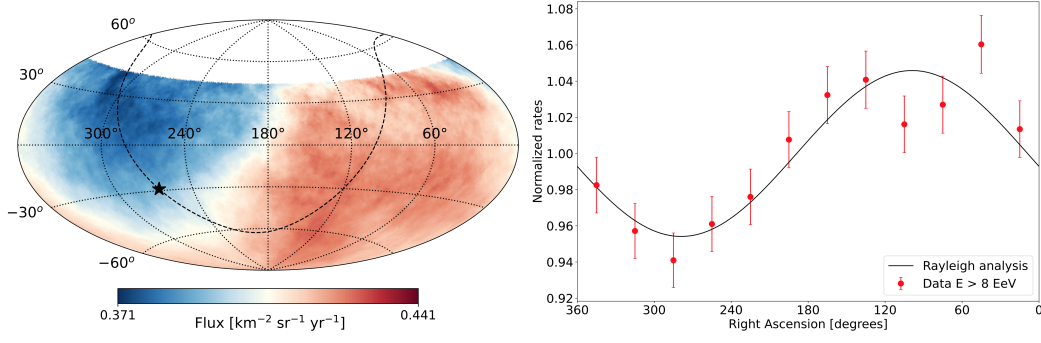
Figure 1: Left: Flux of UHECRs above 8 EeV measured at the Pierre Auger Observatory in equatorial coordinates. The solid line represents the Galactic plane and the black star shows the position of the Galactic center. From [2].
