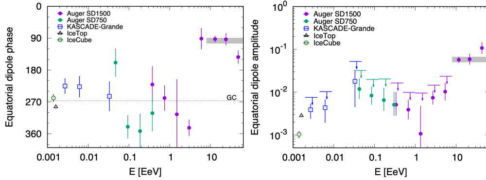
Figure 2: Energy-evolution of the dipole phase ( left ) and dipole amplitude ( right ) measured at the Pierre Auger Observatory given by filled circles. For the amplitude, the 99% confidence upper limits are given in bins with p -values larger than 1%. Results from different experiments are denoted by other markers. From [2].
