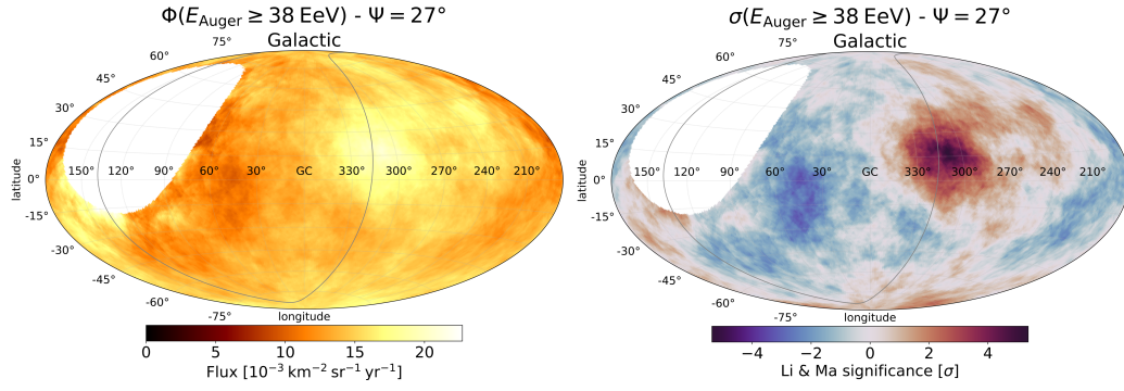
Figure 3: Flux- ( left ) and significance ( right ) maps for the best-fit values, energy threshold and search radius, of the overdensity search in Galactic coordinates. The grey line shows the supergalactic plane. From [2].
