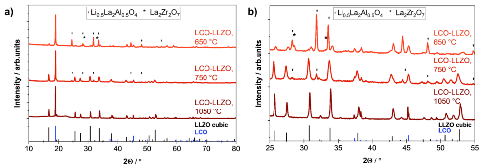
Figure 4.2.5: XRD pattern of tapes after heat treatment of 650 °C, 750 °C and 1050 °C with indication of side phases and the cubic LLZO structure (ICSD: 182312) 52 and LCO (ICSD: 29225) as references, adapted from 218 is licensed under CC BY 4.0 ( https://creativecommons.org/licenses/by/4.0/ ).
