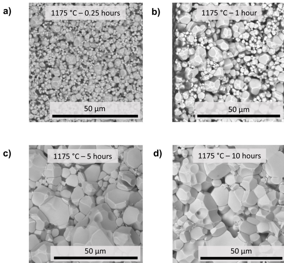
Figure 4.1.14: BSE-SEM image of a cross-section (fractured, not polished) of a sintered LLZO tape without additional Li source but sintered in a Li saturated crucible is shown to evaluate the grain growth, grain shape and grain size. Here, sintering parameters were as following: a) for 0.25 hours, b) for 1 hour, c) for 5 hours and d) for 10 hours, all at 1175 °C with LLZO-10 powder.
