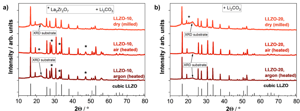
Figure 4.1.2: XRD patterns of the wet-ball milled LLZO powder (dry) and after an additional heat treatment of 750 °C for 2 hours in air and in argon are shown. For analysis, the cubic LLZO reference (ICSD: 182312) 52 is given, while a) shows the LLZO-10 powder for each treatment, and b) shows the LLZO-20 powder for each treatment.
