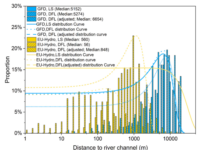
Fig. 13. Distribution of distance to river channels from either EU-hydro or a combination of GFDs for DFLs and landslides (LS). (GFD: combined global fluvial datasets, including GRWL (Allen and Pavelsky, 2018), MERIT Hydro (Yamazaki et al., 2019), and GLOW (Feng et al., 2022)).
