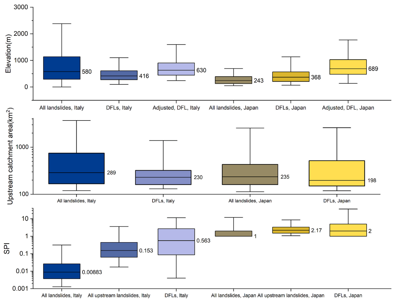
Fig. 6. Box plot showing the geomorphological parameter distribution of all landslides and DFLs in Italy and Japan.
