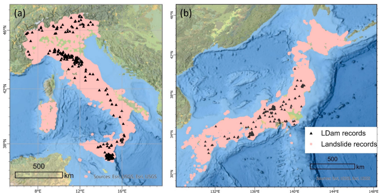
Fig. 3. LDam and landslide records that were used for the spatial distribution comparison: a) Italy; b) Japan.
