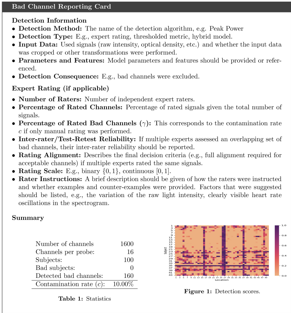
Fig. 9 Bad channel reporting card. The figure displays the template for the bad channel reporting card that contains basic information about the detection method, statistics, and detection scores across channels and subjects.
