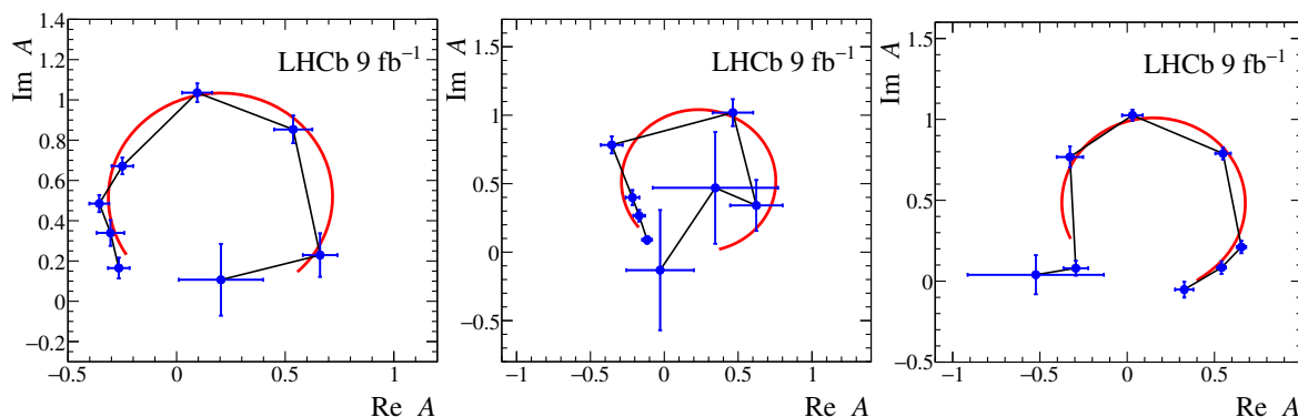
Figure 3. Argand diagram for the quasi-model-independent partial-wave analysis for the (left) T_{cc0}^*(4475)^0 , (middle) T_{ccs1}(4600)^0 , and (right) T_{cc1}(4200)^\pm resonances. The fitted lineshape knots are displayed as connected points with error bars and the invariant mass increases counterclockwise. The Breit-Wigner lineshape with the mass and width from the nominal fit is superimposed (red line).
