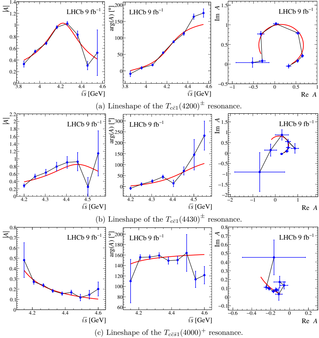
Figure 14. (Left) Magnitude, (middle) phase and (right) Argand diagram of the quasi-model-independent lineshape for T_{c\bar{c}}^{\pm} \rightarrow \psi(2S)\pi^{\pm} and T_{c\bar{c}S}^{+} \rightarrow \psi(2S)K^{+} states. The fitted knots are displayed as connected points with error bars. The Breit-Wigner lineshape with the mass and width from the nominal fit is superimposed (red line).
