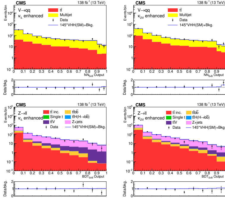
Figure 10. Postfit BDT distributions with the signal-plus-background hypotheses of the FH and 2L channels.
