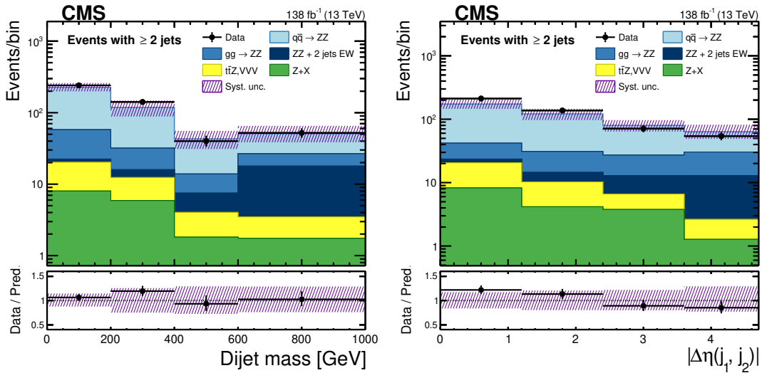
Figure 4: The dijet mass (left) and |\Delta\eta| (right) between the two highest- p_T jets in events with at least two jets. Events are required to have 60 < m_{Z_1 Z_2} < 120 GeV. Other details are as in the caption of Fig. 2.
