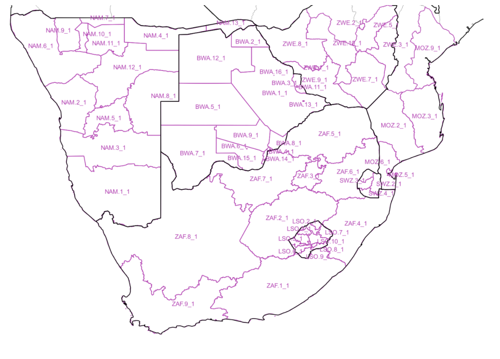
Figure C.1 Location of the 65 fully covered provinces by the ICON-LAM domain over southern Africa. Provincial boundaries are coloured purple and country boundaries are coloured black. For country names and the reference of the indexed province name to the full name, readers are forwarded to Table C.1.
