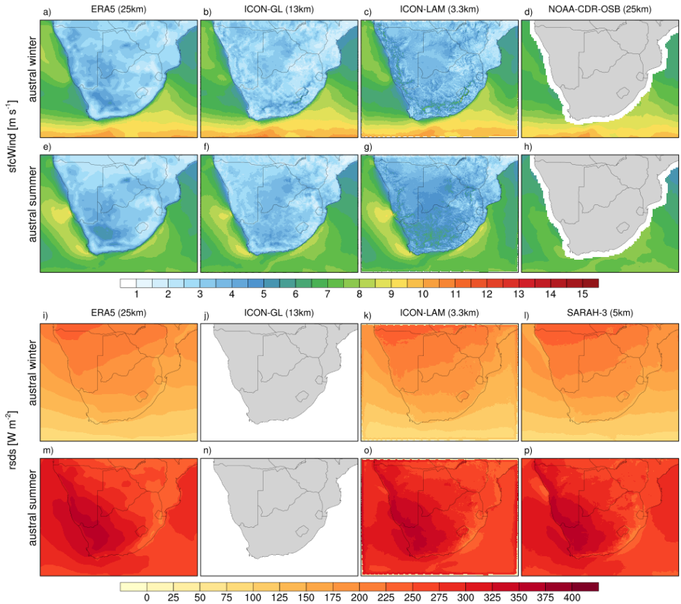
Figure 3.3 Average sfcWind [ \text{m s}^{-1} ] (top multi-panel) and rlds [ \text{W m}^{-2} ] (lower multi-panel) for
