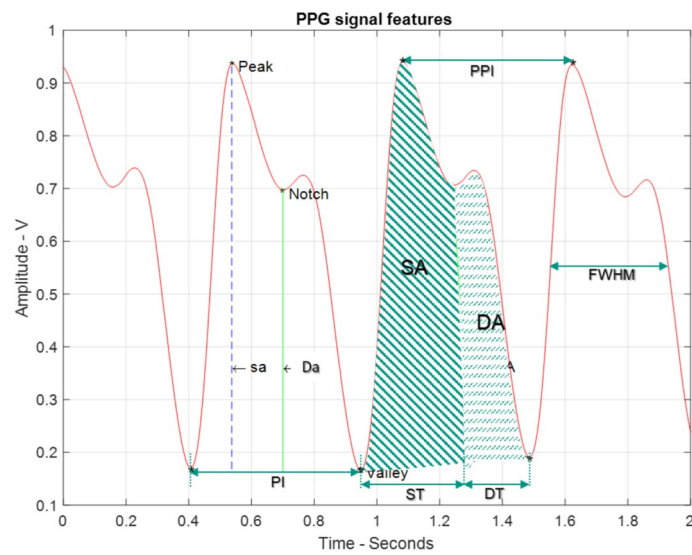
Fig. 20 The definitions of the PPG signal features
