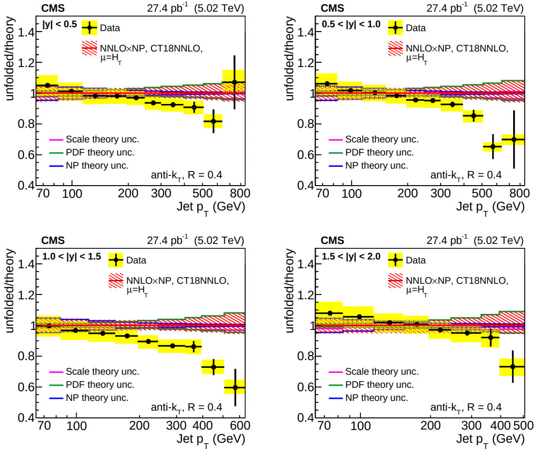
Figure 10: Ratios (points) of the unfolded measured cross sections to the NNLO theoretical predictions, using the CT18NNLO PDF set, with \mu = H_T . The vertical error bars show the statistical experimental uncertainty, the yellow band shows the systematic experimental uncertainty, the hashed red band shows the total theoretical uncertainty, and the individual sources of theoretical uncertainty are shown with colored lines.
