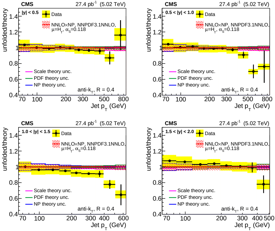
Figure 11: Ratios (points) of the unfolded measured cross sections to the NNLO theoretical predictions, using the NNPDF3.1NNLO PDF set, with \alpha_s(m_Z) = 0.118 and \mu = H_T . The vertical error bars show the statistical experimental uncertainty, the yellow band shows the systematic experimental uncertainty, the hashed red band shows the total theoretical uncertainty, and the individual sources of theoretical uncertainty are shown with colored lines.
