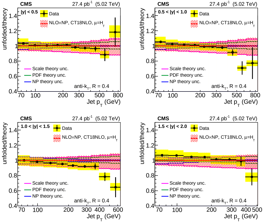
Figure 9: Ratios (points) of the unfolded measured cross sections to the NLO theoretical predictions, using the CT18NLO PDF set, with \mu = H_T . The vertical error bars show the statistical experimental uncertainty, the yellow band shows the systematic experimental uncertainty, the hashed red band shows the total theoretical uncertainty, and the individual sources of theoretical uncertainty are shown with colored lines.
