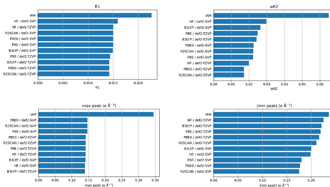
FIG. 6. Quality indicators of the IAM and HAR models created by SISYPHOS employing ORCA and NoSpherA2 on the Olex2 internal “SuperSugar” dataset.
