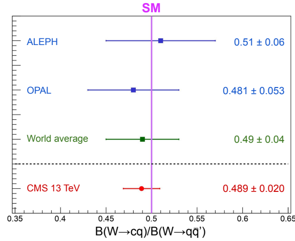
Figure 2: Comparison of the measured value of R_c^W with previous LEP2 measurements [4, 5], and the world-average value [3]. Horizontal bars represent the total uncertainty of the measurements.
