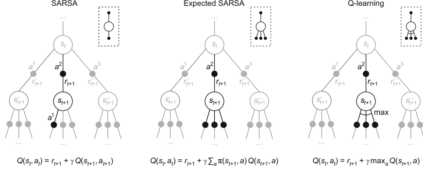
Figure 6.5: Backup diagrams for SARSA, Expected SARSA, and Q-learning. An example with three available actions per state is shown for each backup diagram (inset; reproduced from [70]) of each method. States are indicated by an open circle and state-action pairs by a solid circle. The experience tuple under evaluation is e_t = (s_t, a^2, r_{t+1}, s_{t+1}, a^1) in all examples. The propagation of value information from Q(s_{t+1}, a_{t+1}) back to Q(s_t, a_t) is defined according to the formula below each method. Note that Expected SARSA and Q-learning ignore the second action. They take all state-action pairs of the successor state into account, and either weight them by the policy \pi (Expected SARSA) or select the state-action pair with the highest Q-value (Q-learning). In this study, Expected SARSA was used to update the Q-values.
