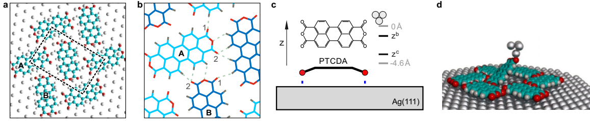
Figure 4.1: Structural properties and interactions of PTCDA/Ag(111). a , The nearly rectangular unit cell of PTCDA on Ag(111) ( 18.96 \times 12.61 \text{ \AA}^2 , tilted by 1^\circ ) contains two molecules with distinct adsorption sites. Molecule A is aligned with the underlying Ag(111) lattice, while molecule B is misaligned. b , The \text{O}_{\text{carb}} are either in the vicinity of one hydrogen (type 1) or two hydrogens (type 2). c , Structural formula and schematic side view of PTCDA bonding to Ag(111). The important heights during a manipulation are sketched on the right side. d , Rendered scene of a PTCDA molecule being partial lifted from the layer with a Ag-terminated tip.
