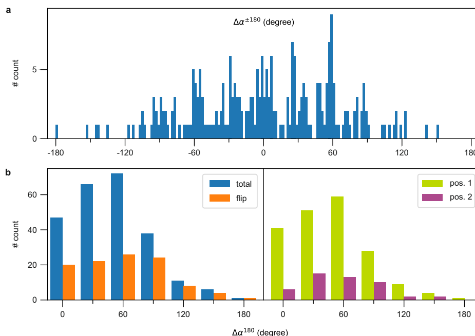
Figure 4.14: Distribution of delta angles before and after the manipulation of the complex. a , Histogram of all recorded \Delta\alpha^{\pm 180} . The bin width is 2^\circ . b , Histograms of the absolute values of the data in a . The left histogram compares the total number of lifting experiments to the number of experiments which show a chirality flip. The right histogram compares the experiments contacted diagonal opposite (pos. 1) with the ones contacted opposite (pos. 2) to the Ag adatom. The bin width is 30^\circ .
