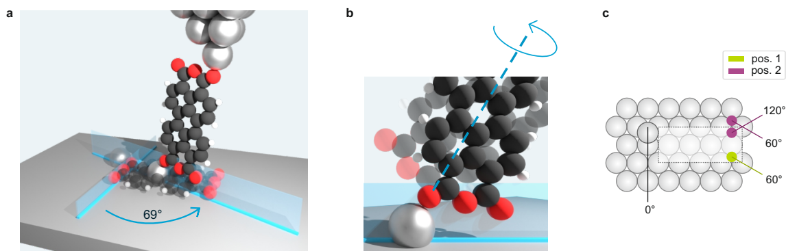
Figure 4.15: Model of the junction during vertical manipulation. a , Sketch of the anticlockwise rotation of PTCDA during lifting for a right-handed complex. The molecule is expected to rotate around 69^\circ , if the Ag adatom moves along the diagonal of PTCDA during lifting in the absence of surface corrugation. The blue walls indicate the orientation of the oxygen atoms before and during the VM. b , Sketch of the closest (opaque molecule) and furthest (transparent molecule) distance between the unpaired O_{\text{carb}} at the bottom of PTCDA and the surface. The dashed line indicates the rotation axis along the diagonal of PTCDA. The opaque molecule has the same orientation as in a . c , Sketch of predicted \Delta\alpha if the adatom ends up in the closest hollow site to the tip during VM. The expected adatom position and orientation of the short axis of the molecule are indicated in green (purple) for contact position 1 (2). Two adatom sites are indicated for contact position 2, because the distribution of \Delta\alpha shows a bias to \Delta\alpha < 90^\circ .
