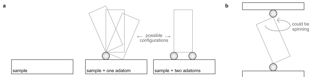
Figure 4.10: Schematics of artificial tips and junction structure a , Schematic of three artificial tips on the surface representing: flat tip, flat tip with a single atom protrusion, flat tip with two single atom protrusions. b , Schematic of a symmetric junction. The molecule could be spinning in it. More precisely, it could perform a random walk between fixed angles of rotation.
