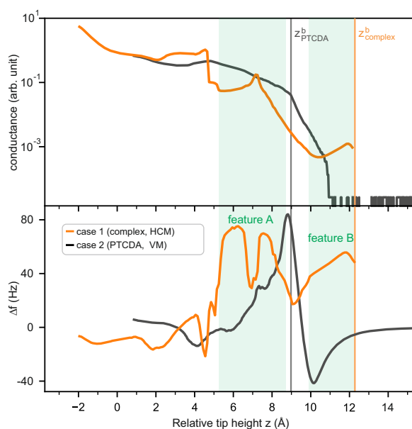
Figure 5.7: Median curves of recorded conductance and \Delta f signals for Ag+PTCDA (HCM) and PTCDA (VM). Two vertical lines (PTCDA: grey, complex: orange) indicate the height z^b , where the bond to either the tip or the surface breaks during the manipulation. The z area corresponding to feature A and B is highlighted in green. z = 0 Å corresponds to the height of (initial) contact formation. For more information see text.
