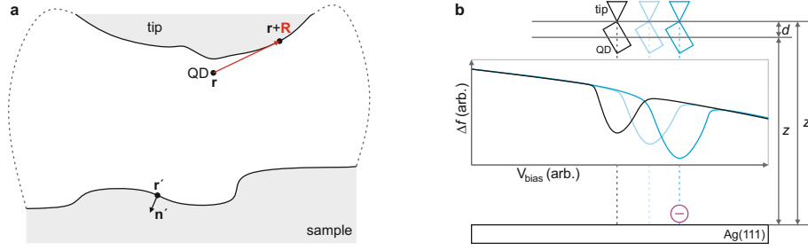
Figure 7.1: Spatial relationships and measurement principle of SQDM. a , Schematic of the spatial relationship between sample, QD, and tip. \mathbf{r}' are points on the sample surface. \mathbf{n}' is the surface normal at \mathbf{r}' . The QD is fixed to the tip and at position \mathbf{r} . The relative position between \mathbf{r} and \mathbf{r} + \mathbf{R} , points on the tip surface, are thus fixed during scanning and fully described by \mathbf{R} (red arrow). Dashed lines indicate electrical connection of tip and sample at infinity. b , Schematic of the measurement principle of SQDM at the example of \Phi^+ . An additional negative charge (purple) is placed on the sample surface. The closer the distance between QD and the charge on the surface, the more V_{\text{bias}} is needed to compensate for \Phi_s to maintain \Phi^+ . QD positions and corresponding \Delta f spectra are indicated by colour.
