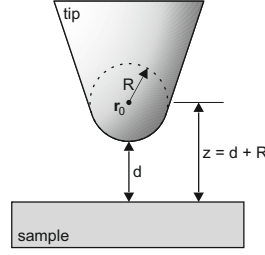
Figure 2.3: Schematic of the STM junction according to Tersoff and Hamann. The part of the tip closest to the surface is modelled as a spherical potential with its origin at \mathbf{r}_0 and a curvature of R . d is the smallest distance between the tip and the surface. Adapted from [24].
