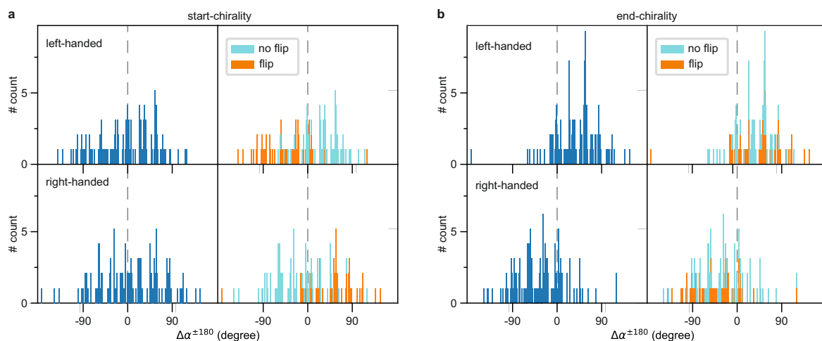
Figure 4.17: Histograms showing the rotation of the complex due to VM in dependants of the chirality. The chirality of the complex is assigned at two points in time: before (a) and after (b) the VM. On the left side of a and b the histograms show the total number of recorded \Delta\alpha^{\pm 180} . On the right, each bin from the left is subdivided into the number of experiments where the chirality of the complex remained the same before and after the VM (no flip, light blue) and where the chirality flipped (flip, orange). The bin width is 2^\circ
