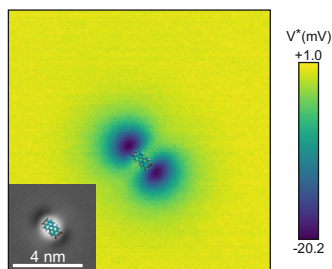
Figure 7.2: Measuring the electrical potential of an isolated PTCDA on Ag(111). The SQDM V^* (STC controller, z_{tip} = 24.4 \text{ \AA} ). The inset shows the STM topography of an isolated molecule (setpoint: 0.35 V, 0.2 nA). The orientation of the molecule is indicated in both the inset and the V^* image.
