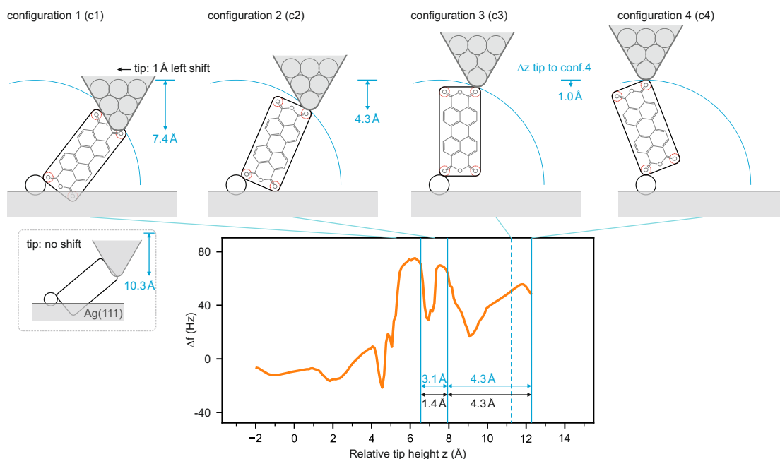
Figure 5.8: Simple model for the junction configuration during HCM considering only the geometry of Ag+PTCDA without distortions. Ag adatom, PTCDA and STM tip are drawn to scale. The blue quarter circle indicates the tip trajectory. The blue arrows ( c1 to c3 ) indicate the difference in tip height to c4 . c1 , Free "top" O_{\text{carb}} attaching to (or detaching from) tip. That the bottom corner is drawn below the surface is due to the simplicity of the model. This simply shows that the molecule must undergo a bending motion (and potentially a rotation out of the vertical plane) during the manipulation. c2 , Free "bottom" O_{\text{carb}} attaching to (or detaching from) surface. c3 , Straight configuration. c4 , Diagonal configuration with the molecule fully stretched in the junction. The configurations are assigned to the \Delta f signal as indicated by the blue vertical lines. The line for c3 is dashed, indicating the lack of a distinct \Delta f feature to assign to. The \Delta z values between the configurations in model (experiment) height are indicated in blue (black). For more information see text.
