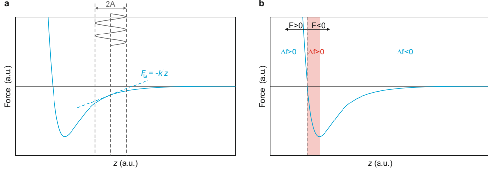
Figure 2.5: Lennard-Jones like force as an example for the tip-sample force. a , For small amplitudes, the tip-sample force is approximated to be proportional to k' in the range of the oscillation. Here, the slope is positive and thus k' < 0 . b , The signs of force and frequency shift are the same for most parts of the z range. In these parts, a positive frequency shift corresponds to a repulsive force and a negative one to an attractive force. Only in the area highlighted in red have they opposite signs.
