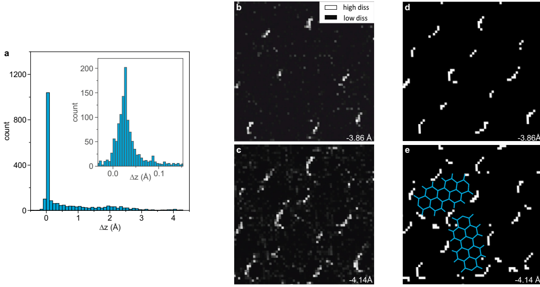
Figure 4.9: Measured vs predicted dissipation. The data shown is from the grid in Fig. 4.3. a , Histogram of \Delta z = z^c - z^b for all spectra which show contact formation. b , c , Height slices through the qPlus dissipation signal during tip approach. d , e , Corresponding simulated dissipation defined by the conditions for z^c and z^b described in the text.
