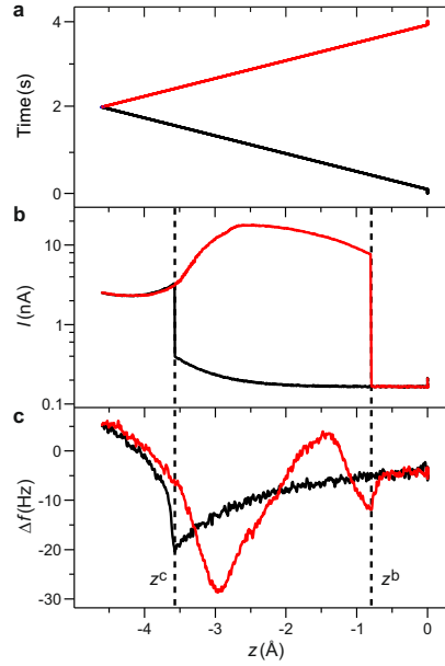
Figure 4.2: Manipulation parameters and data recorded of a VM of PTCDA/Ag(111) in the vicinity of B_2 . The approach is coloured in black and the retraction in red. a , Manipulation z ramp. First the tip approaches 4.6 \text{ \AA} towards the surface, then retracts back to the starting position ( V = -1 \text{ mV} ). Between manipulations, a voltage pulse is applied. b , I(z) spectrum and c , \Delta f(z) spectrum. The heights z^c and z^b are extracted from b .
