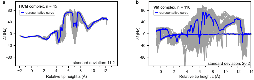
Figure 5.6: Frequency shift curves for HCM and VM of the complex. The representative curve is blue and all other curves are grey for the respective dataset. n corresponds to the number of trajectories in each dataset. a , HCM along a circular trajectory. b , VM. For more information see text.
