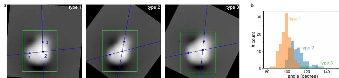
Figure 4.12: Adatom binding geometries for Ag+PTCDA on Ag(111). a , STM topography images of geometry types for right-handed complexes. The two blue lines are defined by the three blue dots: (1) centre of left LUMO lobe, (2) brightest spot on right lobe, (3) centre of adatom. b , Statistics of adatom binding angles as determined by the angle between the blue lines in a .
