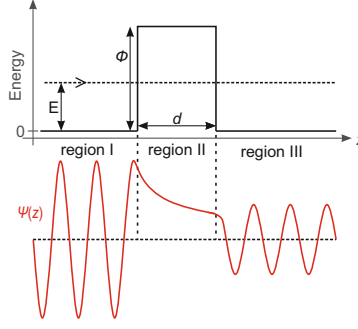
Figure 2.1: Tunnelling through a 1D barrier. The upper part shows a right travelling particle with energy E and the lower part shows its corresponding wave function. The wave function decreases exponentially with the effective barrier height \Phi_{\text{eff}} = \Phi - E in the classical forbidden region.
