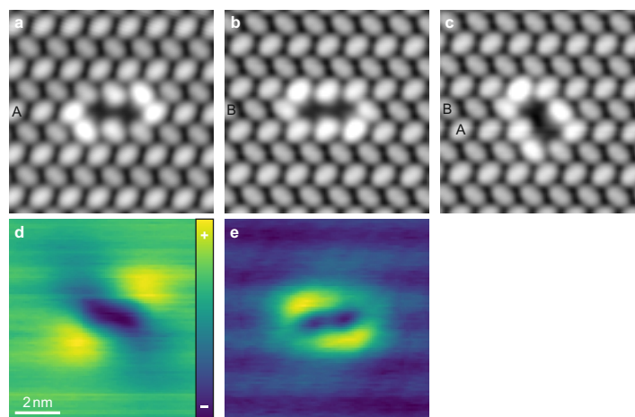
Figure 7.8: STM topography and electrical potential of double vacancies. STM topography of double vacancies: a , type AA vacancy, b , type BB vacancy, c , type AB vacancy. Molecule A and B are indicated. Corresponding SQDM V^* of double vacancies: d , type AA, e , type AB. The scale and V^* contrast are indicated in d . The contrast is maximized for each image separately. Note that the V^* of d and e are based on the same data as Fig. 7.4c,d without line-by-line background correction.
