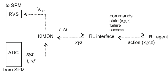
Figure 6.4: Sketch of the RL setup. Only the digital connections are shown.
