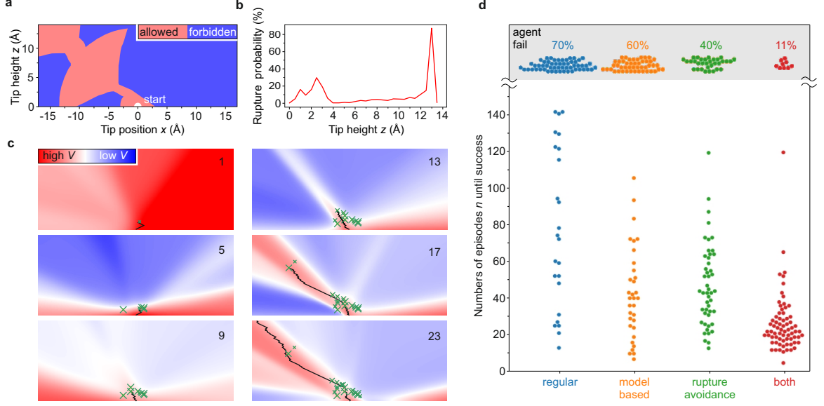
Figure 6.2: Training and performance of RL agents. a , Map (2D slice through 3D system; y = 0 ) of the synthetic bond rupture criteria of the simulated environment. b , Synthetic rupture probability as a function of z calculated in \Delta z = 0.5 \text{ \AA} intervals. c , Maps (2D slices; y = 0 ) of the Q-functions for different episodes of one successful lifting trial, showing the learning progress by the agent after the number of episodes indicated in the upper right corner. The executed trajectory by the agent (black curve; 2D projection) in each panel is based on the Q-function of the same panel. Green crosses indicate synthetic bond-ruptures triggered according to the criteria in a . d , Swarm plot showing the performance of different types of RL agents acting in the simulated environment in a . The number of episodes n needed to finish the removal task is plotted for 80 simulated experiments, or runs, for each agent. A run was considered a failure after 150 unsuccessful episodes (see text). The respective probability of agent-failure is indicated in the upper part of the plot.
