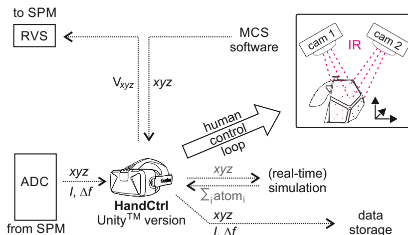
Figure 5.1: Schematic of HCM setup with HandCtrl (Unity™ version). Only the digital connections are shown. A Vicon™ motion capture system (MCS) and Oculus™ VR goggles are used for HCM.
