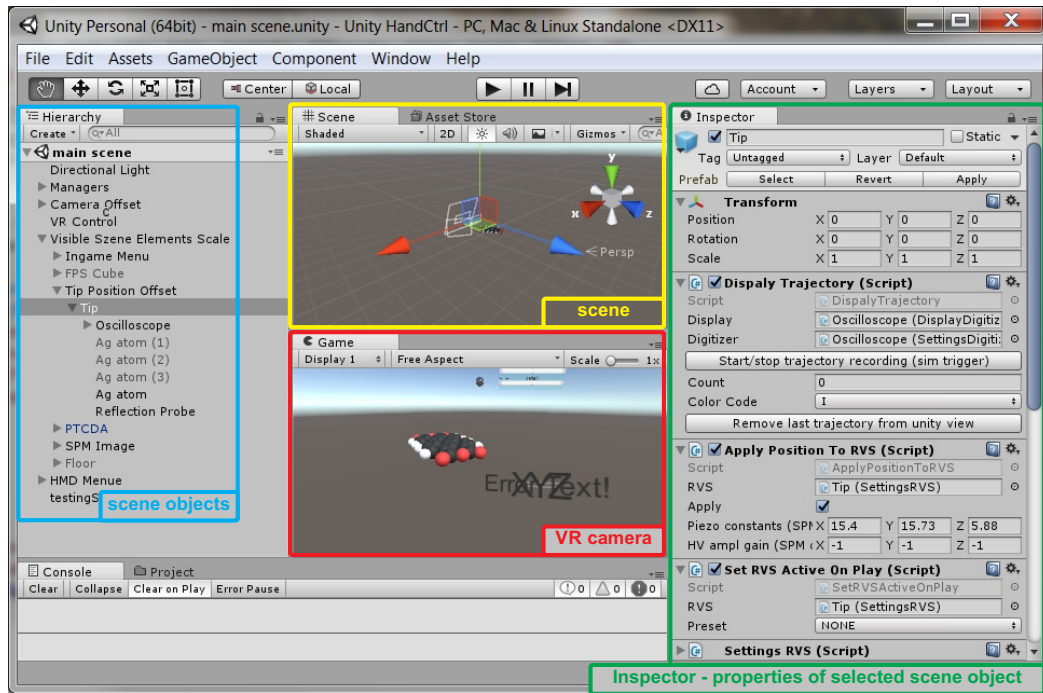
Figure 5.2: Screenshot of HandCtrl in Unity™ editor. The important windows for operating HandCtrl are highlighted by coloured rectangles: Hierarchy (blue), Scene (yellow), Game (red), Inspector (green).
