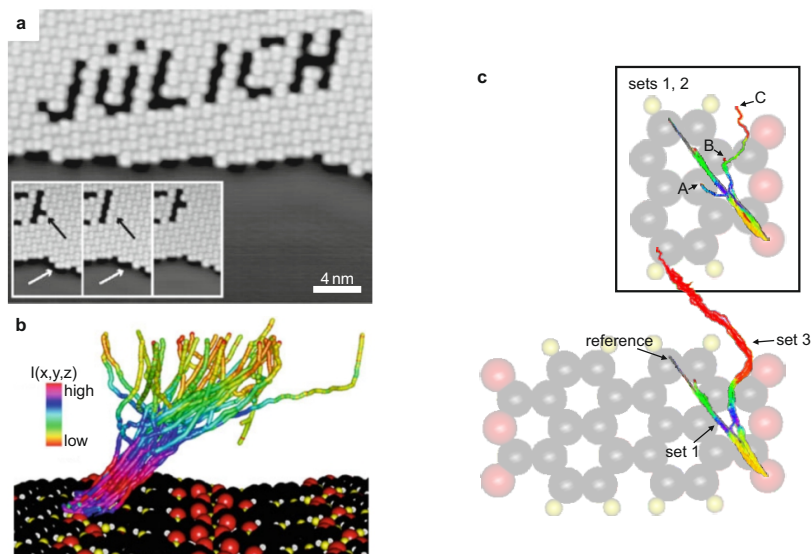
Figure 3.4: Results from hand-controlled manipulation for lifting individual molecules from a monolayer of PTCDA/Ag(111). a , STM topography image (setpoint: -0.35 V, 0.1 nA). The word "Jülich" was written by removing 48 PTCDA molecules with HCM. The insets show the successful correction of a writing error. b , The individual lifting trajectories of the molecules removed in a . c , Demonstration of the control during HCM, allowing highly reproducible I(x, y, z) and \Delta f(x, y, z) along the executed trajectories ( \Delta f not shown). The trajectories in set 1 follow the reference curve (the average trajectory from b ), which did not allow lifting of the molecule for the specific tip. A successful trajectory (set 3) was found after only three attempts (set 2: A, B, C), as shown in the inset.
