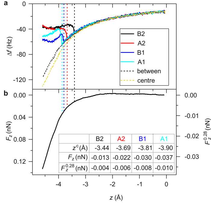
Figure 4.5: AFM spectra of approaching PTCDA/Ag(111) and extracted forces. a , \Delta f(z) spectra at different lateral positions for the approach. b , The background corrected local force acting on the tip. Local F_z(z) is calculated by subtracting the spectrum taken between the molecules from the spectrum taken in the centre of the molecule. F_z^{0.28}(z) gives the local force scaled with a factor of 0.28 and is used to extract the relative forces over the O_{\text{carb}} atoms. For further information see text.
