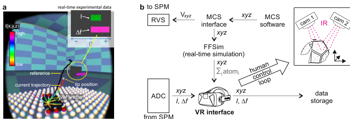
Figure 3.5: HCM software version written in C++. a , Screenshot of HCM (VR interface) during the task of removing a molecule from a PTCDA on Ag(111) layer. b , Schematic of digital data flow for the C++ version of VR interface (analogue connections are not shown).
