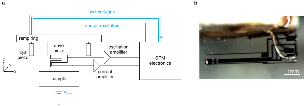
Figure 2.6: Schematic of the SPM setup and picture of a qPlus sensor. a , Schematic. The qPlus sensor is attached to a ramp ring. The ramp ring rests on three piezo tubes (two are shown). The piezos bend in the x , y direction and stretch in the z direction if the corresponding voltages are applied. A drive piezo allows the excitation of the qPlus sensor. b , Picture of a qPlus sensor with attached tip, available from Createc™.
