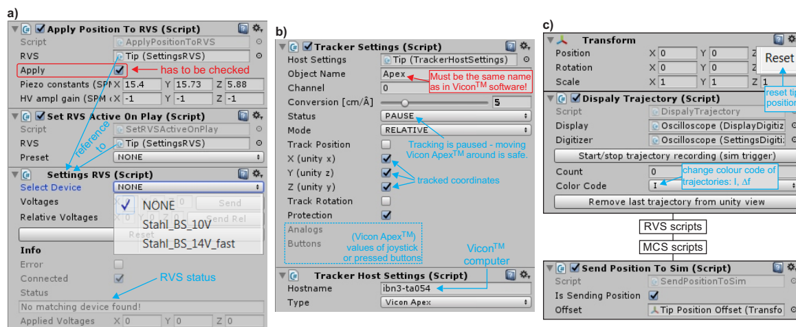
Figure A.6: Components of 'Tip' (Unity™ editor, Inspector). a, Scripts for remote voltage supply (RVS). In 'Settings RVS' the used RVS has to be specified. b, Scripts for motion capture system (MCS). c, Additional scripts attached to 'Tip' with their position in 'Inspector' indicated. They are useful during HCM operation.
