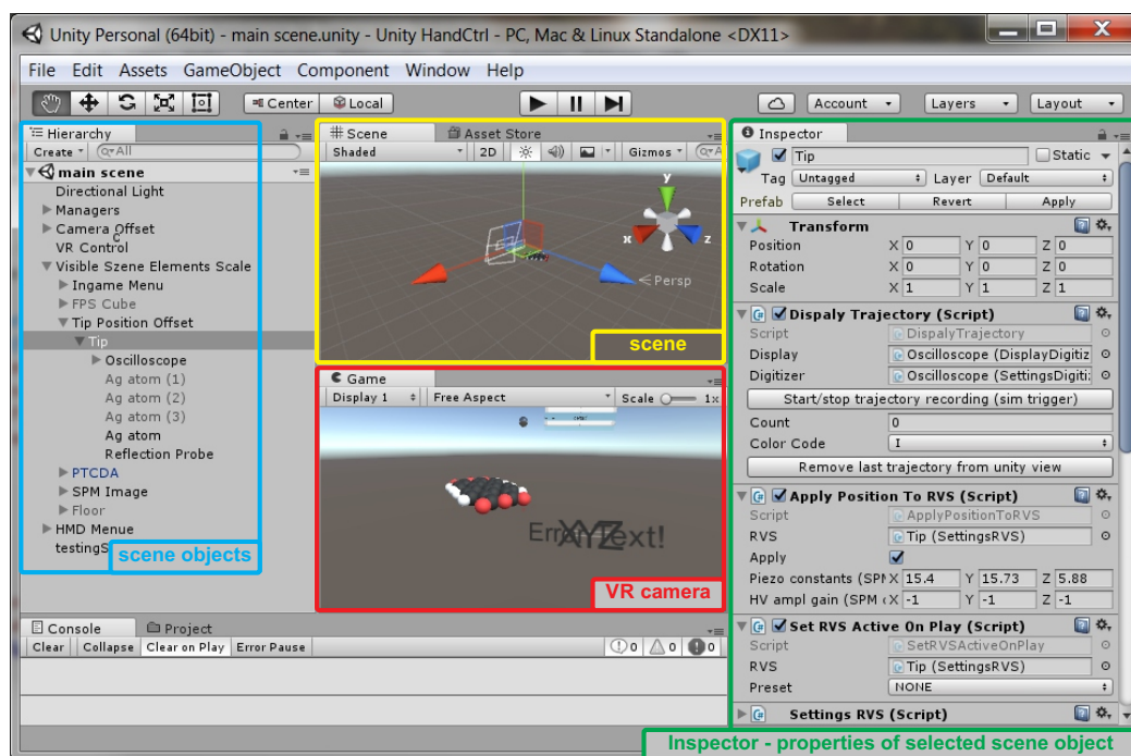
Figure A.3: Screenshot of HandCtrl in Unity™ editor. The important windows for operating HandCtrl are highlighted by coloured rectangles: Hierarchy (blue), Scene (yellow), Game (red), Inspector (green).
