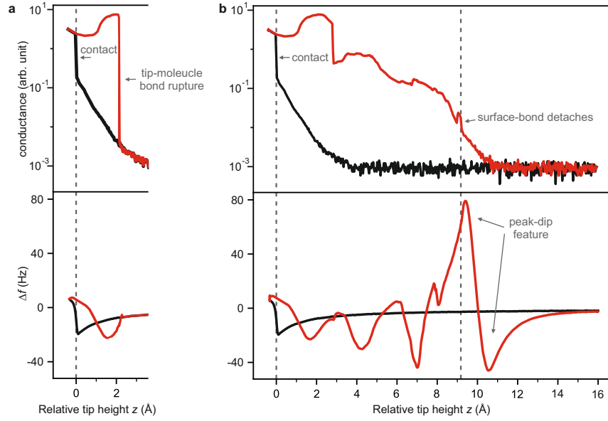
Figure 3.2: Vertical manipulation of PTCDA on Ag(111) - experimental signals. The tip approaches the surface (black curves) and retraces from the surface (red curves) on a vertical trajectory. The dashed lines indicate the height of contact formation and the height, where the last O_{\text{carb}} of PTCDA detaches from the surface. a , Manipulation signals for a molecule inside a molecular layer. b , Manipulation signals for an isolated molecule on Ag(111).
