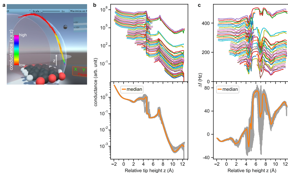
Figure 5.5: Recorded conductance and \Delta f signals during HCM of a Ag+PTCDA complex along a circular trajectory on Ag(111). a , Screenshot of experiment (Unity™ editor). The trajectories display the colour coded conductance( x, y, z ), from red (low values) to purple (high values). The z direction is indicated as a white arrow. b , Conductance signal corresponding to a . c , \Delta f signal corresponding to a . In b and c , the upper panel shows a waterfall plot. In b , the curves are offset by scaling them according to y_i = y_i \cdot 1.5^{i-1} . In c , consecutive curves are offset by 10 Hz. The lower panel in b and c shows the recorded curves (grey) and the corresponding median curve (orange). The tip height z = 0 \text{ \AA} corresponds to the bond formation between the tip and the Ag+PTCDA complex.
