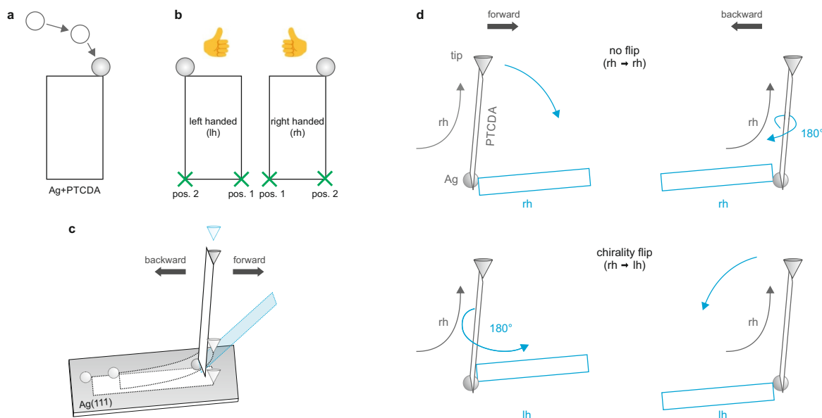
Figure 4.11: Structural properties of Ag+PTCDA on Ag(111) and illustration of the manipulation. a , Schematic of the construction of Ag+PTCDA via LM of a Ag adatom. b , Chirality and the two contact positions: diagonally opposite (pos. 1) and opposite (pos. 2) to the adatom. c , Definition of the molecule falling back to the surface in forward or backward direction. d , Schematic of the scenarios whether a chirality flip occurs. The blue parts indicate configurations after the tip-molecule contact rupture in c and d .
