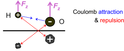
Figure 4.7: Schematic of the O-H coulomb interactions including image charges due to the metal substrate.
