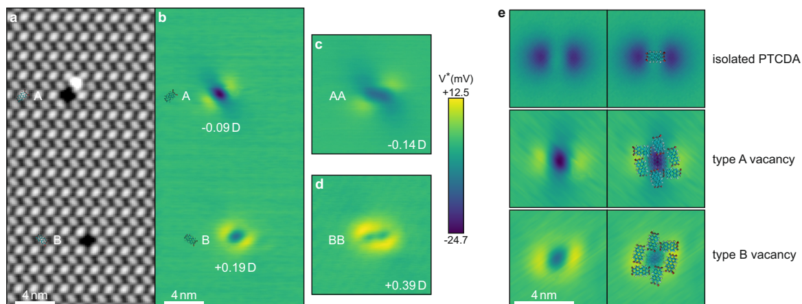
Figure 7.4: Measurement of the electrostatic potential over molecule vacancies in a PTCDA on Ag(111) monolayer and its comparison to the potential over an isolated PTCDA. The orientation of the molecules, the vacancy types and the corresponding measured dipole moments are indicated. a , STM topography of layer with type A and B vacancy (setpoint: 0.35 V, 0.2 nA). SQDM V^* images of molecule vacancies (STC controller): b , two single molecule vacancies of type A (top) and B (bottom, z_{tip} = 25.5 \text{ \AA} ), c , double vacancy of type AA ( z_{tip} = 27.8 \text{ \AA} ), d , double vacancy of type BB ( z_{tip} = 27.2 \text{ \AA} ). Line-by-line correction was applied to all V^* images to remove the background from the PTCDA layer. All V^* images share the same contrast range indicated on the right. Note that c , d look fainter than b because b was recorded closer to the surface. Note also the field emission damage visible in a . It occurred during the recording of V^+ of b and could be corrected by filling the affected area with an average value of the layer background signal. V^- was unaffected because it was recorded before V^+ . e , Comparison of V^* of isolated molecule (Fig. 7.2, ( z_{tip} = 24.4 \text{ \AA} )) with V^* of vacancies of type A, B. Each image is rotated such that the long axis of the centre (missing) PTCDA is orientated horizontally. On the right is the V^* image from the left superimposed with the molecular structure. The removed molecules are shown as transparent.
