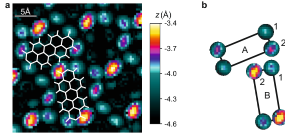
Figure 4.4: Contact heights extracted from approach spectra, of the grid in Fig. 4.3. a , z^c(x, y) map overlaid with the herringbone structure of PTCDA on Ag(111). Colour code: black for no contact, all other colours mark contact formation between tip and molecule at different heights. b , The four species of \text{O}_{\text{carb}} in the order they jump towards the tip, starting furthest away from the surface: \text{B}_2 , \text{A}_2 , \text{B}_1 , \text{A}_1 .
