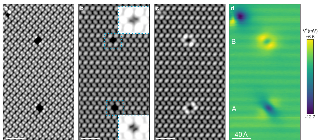
Figure 7.7: STM topography and electrical potential of type A and B vacancies for the same area. The topography images ( I = 0.2 nA) were recorded after d and at: a , -0.35 V, b , 0.35 V, c , 0.7 V. The insets in b show a magnification of the indicated areas with enhanced contrast in the vacancy. d , V^* measured at z^{tip} = 27.9 Å with STC controller. Also a damaged molecule from field emission (top left) and the contrast between rows is visible. Rows of molecule A and B and the image scale are indicated. The surface area recorded in d is slightly shifted to the left compared to a-c .
