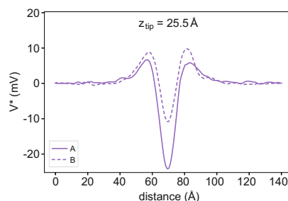
Figure 7.6: Direct comparison of profiles for type A and B vacancies along direction 1.
