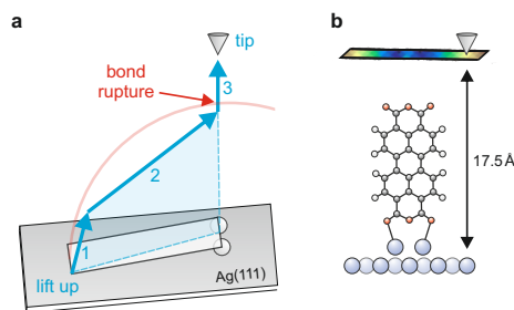
Figure 3.3: Manipulation protocol for erecting a 2Ag+PTCDA complex and its final structure. a , Schematic of the manipulation protocol. The three blue arrows indicate the manipulation trajectory for erecting PTCDA on two adsorbed Ag adatoms. The trajectory begins above one of the two unpaired O_{\text{carb}} (point of bond formation) and ends above the centre between the two Ag adatoms (after bond rupture). b , Schematic side view of a standing PTCDA molecule. The bar shows a recorded \Delta f -image at 17.5 Å above the Ag(111) surface, colour code from blue (negative) to brown (positive); adapted from [36]. For more information see text.
