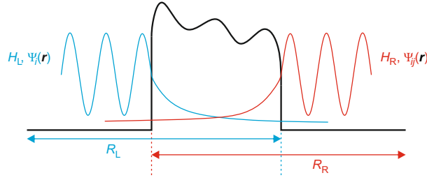
Figure 2.2: Separation of the tunnelling junction into the left R_L and right part R_R , according to Bardeen.
