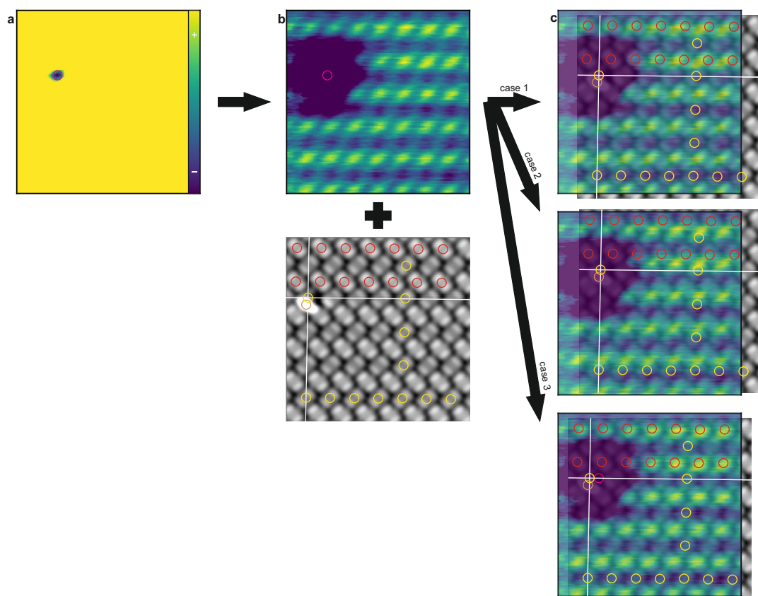
Figure C.1: Aligning STM topography and SQDM V^* on damaged molecule. The order of alignment steps is indicated by arrows. a , SQDM V^* (STC controller). The minimum is marked by a purple circle. b , SQDM V^* (same contrast range as in Fig. 7.3c) and corresponding STM topography (setpoint: -0.35 V, 0.2 nA). The coloured circle in the topography mark: molecule A (red), molecule B (yellow), maximum of damaged molecule (brown). c , Overlay of the images in b showing three possible cases for the alignment. Case 1, minimum V^* over the centre of damaged molecule. Case 2, minimum V^* over maximum of damaged molecule in the topography. Case 3, minimum V^* over dark area of damaged molecule.
