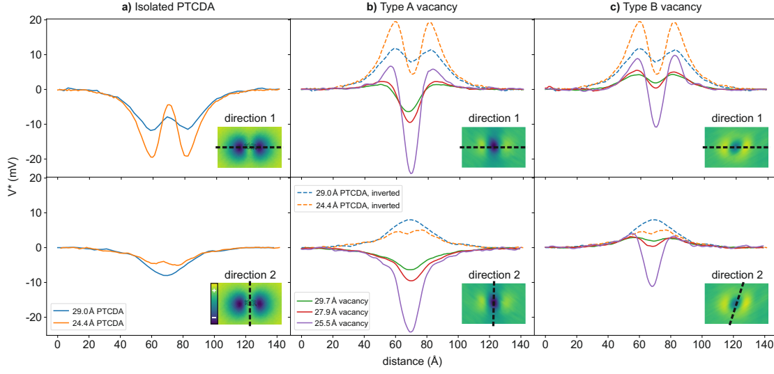
Figure 7.5: V^* line profiles of PTCDA/Ag(111) measured at different SPM tip heights. Profiles from left to right for: a , isolated PTCDA, b , type A vacancy, c , type B vacancy. The V^* profiles for type A and B vacancies at one height were extracted from the same SQDM image. The inverted PTCDA profiles (dashed lines) are plotted together with the vacancy profiles for direct comparison. The profile direction is indicated by the inset (taken from Figs. 7.2 and 7.4b).
