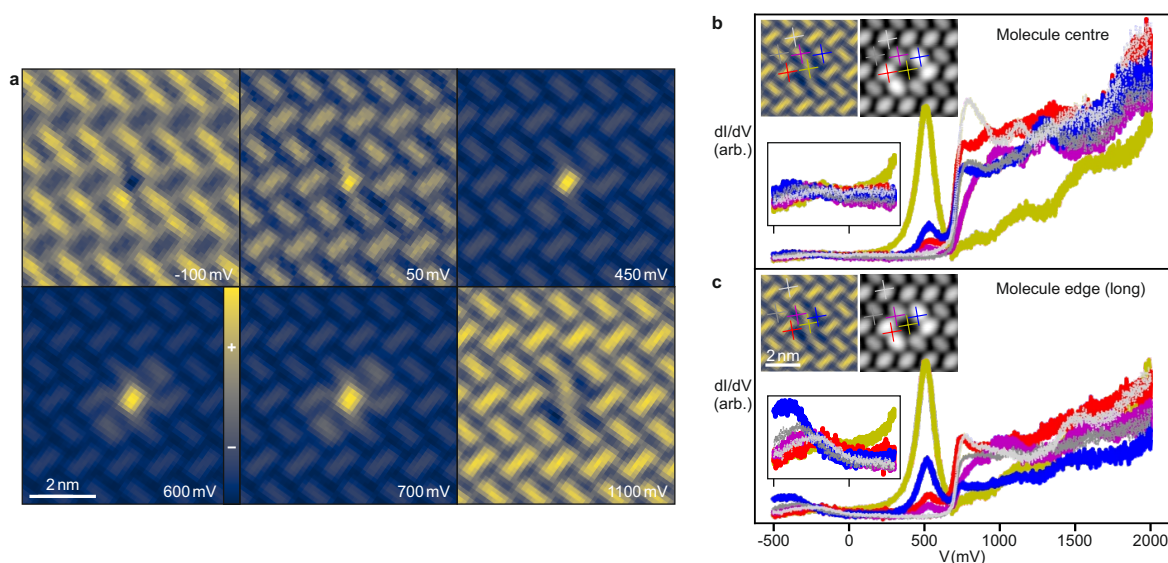
Figure 7.9: Slices and individual spectra of 85x85 spectra recorded in a grid around a type A vacancy. a , Slices through the I signal of the grid (left to right, first top then down): -100 mV, 50 mV, 450 mV, 600 mV, 700 mV, 1100 mV. Note that feedback is on between spectra, setpoint: -0.35 V, 0.1 nA. The tip is therefore closer towards the surface over the vacancy than over the layer. The scale and contrast are indicated. The contrast was optimized separately for each slice. b,c , dI/dV spectra of the indicated positions in the insets. The upper two insets (left to right): section of the 1100 mV slice ( a ), STM topography (setpoint: 0.7 V, 0.2 nA; section of Fig. 7.7c). The lower inset shows a magnification of the spectra in the range of -500 mV to 300 mV.
