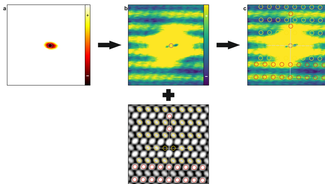
Figure C.2: Aligning STM topography and SQDM V^* on double vacancy of type BB. The order of alignment steps is indicated by arrows. a , Dielectric topography. The minimum is marked by a purple circle. b , SQDM V^* (STC controller, z_{tip} = 27.2 \text{ \AA} ) and corresponding STM topography (setpoint: 0.35 V, 0.2 nA). In the STM topography molecule positions are marked by coloured circles: red (A), yellow (B). c , Overlay of SQDM V^* and molecule positions of b . For more information see text.
