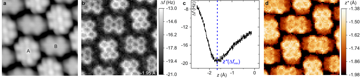
Figure 4.6: Height variation of PTCDA/Ag(111) measured with a CO-terminated tip. The perylene backbone of molecule A is (0.05 \pm 0.01) Å further away from the surface than for molecule B. a , STM topography image with a CO-terminated tip ( 3 \times 3 \text{ nm}^2 , I = 0.05 \text{ nA} , V = 16 \text{ mV} ). b , Height slice through \Delta f(z) spectra of a 3D dataset showing the perylene backbone of the PTCDA molecules. c , Example \Delta f(z) approach spectrum labelled with the position of z^*(\Delta f_{min}) . d , Map of z^*(\Delta f_{min}) for the tip approaching the surface, revealing the adsorption geometry of PTCDA on Ag(111). Bright colours correspond to distances further away from the surface than dark colours.
