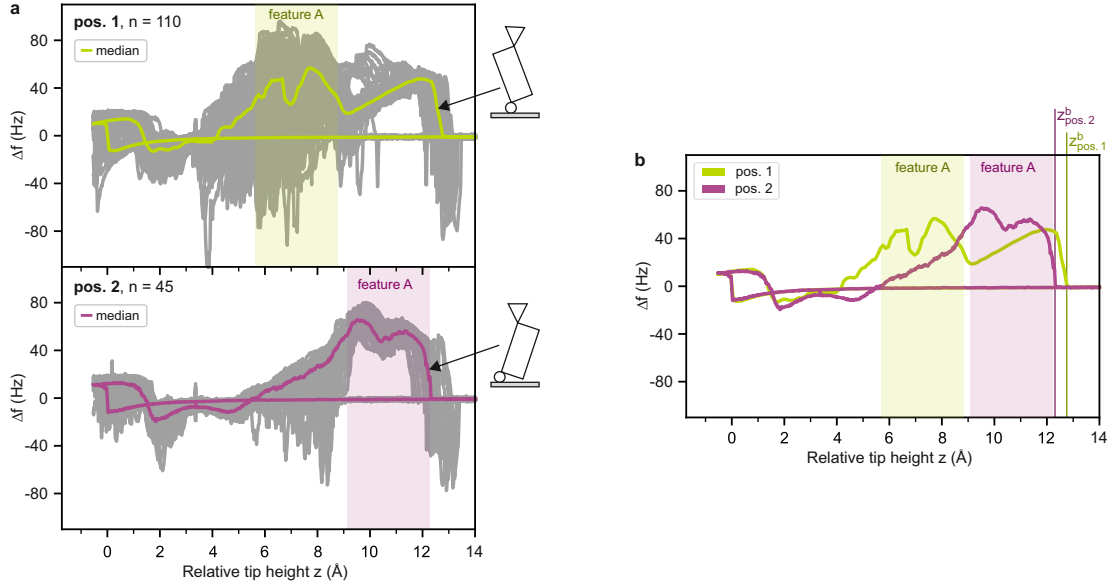
Figure 4.16: Comparison of VM of complex for contact position 1 and 2. a , \Delta f signals for both contact positions. The VM curves are coloured in grey and the corresponding median curves are coloured in green (position 1, diagonal opposite) and purple (position 2, opposite). The double peak feature (feature A) is indicated in the colour of the corresponding median curve. The sketches to the right of a indicate the expected junction configuration before tip-molecule contact breaking for both contact positions. The median curves were calculated by taking the median of all recorded \Delta f values at each z position of the corresponding VM curves. The number of VM curves used in calculating the corresponding median curves is indicated by n . z = 0 \text{ \AA} corresponds to the contact formation of the median curves. Any VM curves with loss of \Delta f tracking were removed. Only around half of the VM curves for position 1 are shown, because the first half was recorded with different manipulation settings to position 2, e.g. faster manipulation speed. b , Median curves from a . The tip-molecule contact breaking heights z_{\text{pos.1}}^b and z_{\text{pos.2}}^b for both contact positions are indicated by a vertical line. For more information see text.
