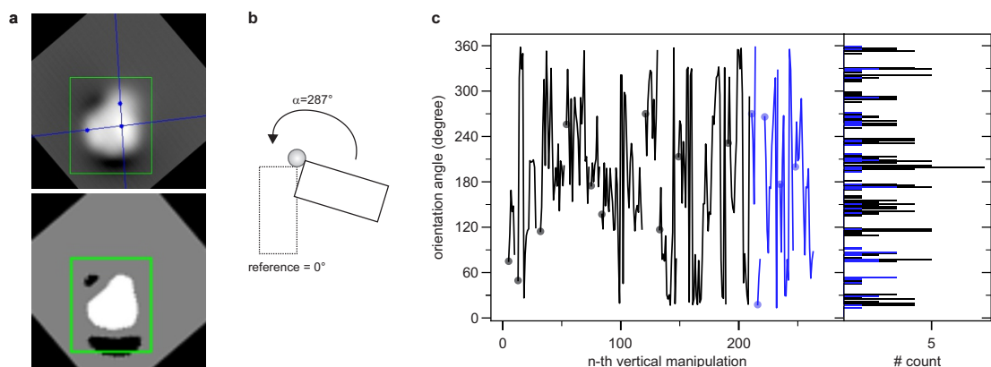
Figure 4.13: Detection and evaluation of the complex orientation. a , STM topography image of the Ag+PTCDA complex (top) and the processed version of the image (bottom) for the automated detection of the complex orientation. b , The angle \alpha is defined by the number of degrees a recorded orientation has to be rotated in anticlockwise direction to match the reference orientation. c , Graph (left) and histogram (right) of the recorded orientations of all VM experiments. The orientations in sequence are connected by a line in the graph. The start of each sequence is marked by a dot. The colour indicates the contact position used for VM: black (position 1), blue (position 2). The centres of the twelve orientation groups in the histogram are marked by green ticks.
