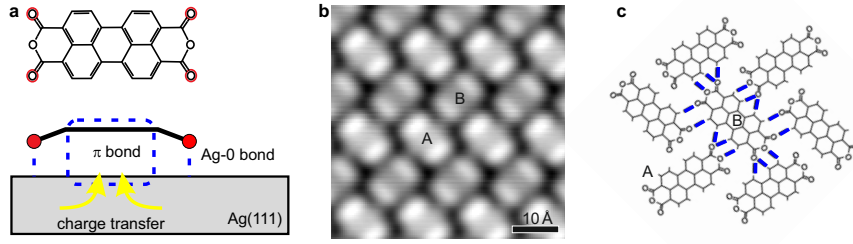
Figure 3.1: Interactions and structural properties of PTCDA/Ag(111). a , Structural formula and sketch of PTCDA bonding to Ag(111); adapted from [29]. b , Former LUMO contrast topography image of PTCDA/Ag(111), setpoint: -0.35 V, 0.2 nA. c , Sketch of the H-bonds between PTCDA molecules. The orientation of the molecules in b and c is the same.
