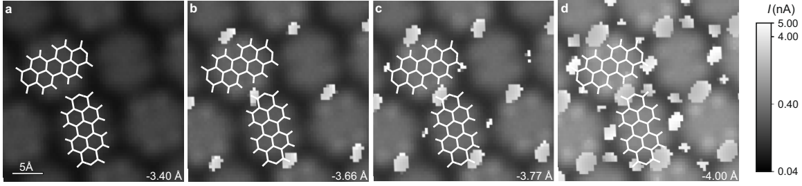
Figure 4.3: Height slices through I(x, y, z) data of 3D dataset for the tip approaching PTCDA on Ag(111), measured with qPlus oscillation and V_{\text{bias}} = -1 mV. The height given in each slice corresponds to the distance the tip approached towards the surface from the set point. Areas of high current indicate the presence of a tip-molecule bond. b-d , Bond formation around positions of \text{O}_{\text{carb}} . d , Additional observation of contact over the perylene core of molecule A.
