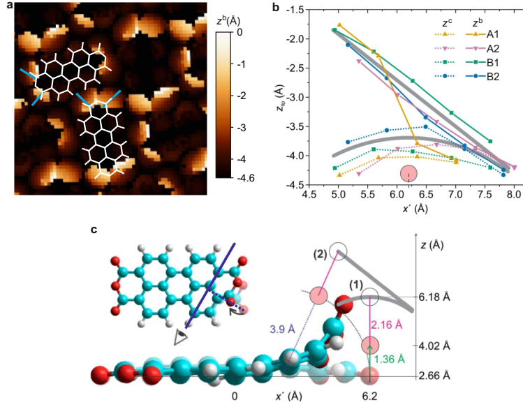
Figure 4.8: Analysis of tip-molecule bond breaking. a , z^b(x, y) map at which the tip-molecule bond breaks. The gradient of z^b(x, y) is indicated by the light blue lines. The origin of the asymmetry between oxygen atoms of the same type of the same PTCDA molecule lies most likely in a slightly asymmetric tip apex. b , z^c (dotted) and z^b (solid) line profiles along the white light blue lines in a . The O_{\text{carb}} position is indicated by a pink circle. The origin of the x axis is the centre of the respective molecule. The generic behaviour of the z^c(x') and z^b(x') curves is captured by the grey lines. c Analysis of the lifting process during the experiment based on the generic curves in b . The absolute z values are determined from theory [16] (see text). On tip approach to position (1), the O_{\text{carb}} jumps up 1.36 Å (green arrow) and forms a tip-molecule bond with a bond length of 2.16 Å (pink line). The bending radius obtained from an analysis of the z^b(x') curve is approximately 3.9 Å. A model molecule computed with a force-field approach [12] illustrates the lifting process. The bending axis, which is perpendicular to the drawing plane of the model, is shown as a blue line in the inset (top view of molecule).
