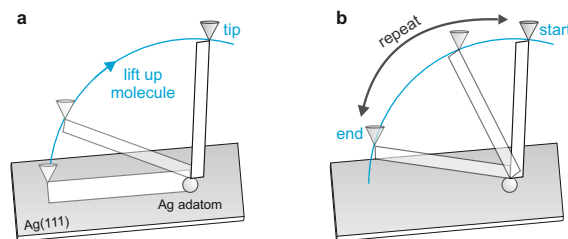
Figure 5.4: Schematic of Ag+PTCDA manipulation procedure. a , Contacting and lifting of Ag+PTCDA complex in stretched configuration. b , Repeated manipulation of complex on circle like trajectory. The start point is the last configuration in a , while the end point is close to the Ag(111) surface.
