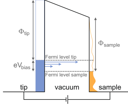
Figure 2.4: Energy diagram of the tunnelling process with a positive bias voltage V_{\text{bias}} applied to the sample. Electrons tunnel from occupied states of the tip to unoccupied states of the sample, as indicated by the blue arrows.
