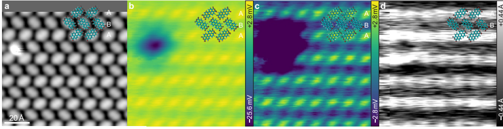
Figure 7.3: Measuring the electrostatic potential over a PTCDA on Ag(111) layer containing a defect (damaged molecule B by field emission). The overlay shows the molecular structure and molecule A and B are indicated. a , STM topography of PTCDA/Ag(111) monolayer (setpoint: 0.35 V, 0.2 nA). b , and c , SQDM V^* images (STC controller) with full contrast range emphasizing the defect in b and limited range emphasizing the intralayer contrast in c . d , Corresponding dielectric topography image of t_d = (\alpha_{rel} - 1)/g [89]. g was estimated from calibration measurements to be g \approx 0.08 \text{ \AA}^{-1} .
