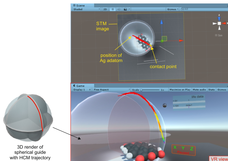
Figure 5.3: Screenshot of experiment using HCM Unity™ version. The bottom window, highlighted in red, shows the view seen by the experimenter while wearing VR goggles. The trajectories display the colour coded conductance signal, from red (low values) to purple (high values).
