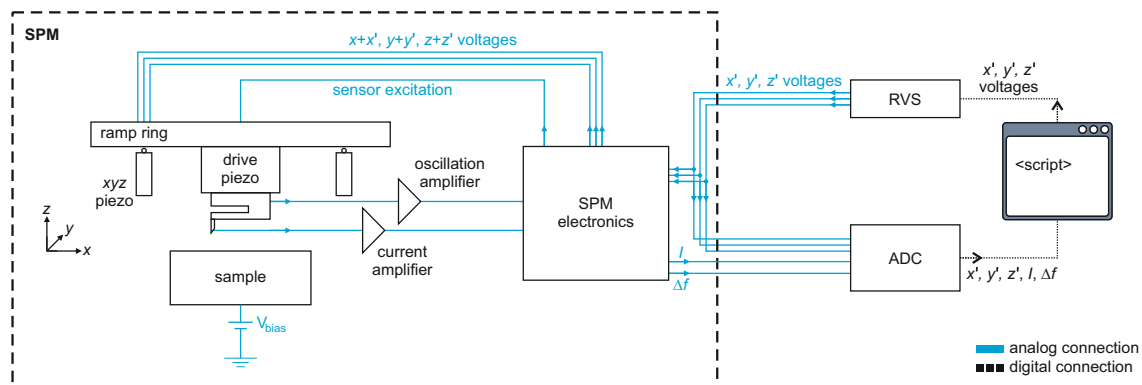
Figure 2.8: Schematic of the extended SPM setup.
