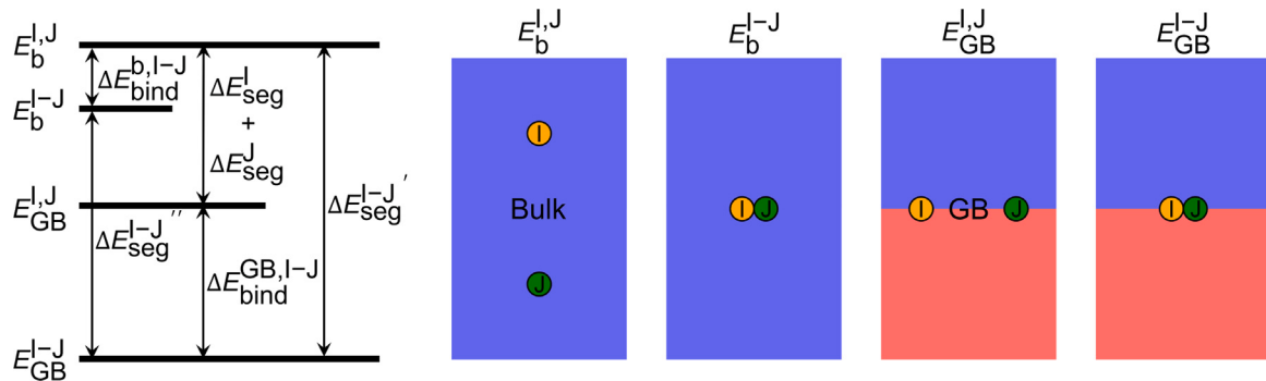
Fig. 6. Schematic illustration of the relationships between energy states ( E ), segregation energies ( \Delta E_{\text{seg}} ), co-segregation energies ( \Delta E_{\text{seg}}^{I-J} ), and binding energies ( \Delta E_{\text{bind}}^{I-J} ) for solutes I and J in bulk Mg and at the GB.
