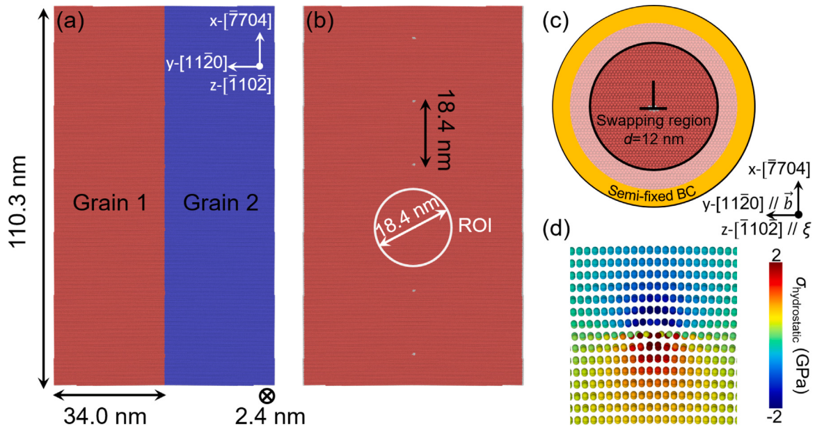
Fig. 2. Atomistic configuration of the symmetric tilt LAGB with a misorientation of 1^\circ along the [1\bar{1}0\bar{2}] rotation axis on the (11\bar{2}0) GB plane. (a) Slab setup ( 110.3 \times 68.0 \times 2.4 \text{ nm}^3 ) of the symmetric tilt LAGB with periodic boundary conditions in x and z directions. (b) The relaxed symmetric tilt LAGB, consisting of an array of edge dislocations with identical core structures and a spacing of 18.4 nm. Atoms are colored according to the common neighbor analysis [62], with white indicating atoms at dislocation cores and red for those in the matrix. (c) Schematic of the cylindrical setup ( d=18.4 \text{ nm} , l_z=2.4 \text{ nm} ) used for solute segregation calculation at the dislocation, featuring semi-fixed boundary conditions (constrained in x and y directions) at outermost layers with a thickness of 1.2 nm. (d) Hydrostatic stress map illustrating the stress fields around the dislocation core region, where blue and red regions represent compressive and tensile stress fields of the edge dislocation, respectively. (For interpretation of the references to color in this figure legend, the reader is referred to the web version of this article.)
