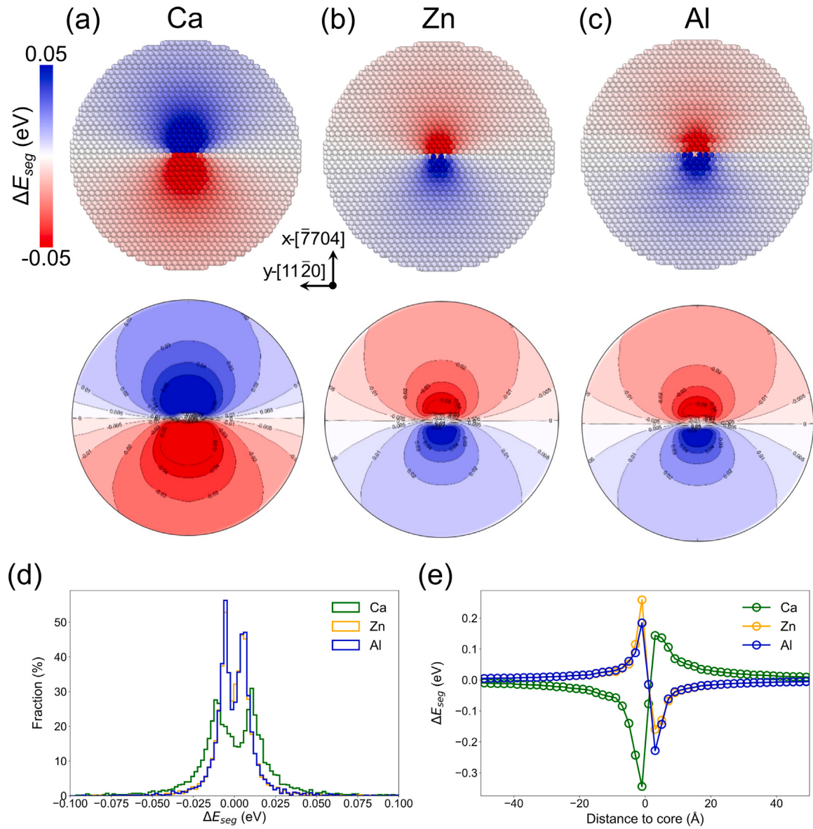
Fig. 5. Mono-segregation behavior of (a) Ca, (b) Zn and (c) Al solutes at the dislocation. Upper row: Atomistic simulations; lower row: Interaction energy fields between the solute modeled as an elastic dipole and the strain field of the dislocation. A negative value of \Delta E_{\text{seg}} indicates that segregation is energetically favorable. (d) Distribution of \Delta E_{\text{seg}} for Ca, Zn and Al solutes with data grouped into bins of 2 meV. (e) Statistics of \Delta E_{\text{seg}} as a function of distance to the center of the dislocation core. Negative distances correspond to the tensile stress region, whereas positive distances indicate the compressive stress region. Data is divided into bins of 2 Å.
