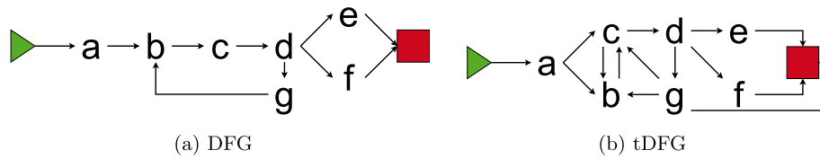
Fig. 5 DFG and tDFG obtained from translucent event log L = [\langle a, bc, c, d, efg \rangle, \langle a, bc, c, d, efg \rangle, \langle a, bc, c, d, efg, bc, c, d, efg \rangle]
