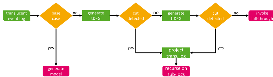
(a) IMf only using tDFGs (IMfto)
