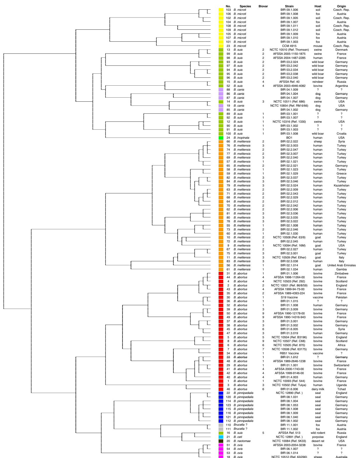
Figure 3 Cluster analysis of Brucella field isolates based on biochemical reactions. Cluster analysis of 113 Brucella strains including the reference strains and two isolates of a potentially new species that originated from Austrian foxes based on 93 biochemical reactions tested with the newly developed Brucella specific Micronaut™ microtiter plate. Hierarchical cluster analysis was performed by the Ward's linkage algorithm using the binary coded data based on the empirically set cut-off.
