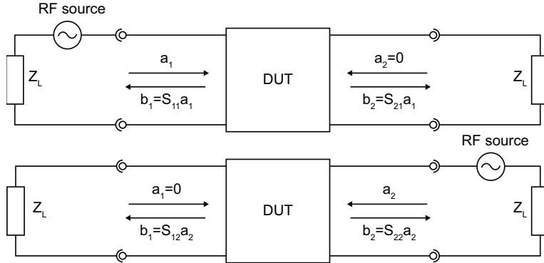
Figure 7.1: Circuitry for the determination of the S -parameters S_{11} and S_{21} (top) and S_{12} and S_{22} (bottom).
