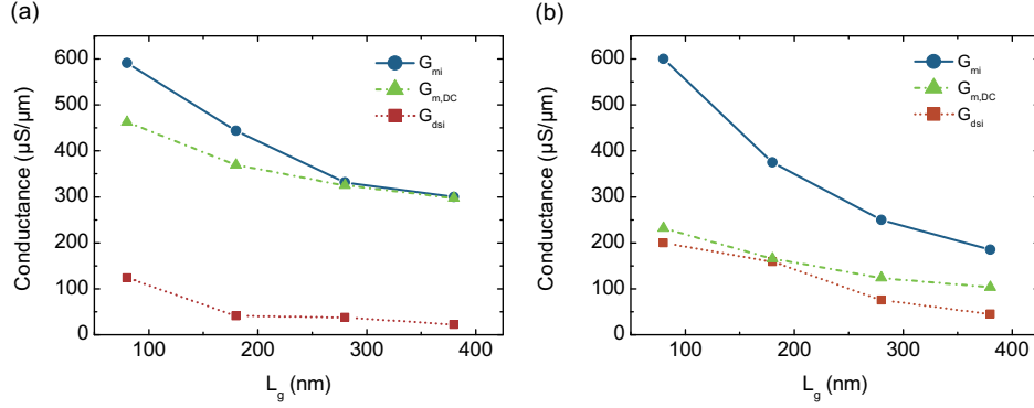
Figure 7.18: Intrinsic transconductance G_{mi} , output conductance G_{dsi} and maximum DC transconductance G_{m,DC} versus gate length L_g in saturation for (a) n-type and (b) p-type SB-MOSFETs.
