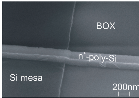
Figure 5.5: SEM image (60° tilted) of the Si mesa of a SB-MOSFET on thin-body SOI ( t_{\text{Si}} = 30\text{ nm} ) with a 3.5 nm gate oxide and a 160 nm thick \text{n}^+ -poly-Si gate; the channel length is 180 nm.
