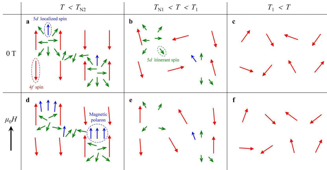
Figure 5 | Schematic illustration of the spin states with and without applied magnetic field, \mu_0 H , in different temperature regimes. (a–c) At zero magnetic field. (d–f) At applied magnetic field of \mu_0 H . When T > T_1 , spin moments more or less rotate (f), depending on the strength of \mu_0 H and the size of MA, from a pure PA state (that is strictly observing the Curie-Weiss law as shown in Supplementary Fig. S4) in (c). When T_{N1} < T < T_1 , the short-range AFM spins that are attributed only to the local 4f moments appear (b) accompanied by the generations of polarized itinerate 5d spins, based on the deviation of the unit-cell volume from the Grüneisen model shown in Fig. 1b, and possible small amount of localized 5d spins according to equation (1). Applied magnetic field mainly aligns the local AFM spins (e), leading to a decrease of the electron-spin scattering and resultant the NMRV. When T < T_{N2} , the LRO AFM state with almost equivalent AFM and FM interactions (see Supplementary Fig. S4) forms (a) with more itinerate 5d moments (based on the large PMV effect shown in Fig. 1b). Applied magnetic field mainly localizes more 5d moments by enhancing the exchange of J in equation (1), resulting in the formation of magnetic polarons and the consequent PMRV (d).
