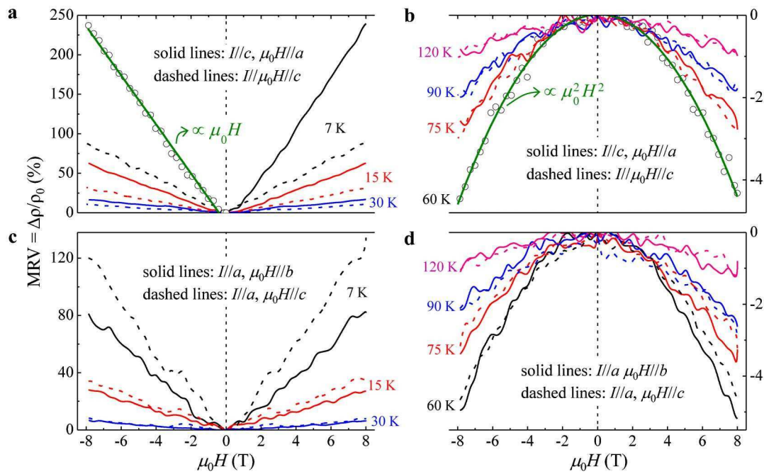
Figure 4 | Field- and temperature-dependent MR values. (a) Field and temperature dependencies of the MR values with I \parallel c -axis and applied magnetic field, \mu_0 H , along the a or c axis below T_N , and (b) above T_N . The representatives of the linear-field dependence of the PMRV (i.e., the PMRV is proportional to the strength of applied magnetic field) at 7 K (below T_N ) and the quadratic variation of the NMRV (i.e., the absolute NMRV is proportional to the square of the strength of applied magnetic field) at 60 K (above T_N ) were shown in (a) and (b), respectively. (c) Field and temperature dependencies of the MR values with I \parallel a -axis and applied magnetic field, \mu_0 H , along the b or c axis below T_N , and (d) above T_N .
