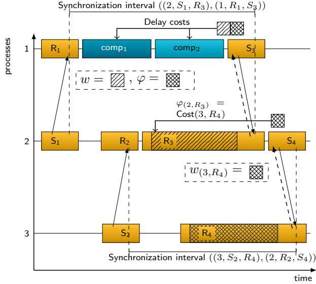
Figure 4.4: Source-related accounting of long-term costs via backward replay and successive accumulation of indirectly induced waiting time. The waiting time w_{(3,R_4)} first travels to its immediate cause, wait state R_3 on process 2, from where it is propagated further to its ultimate cause, the delay on process 1.
