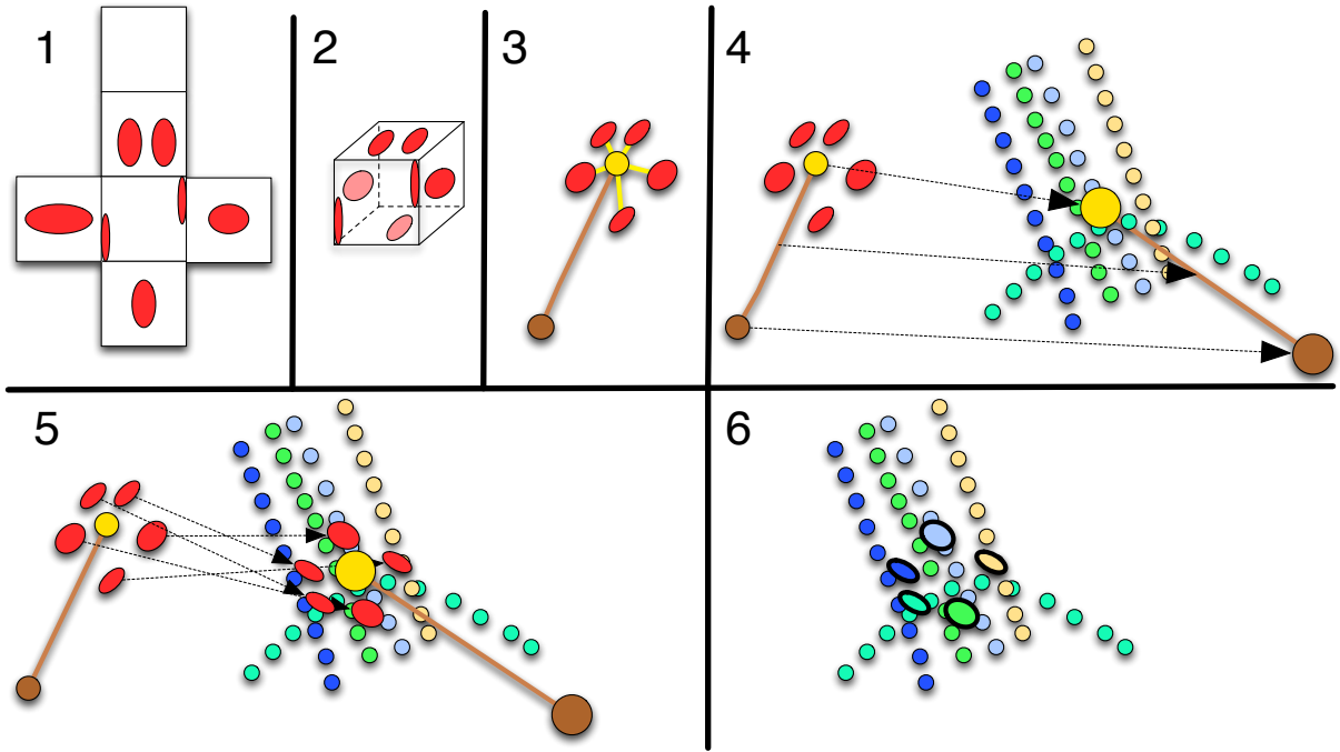
Figure 6.7: The algorithm to infer the hand posture. Rotation around the connection line is omitted in this sketch: 1: Detect ellipses on touch sensor input. 2: Select five touches and map to 3D coordinates. 3: Calculate center of gravity, guess hand origin. 4: Get transformation from input space to model space. 5: Apply transformation to touch points. 6: Assign finger labels to touch points.
