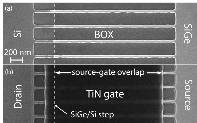
Figure 5.3: Top view SEM image of the heterostructure NW array (a) before and (b) after gate stack deposition and patterning.
