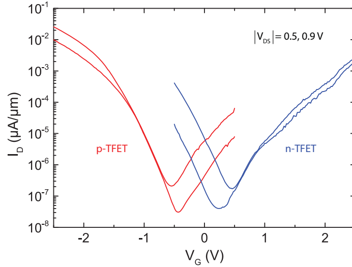
Figure 6.6: I_D - V_G characteristics of p-channel and n-channel SSOI NW array TFETs with 2\mu\text{m} gate length..
