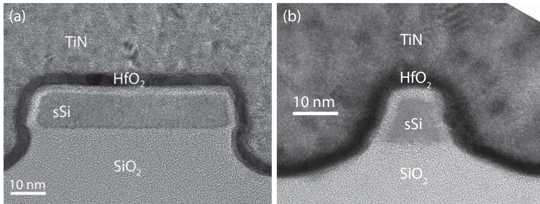
Figure 3.3: Cross-sectional transmission electron microscope (TEM) images of single NWs with (a) 10 \times 50 \text{nm}^2 and (b) 10 \times 10 \text{nm}^2 in a SSOI NW array TFET with high- \kappa /metal gate.
