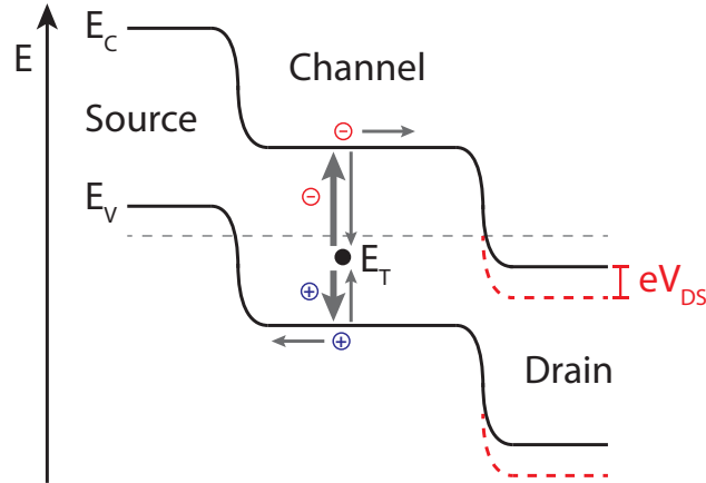
Figure 2.7: Illustration of the SRH generation-recombination process at trap states within the band gap. Under reverse bias conditions holes flow to the p-doped source and electrons to the n-doped drain.
