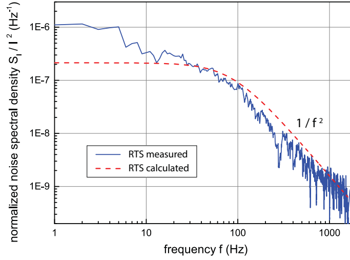
Figure 7.7: Current noise spectrum of the RTS noise calculated by subtracting an average of spectra without RTS noise from the spectrum at V_G = -2\text{ V} (blue solid line). Calculated two level RTS noise spectrum for lifetimes extracted from the measured RTS (red dashed line) shows good agreement with measured RTS spectrum.
