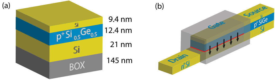
Figure 5.2: (a) Illustration of the in situ boron doped p^+Si_{0.5}Ge_{0.5} on SOI layer stack with corresponding layer thicknesses. The SiGe layer is biaxially compressive strained due to the pseudomorphic growth on the SOI; (b) Schematic of a single NW of the heterostructure n-channel TFET. The tri-gate covers the the step in the nanowire. The vertical tunnel direction from the p^+Si_{0.5}Ge_{0.5} in to the bottom Si layer is indicated with black arrows. The tunnel junction is marked with a red line.
