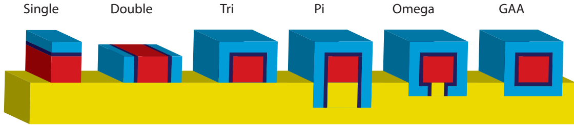
Figure 2.9: Schematic of various gate configuration types.
