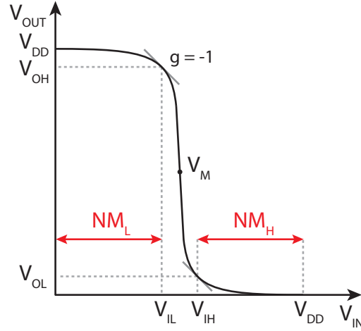
Figure 6.2: Schematic voltage transfer characteristics of an inverter.
