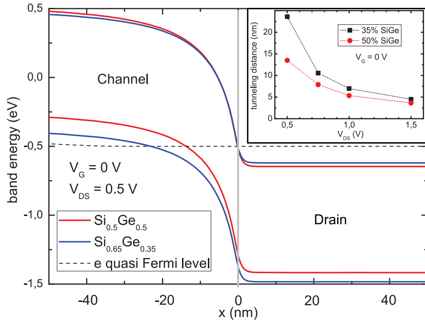
Figure 4.8: Simulated valence and conduction band energies at the channel drain junction for a \text{Si}_{1-x}\text{Ge}_x TFET with x = 35\% and 50\% Ge content. The TFET is in the off-state with V_G = 0\text{ V} and V_{DS} = 0.5\text{ V} . The inset shows the decrease of tunneling distance for increasing V_{DS} for the different Ge contents.
