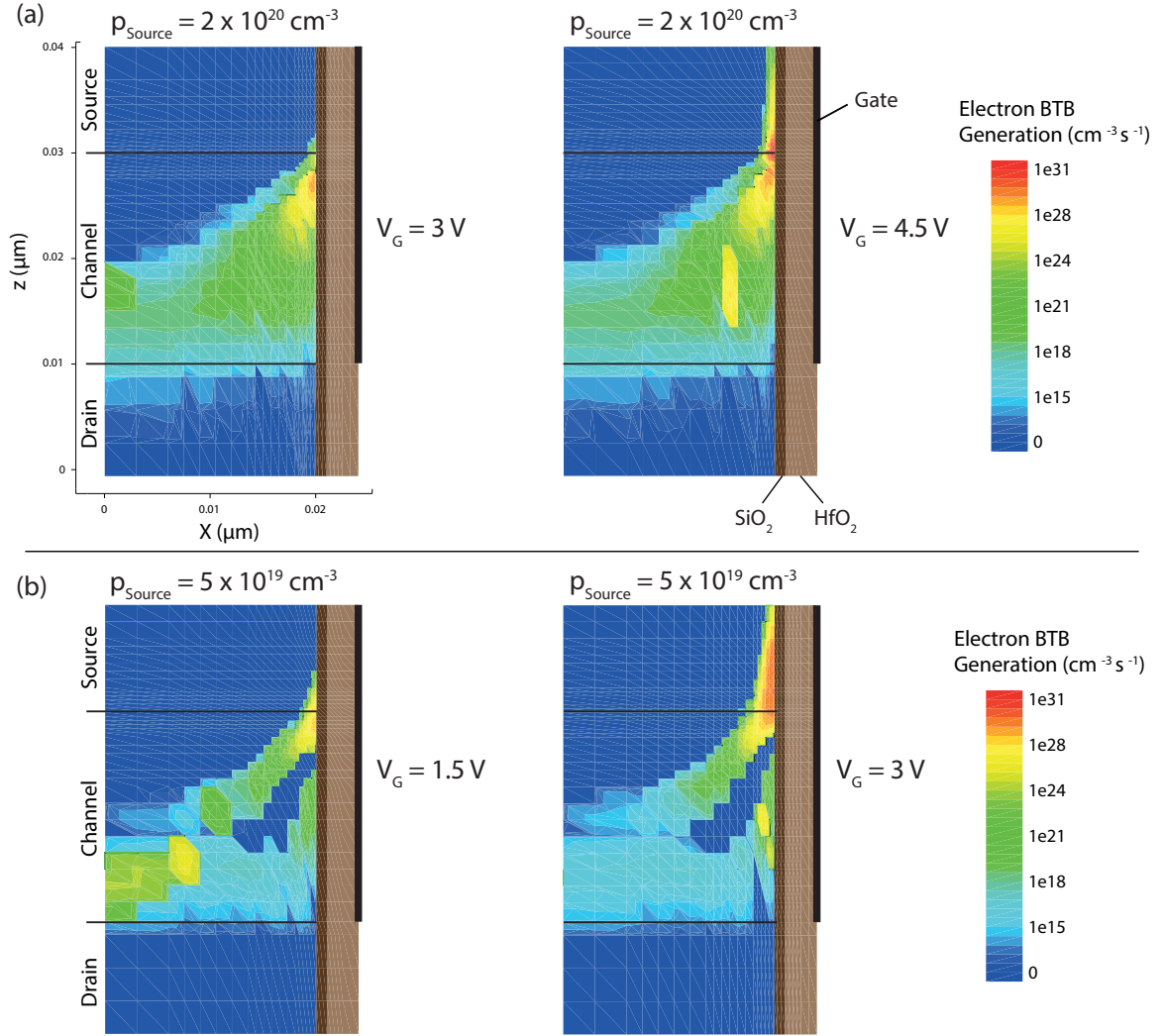
Figure 5.13: Simulated electron BTB generation in the right half of the simulated structure for (a) p_{source} = 2 \times 10^{20} \text{ cm}^{-3} and (b) 5 \times 10^{19} \text{ cm}^{-3} at different values of V_G .
