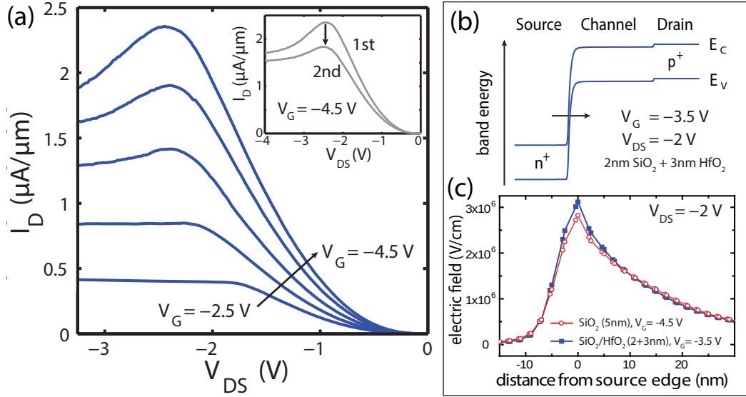
Figure 3.15: (a) Output characteristics of p-channel NW TFET with 100 nm gate length and 50 nm NW width. Negative differential conductance occurs for |V_G| \geq 3.5 V. Inset shows the deterioration of repeatedly measured I_D - V_{DS} curves; (b) Simulated band energies of valence and conduction band under bias condition V_G = -3.5 V and V_{DS} = -2 V; (c) Electric field as a function of the distance from the source-channel junction.
