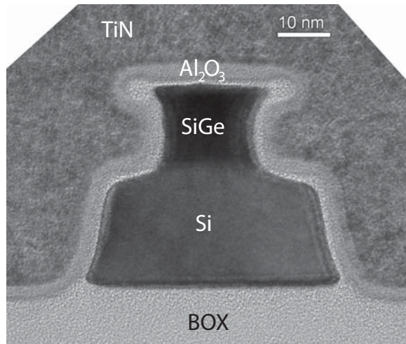
Figure 4.4: Cross-sectional TEM of a single SiGe on SOI NW with \text{Al}_2\text{O}_3/\text{TiN} gate stack.
