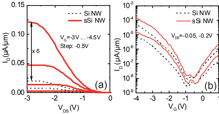
Figure 3.4: (a) Output and (b) transfer characteristics of strained Si NWs with \text{HfO}_2/\text{poly-Si} gate stack fabricated by Sandow [83].
