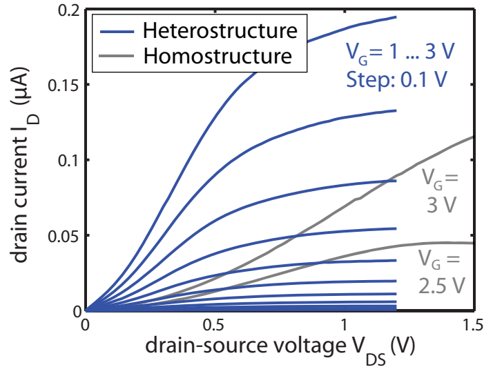
Figure 5.5: Output characteristics of a n-channel \text{Si}_{0.5}\text{Ge}_{0.5}/\text{Si} heterostructure NW TFET with 2\mu\text{m} gate length (blue). In comparison output characteristics of the homostructure \text{Si}_{0.5}\text{Ge}_{0.5} NW TFET from chapter 4 are shown in gray. Currents are normalized per NW in the array for both devices.
