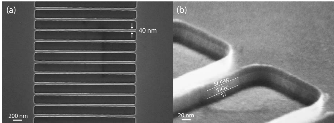
Figure 4.3: (a) Top view SEM image of a SiGe on SOI NW array with 2.4 \mu\text{m} long and 40 nm wide NWs; (b) Tilted angle SEM image of a NW array etched into a Si/Si 0.5 Ge 0.5 /Si stack with Cl 2 /Ar dry etching.
