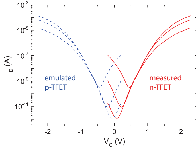
Figure 6.10: Measured transfer characteristics of an n-channel SiGe/Si nanowire array TFET and emulated p-channel transfer characteristics.
