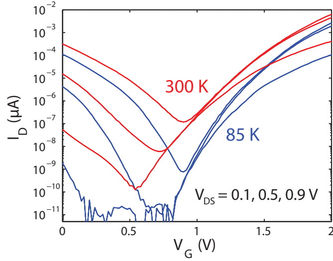
Figure 5.8: Transfer characteristics of a n-channel \text{Si}_{0.5}\text{Ge}_{0.5}/\text{Si} heterostructure NW TFET with 2\,\mu\text{m} gate length measured at 85 and 300 K. Currents are normalized per NW.
