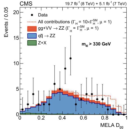
Fig. 3. Distributions of (top) the four-lepton invariant mass after a selection requirement on the MELA likelihood discriminant \mathcal{D}_{gg} > 0.65 , and (bottom) the \mathcal{D}_{gg} likelihood discriminant for m_{4\ell} > 330 GeV in the 4\ell channel. Points represent the data, filled histograms the expected contributions from the reducible ( Z + X ) and q\bar{q} backgrounds, and from the gluon fusion ( gg ) and vector boson fusion ( VV ) SM processes (including the Higgs boson mediated contributions). The dashed line corresponds to the total expected yield for a Higgs boson width and a squared product of the couplings scaled by a factor 10 with respect to their SM values. In the top plot, the bin size varies from 20 to 85 GeV and the last bin includes all entries with masses above 800 GeV.
