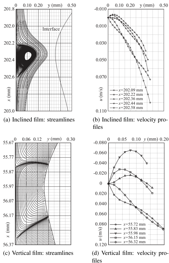
Fig. 11 Simulated streamlines and streamwise velocity profiles at the first capillary minimum for the inclined and vertical film.
