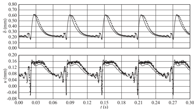
(a) y = 120 \mu\text{m}
