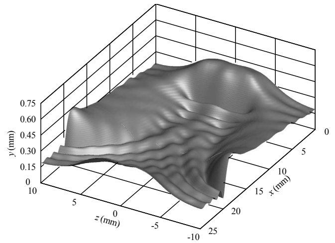
(a) Free surface topology (single spanwise wavelength)
