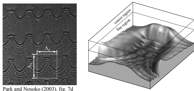
Fig. 8 Shadowgraph of the 3-dimensional film (with permission from John Wiley & Sons, Inc.), demarcating the periodic wave segment included in the computational domain. \Lambda_x=25 mm, \Lambda_z=20 mm.
