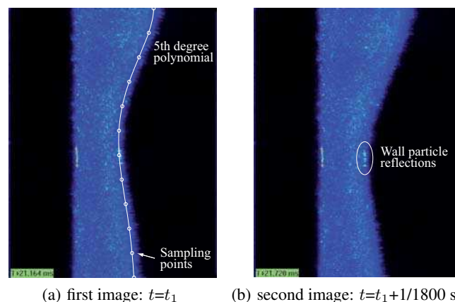
Fig. 6 Successive digital PIV images recorded with the CMOS camera in the region of the first capillary minimum.
