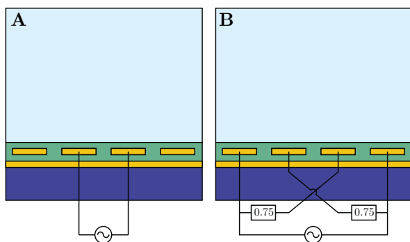
FIGURE 4.6: Cross-sectional schematic of the application of AC signals to the upper layer of wires. A: Supplying two wires with signals of AC_{in} and -AC_{in} will generate an AC voltage between the wires. B: Supplying four wires with amplitudes of AC_{in} , -0.75AC_{in} , 0.75AC_{in} , and -AC_{in} , respectively, will generate an electric field gradient pointing towards the center of the wires.
