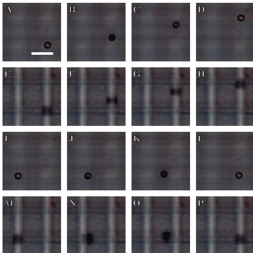
FIGURE 4.15: 3-dimensional actuation of a 2.7 μm particle. A-D: Image sequence of a particle being moved in the vertical direction. The video was recorded at the particle's levitation height. E-H: Equivalent frames taken from a video recorded at the chip's surface. I-L: Image sequence of a particle being moved in the horizontal direction. The video was recorded at the particle's levitation height. M-P: Equivalent frames taken from a video recorded at the chip's surface. Scale bar in A corresponds to 10 μm and applies to all images.
