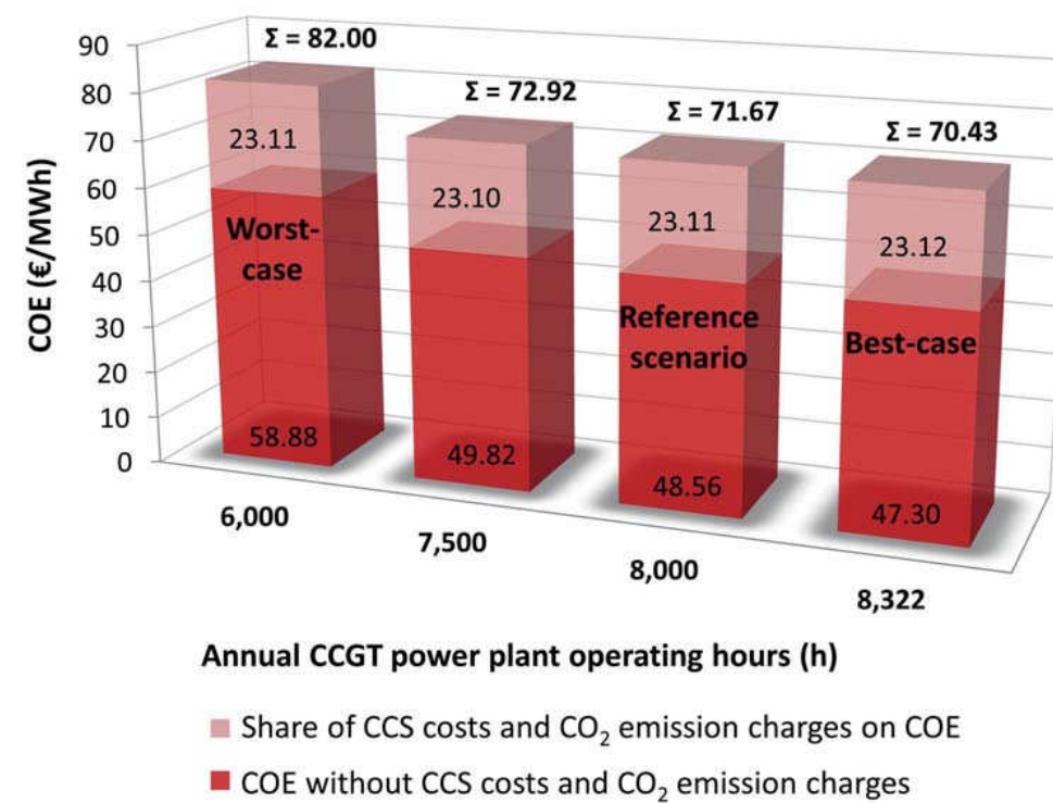
Figure 3.15: CCGT power plant operating hours variation from 6,000 hours to 8,322 hours causes an overall COE bandwidth of 11.6 €/MWh (including CO 2 emission handling costs), modified from Nakaten et al. (2014a).
