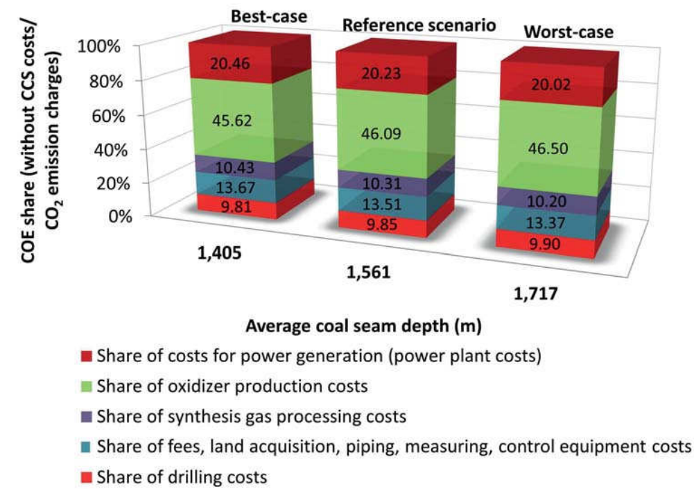
Figure 3.4: Coal seam depth variation by \pm 10\% compared to the reference scenario and the resulting percentage impact of fuel and power plant costs on costs of electricity (without CCS costs or \text{CO}_2 emission charges).
