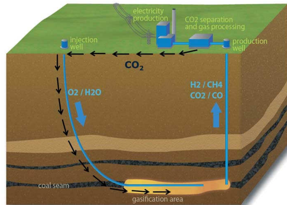
Figure 1.1: Schematic of a UCG process coupled to electricity generation with CO_2 capture and storage in the former UCG voids, modified from Kempka et al. (2009).
