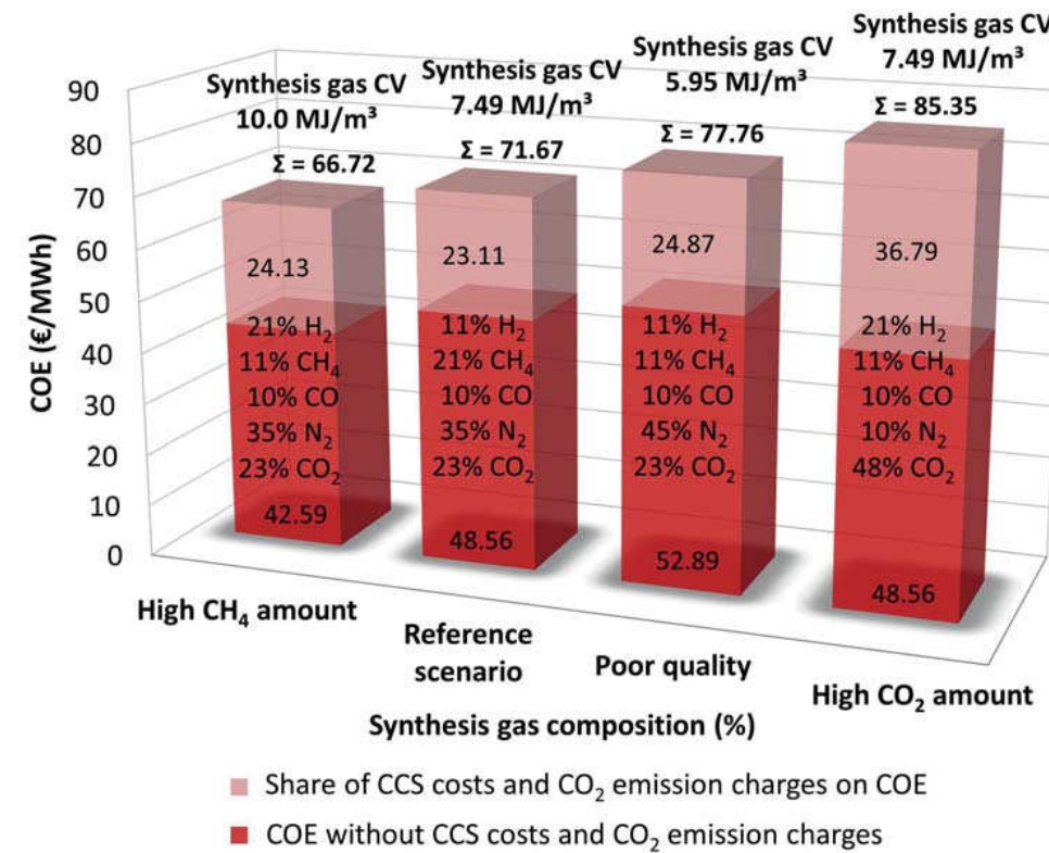
Figure 3.13: Variation of synthesis gas quality causes an overall COE difference of 18.6 €/MWh (including CO₂ emission handling costs), modified from Nakaten et al. (2014a).
