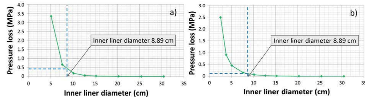
Figure 2.2: a) Pressure loss in injection wells during oxidizer injection (N 2 -O 2 gas mixture, average injection rate of 41.9 t/well/hour) and b) CO 2 injection (CO 2 single gas, average injection rate of about 8 t/well/hour) with an inner liner roughness of 0.0008 cm, modified from Nakaten et al. (2014b).
