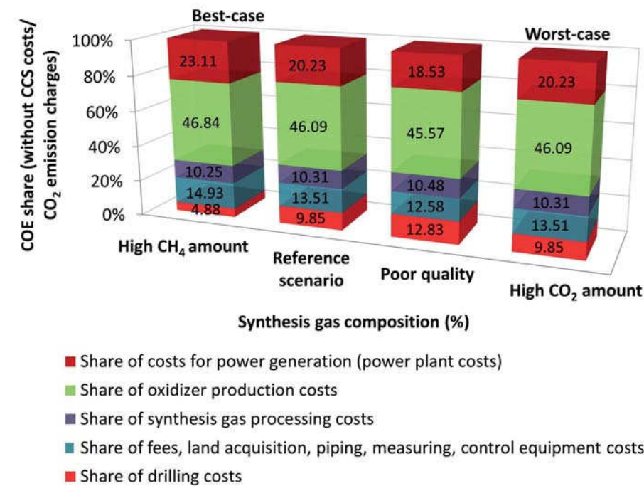
Figure 3.14: Variation of synthesis gas quality and the resulting percentage impact of fuel costs and other power plant costs on COE (without CCS costs or CO 2 emission charges), modified from Nakaten et al. (2014a).
