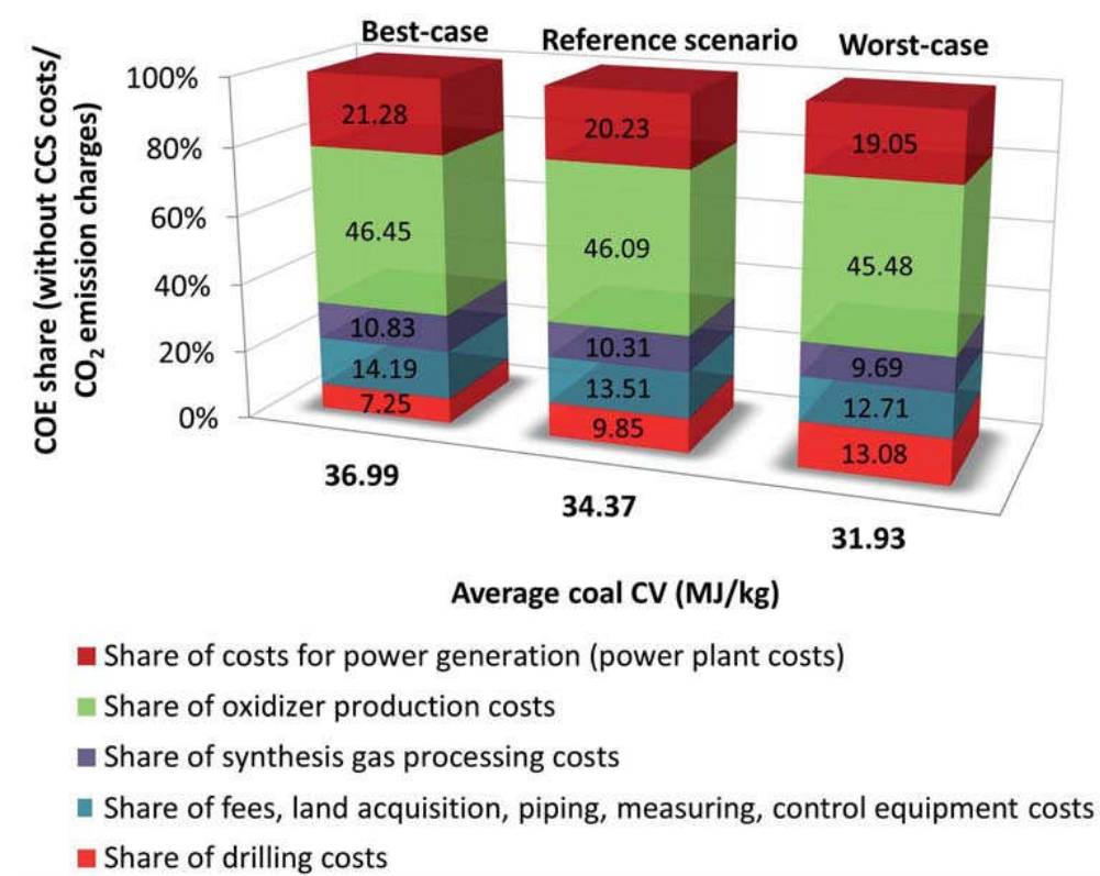
Figure 3.12: Coal CV_{Coal} variation by \pm 10\% compared to the reference scenario and the resulting percentage impact of fuel and power plant costs on COE (without CCS costs or CO 2 emission charges), modified from Nakaten et al. (2014a).
