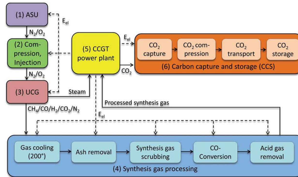
Figure 2.6: Techno-economic model developed for UCG-CCGT-CCS COE determination and its six sub-models, modified from Nakaten et al. (2012).
