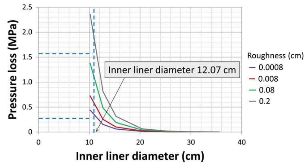
Figure 2.3: Pressure loss in synthesis gas production wells (H 2 -CH 4 -N 2 -CO 2 gas mixture, production rate of 92.8 t/well/hour) for different liner roughness, modified from Nakaten et al. (2014b).
