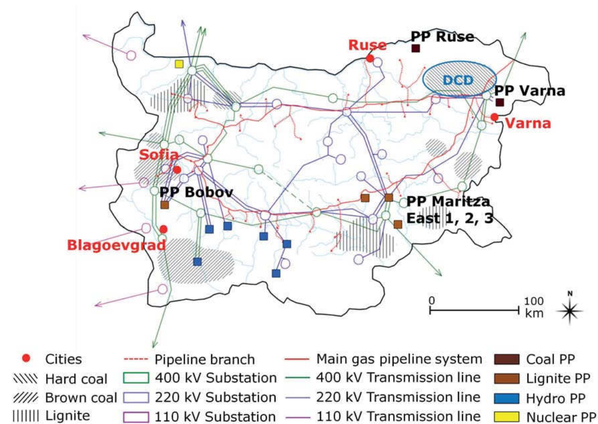
Figure 4.1: Bulgarian coal resources, energy infrastructure and largest power plants (PP), modified from Nakaten et al. (2013).
