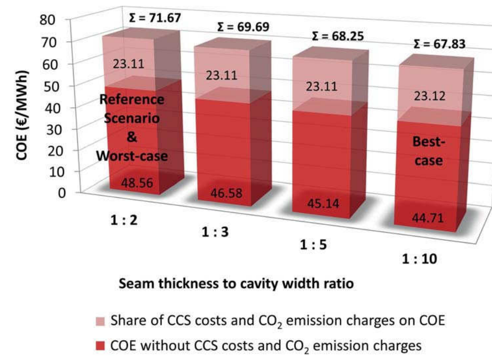
Figure 3.7: Coal seam thickness to cavity width ratio variation from 1:2 to 1:10 causes a COE, margin of 3.8 €/MWh (including CO 2 emission handling costs), modified from Nakaten et al. (2014a).
