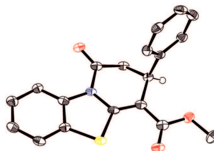
Figure 1 Absolute configuration [X-ray, x_{\text{abs}} = 0.078 (32)] of 3b
