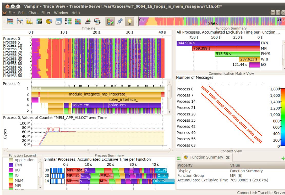
Figure 13: Vampir GUI.
