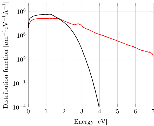
Fig. 7. Energy distribution function for electrons (red) and holes (black) in the middle of the p-n junction ( x = 2.5 \mu\text{m} ) at 37.172 V and room temperature for 10 pA/μm 2 (dashed lines) and for 10 nA/μm 2 (solid lines) scaled with the corresponding current density.
