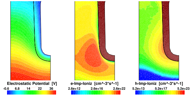
Fig. 8. Potential, electron, and hole II rates in the space-charge region of the vertical power MOSFET for a drain bias of 35.83 and 0 V at all other contacts for a current of 10 pA/μm 2 .
