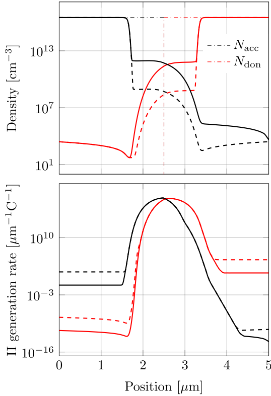
Fig. 6. Electron (red, top graph) and hole (black, top graph) density, and II generation due to electrons (red, bottom graph) and holes (black, bottom graph) at 37.172 V and room temperature for 10 pA/μm 2 (dashed lines) and 10 nA/μm 2 (solid lines). Doping profiles (dashed dotted, top graph).
