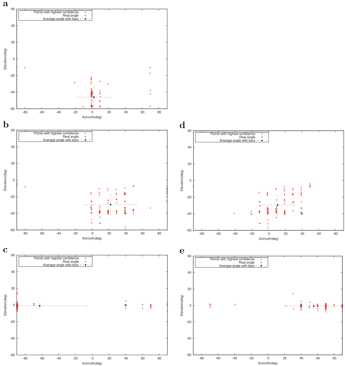
Figure 4.18: Localization in azimuth and elevation using the artificial owl ruff (funnels-only variant). a-c Localization using ITDs only. d-e Localization using the combination of ITDs and ILDs. Only a few exemplary positions are shown: a : (0^\circ, -40^\circ) ; b , d : (40^\circ, -40^\circ) ; c , e : (40^\circ, 0^\circ) . (Krämer, 2008)
