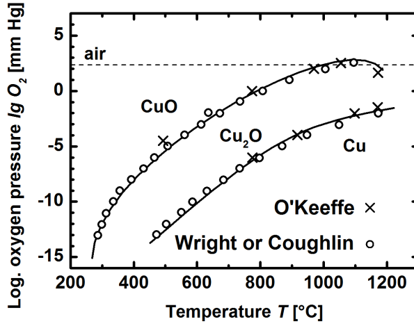
Figure 3.1 – P - T phase stability diagram of the \text{Cu} - \text{Cu}_2\text{O} - \text{CuO} system according to Rakhshani [23] comprising data from Wright (circle), Coughlin (circle) and O'Keeffe et al. (cross) [24, 25, 26].
