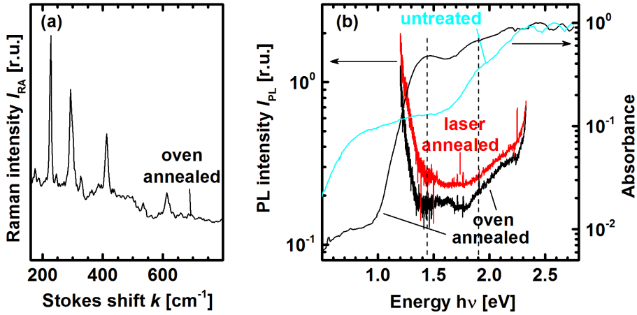
Figure 5.2 – Figure (a) illustrates the Raman spectrum of the iron oxide nanoparticles after the oven annealing step at 1000°C for 30 minutes under nitrogen atmosphere after Jan Flohre [21]. Figure (b) shows the corresponding PL and PDS spectra (black line). For comparison, the emission signal of the laser annealed nanoparticles (red line) and the absorbance of the as-prepared nanoparticles (cyan line) are presented.
