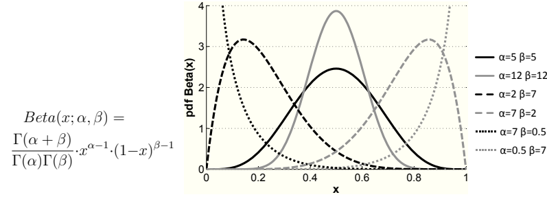
Figure 7.4: Probability density function of the Beta distribution
