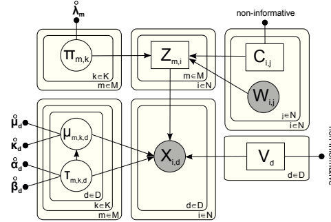
Figure 8.2: Graphical model of our method. Rectangles denote discrete random variables, circles continuous random variables, and black dots (deterministic) hyperparameters of the prior distributions.
