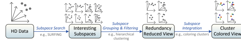
Figure 14.1: Our proposed analysis pipeline. A subspace selection algorithm is applied to automatically identify a candidate set of interesting subspaces. A filtering step reduces the potentially large and redundant set of automatically obtained subspaces to a user-selectable number of representing subspaces. Visual-interactive user exploration then proceeds on the subspace representations. Subspace analysis is also supported by comparative cluster views, allowing users to identify meaningful similar, complementary, or even conflicting clustering structures in the set of subspaces.
