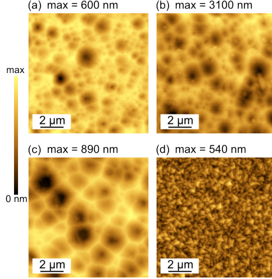
Figure 6.1.: Topographies of small feature sample (a) with heights up to 600 nm, stretched sample (b, heights up to 3100 nm), and large feature air and \mu c-Si:H sample (c) with heights up to 890 nm as measured by AFM. (d) shows the surface of the LPCVD-grown ZnO:B layer (heights up to 540 nm).
