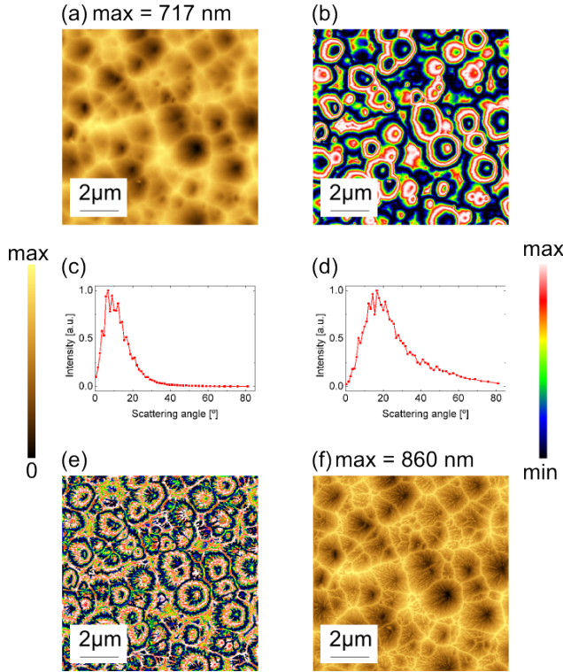
Figure 7.19.: Sketch of the topography optimisation by using FFT and PM. (a): The original texture that should be optimised. (b): The real part of the phase as obtained by PM. (c): The resulting FFT and AID. (d): FFT and AID after applying the high-pass filter. (e): The real part of the phase image obtained by iFFT. (f) The final result: An optimised texture calculated from the phase image. The structure is still very similar to the original texture, with smaller additional features inside the craters and the craters generally deeper and steeper. The additional features are rooted in small features which are small but present in the original texture. Also, some FFT artefacts can be seen, but these are not strongly pronounced.
