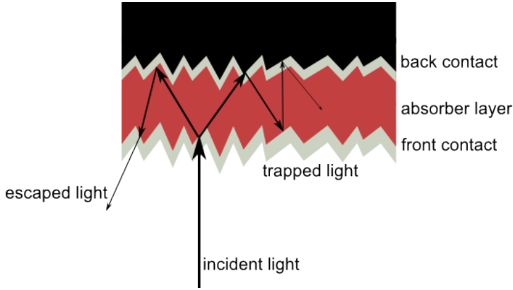
Figure 2.4.: Sketch of light trapping approximated using geometrical optics. A textured interface can scatter light into different angles. For small angles (left side), the light can couple out of the cell in the same way it could with flat interfaces, however the light path is increased by the angle. In the best case (right side), the light is scattered into an angle above the angle total internal reflection and trapped inside the absorber layer until it is absorbed.
