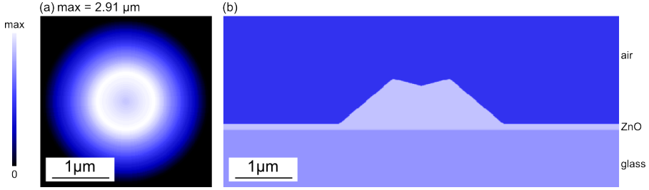
Figure 8.10.: Sketch of the crater used for investigating the influence of the SNOM tip; (a) shows a top-down view of the crater. It is assumed to be rotationally symmetric, with an inner (crater centre to rim) radius of 500 nm. (b) shows a cross-section of the crater. The inner and outer angles of the crater were set to 65^\circ and 55^\circ , respectively.
