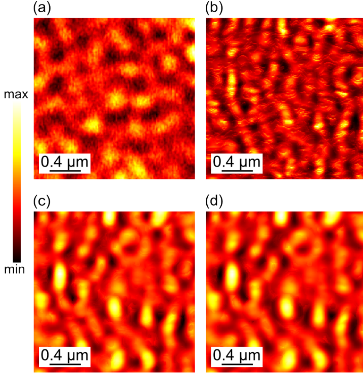
Figure 8.8.: Light intensity distributions from SNOM measurement and FDTD simulation of the AN 10 sample. (a) shows the intensity distribution as measured by SNOM. The shape of the features in this distribution is similar to those seen in the topography measurement (Fig. 8.6(a)). (b) shows the intensity distribution from FDTD simulation at a constant distance of 20 nm above the surface. There are many smaller features visible, as well as features that relate to near-field effects. (c) and (d) show the light intensity distribution obtained when taking into account the offsets obtained by the algorithm (Fig. 8.6(f) for the bad geometry). The agreement with the SNOM measurement is better for both geometries.
