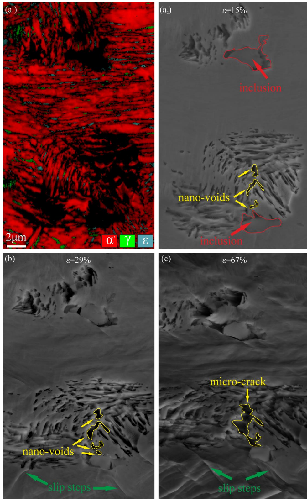
Figure 4.7: Interactions of micro-cracks with the surrounding phases in S_{8h} revealed by in-situ tensile test, as characterized by (a 1 ) EBSD phase map; (a 2 ) SE imaging of area in a 1 ; (b, c) SE imaging of this area after
