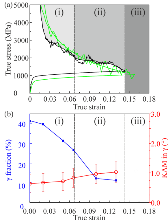
Figure 8.6: (a) True stress strain curve and strain hardening curve for M-A (AQ+8h) and M-A (CR+1h) ; (b) evolution of \gamma fraction (blue data points) and kernel average misorientation (KAM) in \gamma (red data points) during deformation of M-A (CR+1h) , as measured by EBSD. M-A (AQ+8h) : 600 °C 8 h annealed as-quenched \alpha' martensite; M-A (CR+1h) : 600 °C 1 h annealed cold-rolled \alpha' martensite.
