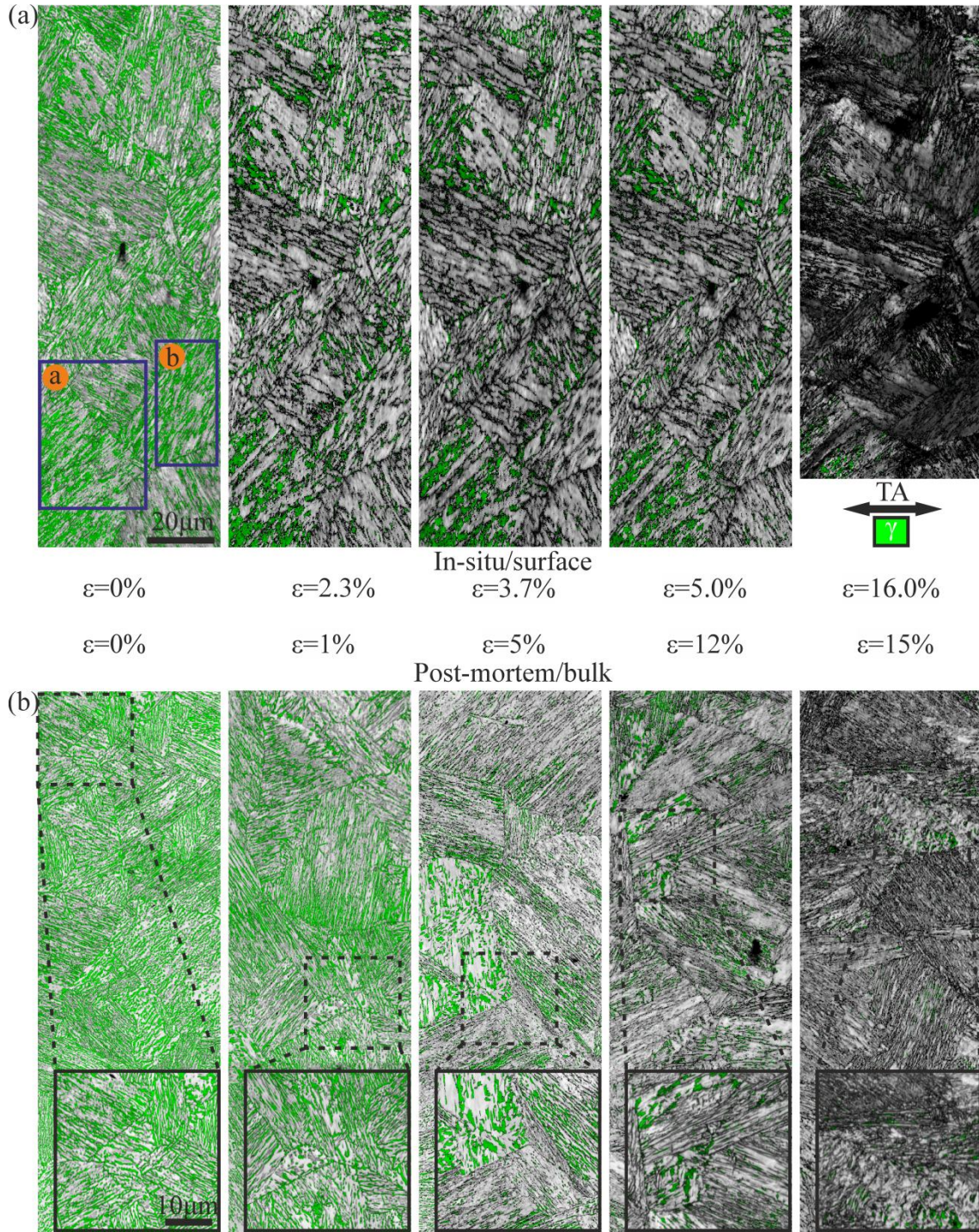
Figure 7.4: Evolution of \gamma_{\text{RN}} phase during (a) in-situ (surface data probed) and (b) post-mortem (bulk data probed) tensile tests. For the in-situ data set, two areas a-b are outlined and will be further analyzed in Figure 7.5. For the post-mortem data set, a magnified image is inserted for each map (TA: tensile axis). Source: Image from [35], Courtesy of Elsevier.
