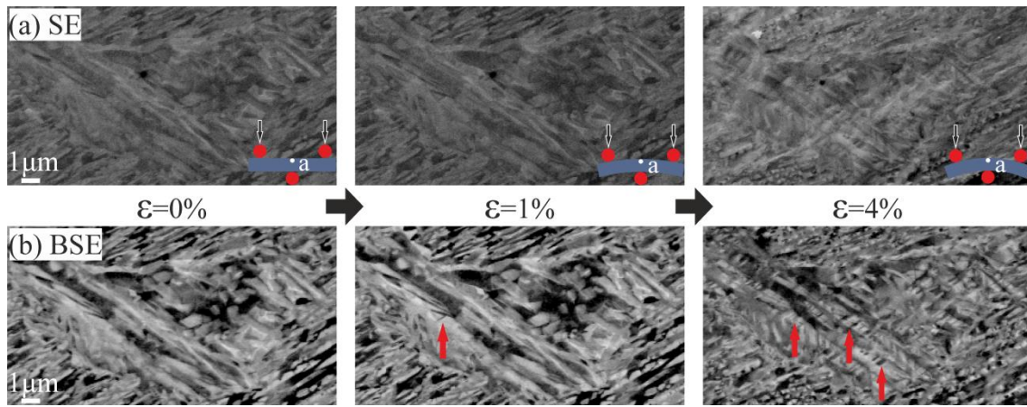
Figure 7.8: Investigation of the tension side of a sample during in-situ 3-point bending experiments by (a) secondary electron imaging, demonstrating the evolving surface morphology; and (b) electron channeling contrast imaging (ECCI), demonstrating the appearance of twin boundaries, as indicated by red arrows. Source: Image from [35], Courtesy of Elsevier.
