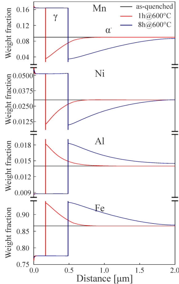
Figure 7.1: Predicted reversion of \alpha' martensite back into \gamma_{\text{RN}} in the current Fe-9Mn-3Ni-1.4Al-0.01C (mass %) TRIP-maraging steel at 600 °C for 1 h and 8 h, and the corresponding elemental partition of Mn/Ni/Al/Fe, simulated by Dictra using thermodynamic database TCFE7 and mobility database MOBF2. Source: Image from [35], Courtesy of Elsevier.
