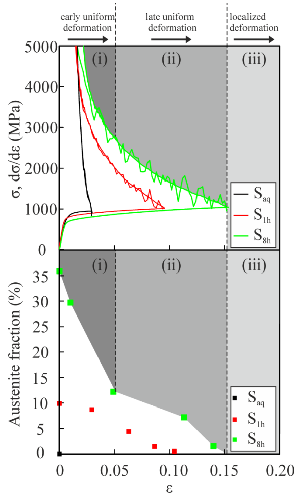
Figure 4.2: The true stress strain curve, the strain hardening ( d\sigma/d\epsilon ) curve and the evolution of \gamma_{RN} fraction during uniaxial tensile tests for S_{aq} , S_{1h} and S_{8h} . Three different deformation regimes are highlighted for S_{8h} . S_{aq} : as-quenched sample; S_{1h} : 1-hour heat treated sample; S_{8h} : the 8-hour heat treated sample. Source: Image from [33], Courtesy of Elsevier.
