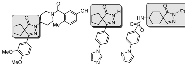
Scheme 1. General outline of the strategy employed herein and previous related work (H-Do denotes hydrogen-bonding donor).
