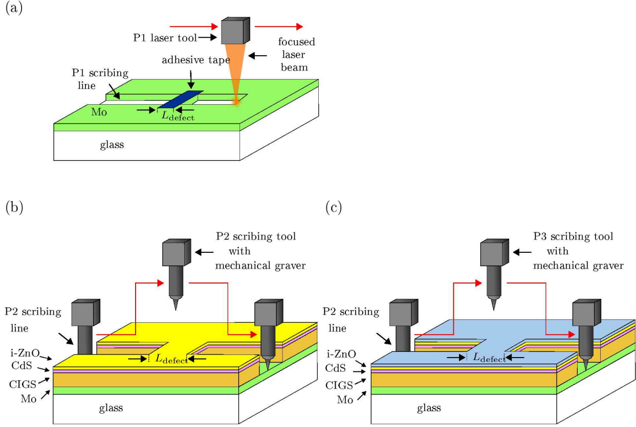
Figure 6.8: Implementation of scribing defects. (a) P1 scribing defect implementation with a tape that absorbs the laser energy. Here I show P1 film side scribing for the sake of a better visualisation, although P1 substrate side scribing has actually been applied. (b) P2 and (c) P3 scribing defect implementation by drawing back the mechanical graver during scribing process. Red arrow shows the moving direction of the correspondent scribing tool.
