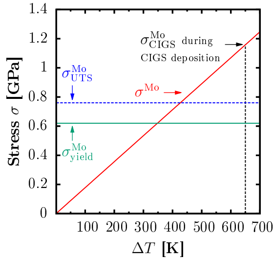
Figure 8.16: First order approximation of thermally induced mechanical stress \sigma^{\text{Mo}} imposed by the glass onto the Mo layer. The yield strength \sigma_{\text{yield}}^{\text{Mo}} required for irreversible deformation is exceeded at approximately \Delta T = 350 K, and the ultimate tensile strength \sigma_{\text{UTS}}^{\text{Mo}} required for creation of fractures at approximately \Delta T = 400 K. The actual CIGS deposition takes place at approximately \Delta T = 650 K with room temperature as reference.
