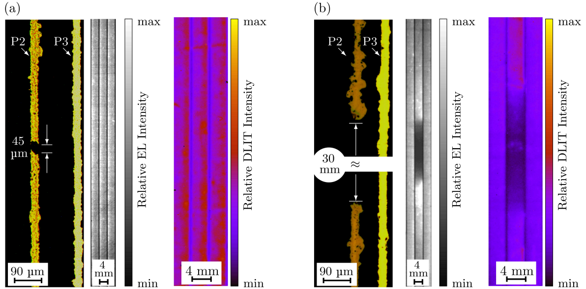
Figure 7.2: P2 defect appearance for (a) L_{P2} = 45 \mu\text{m} and (b) L_{P2} = 30 mm in microscope, EL, and DLIT images (EL and DLIT measured at j = 8.3 \text{mA}/\text{cm}^2 ). P2 defects are located at vertical centre between middle and right cell. Microscope images are recorded/illuminated from film side, microscope image in (b) is combined from two images due to the long L_{P2} .
