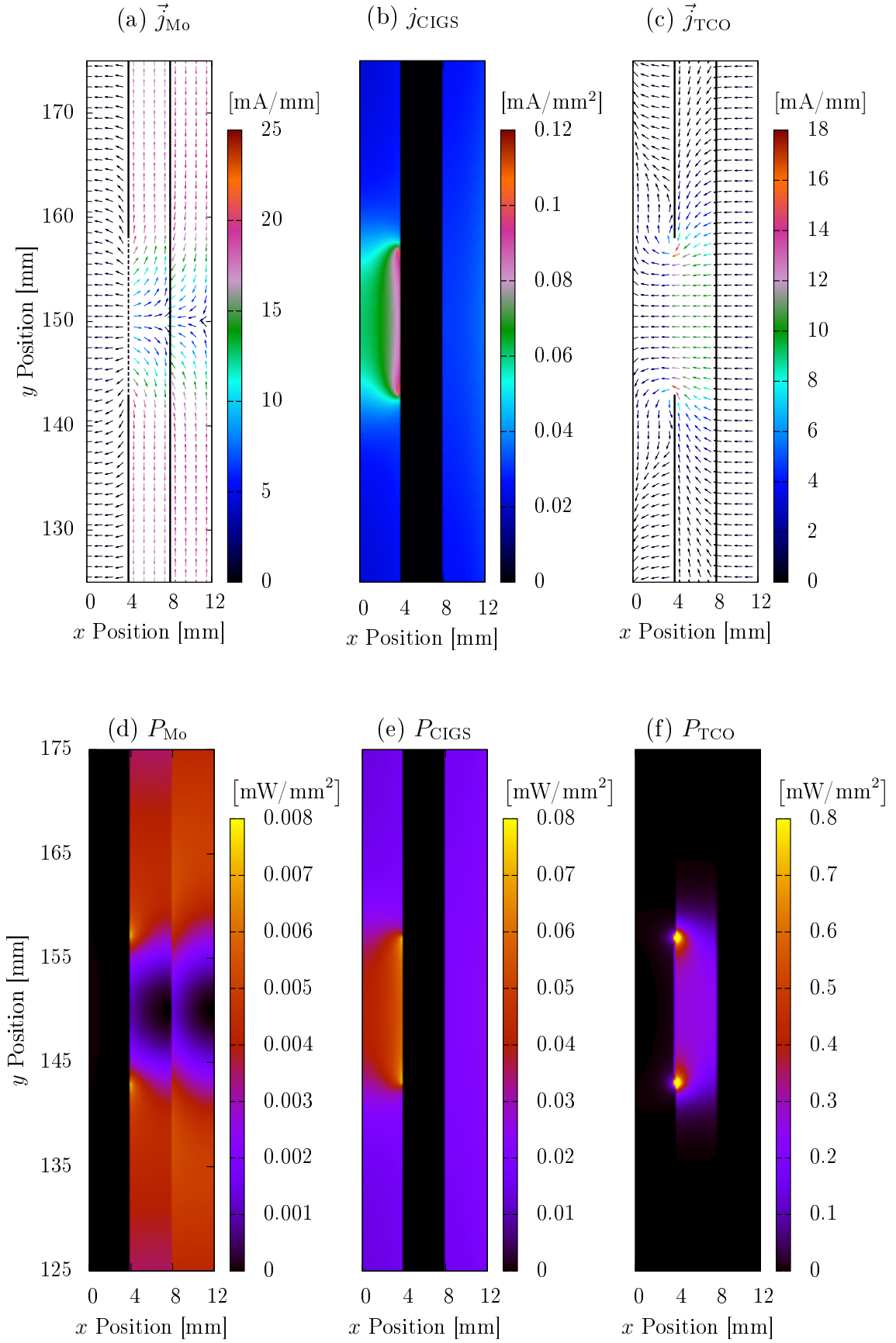
Figure 6.13: Simulation of a P3 defect of 14 mm length with j_{\text{DLIT}} = 8.3 \text{ mA/cm}^2 . (a) Horizontal current flow within Mo. (b) Vertical current flow through CIGS plus buffer layers. (c) Horizontal current flow within TCO. Correspondent power dissipation is shown in (d) - (f).
