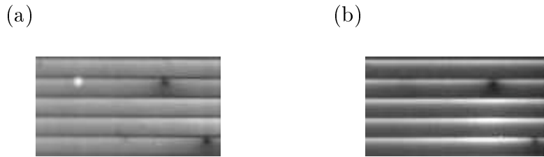
Figure 4.1: Influence of light soaking on EL image. EL image (a) before and (b) after 48 hours of light soaking at 800 W/m 2 intensity. White spot in the upper left part disappears and image contrast is increased during light soaking. This effect has been explained in [78].
