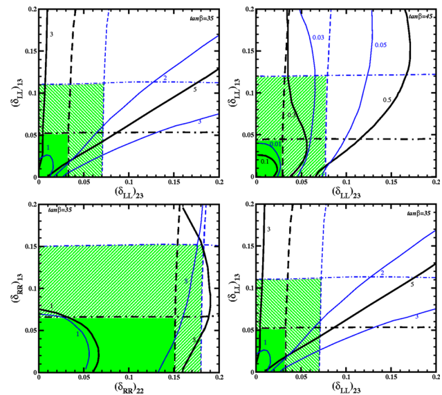
Fig. 143 Constraints on the magnitudes of the mixing parameters and possible LFV effects for reference points from [1261]. The shaded areas are those allowed by current limits on \text{BR}(\tau \rightarrow e \gamma) (dot-dash line) and \text{BR}(\tau \rightarrow \mu \gamma) (dash line) using four different reference points (shown by the thick lines bounding the solid shaded areas and the thin blue lines bounding the ruled shaded areas). The solid lines are contours of \sigma(e^+ e^- \rightarrow \tau^\pm \mu^\mp + 2\chi^0) in fb for \sqrt{s} = 2000 GeV
