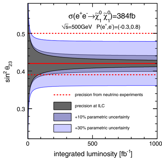
Fig. 8 Achievable precision on \sin^2 \theta_{23} from bi-linear R -parity-violating decays of the \tilde{\chi}_1^0 as a function of the produced number of neutralino pairs compared to the current precision from neutrino oscillation measurements [52]
