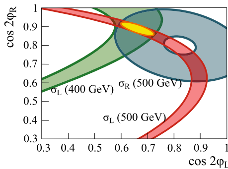
Fig. 137 Determination of the chargino mixing angles \cos 2\phi_{L,R} from LC measurements in e^+e^- \rightarrow \tilde{\chi}_1^+ \tilde{\chi}_1^- with polarised beams at different cms energies. The electroweak part of the spectrum in this scenario is a modified benchmark scenario SPS1a
