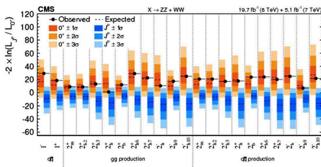
Fig. 29 Distributions of the test statistic q = -2 \ln(\mathcal{L}_{JP} / \mathcal{L}_{0+}) for the spin-1 and spin-2 JP models tested against the SM Higgs boson hypothesis in the combined X \rightarrow ZZ and WW analyses [117]. The expected median and the 68.3, 95.4, and 99.7 % CL regions for the SM Higgs boson (orange, the left for each model) and for the alternative J^P hypotheses (blue, right) are shown. The observed q values are indicated by the black dots
