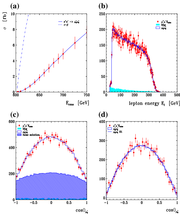
Fig. 133 a The unpolarised cross section of e^+e^- \rightarrow \tilde{\mu}_R^+ \tilde{\mu}_R^- production close to threshold, including QED radiation, beamstrahlung and width effects; the statistical errors correspond to \mathcal{L} = 10 \text{ fb}^{-1} per point, b energy spectrum E_\mu from \tilde{\mu}_R^- \rightarrow \mu^- \tilde{\chi}_1^0 decays; polar-angle distribution \cos \theta_{\mu_R} c with and d without contribution of false solution. The simulation for the energy and polar-angle distribution. The simulation for the energy and polar-angle distribution is based on polarised beams with (P_{e^-}, P_{e^+}) = (+0.8, -0.6) at \sqrt{s} = 1 \text{ TeV} and \mathcal{L} = 500 \text{ fb}^{-1} . For details, see Ref. [1172]
