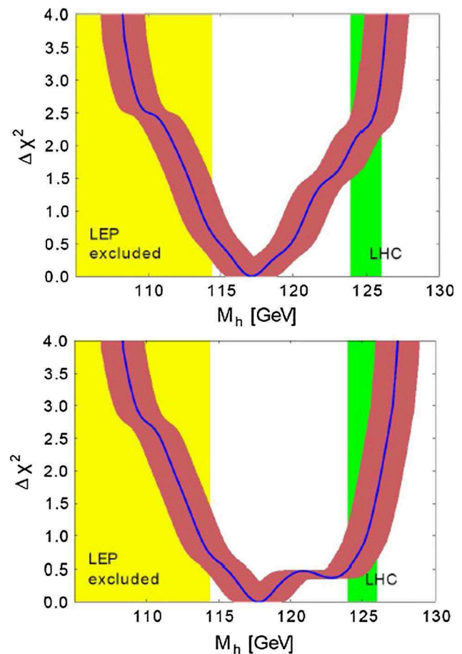
Fig. 62 Fit for the light \mathcal{CP} -even Higgs mass in the CMSSM (left) and NUHM1 (right) [254]. Direct searches for the light Higgs boson are not included
