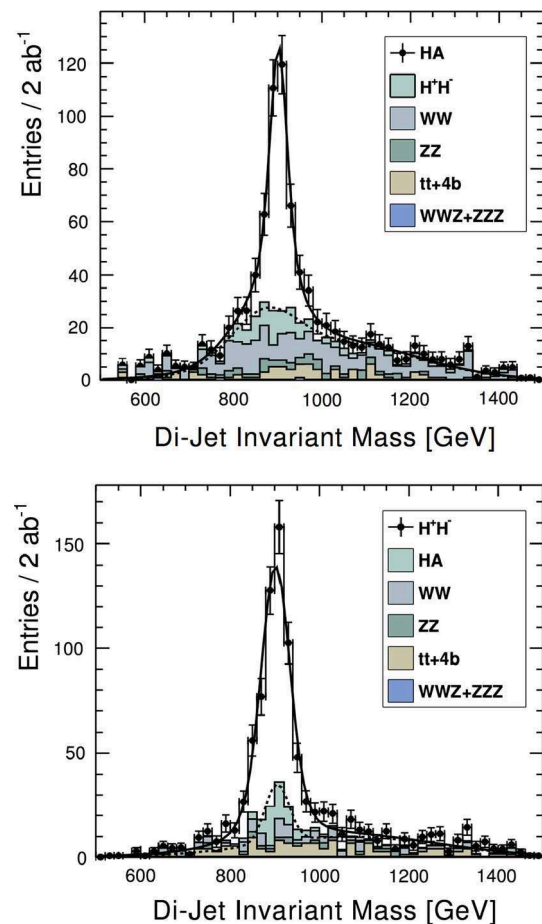
Fig. 13 Upper plot reconstructed 2-jet invariant mass for associated production: e^+e^- \rightarrow AH \rightarrow b\bar{b}b\bar{b} for a Higgs mass of 900 GeV at a collider energy of 3 TeV; lower plot similar plot for e^+e^- \rightarrow H^+H^- \rightarrow t\bar{t}b\bar{b}
