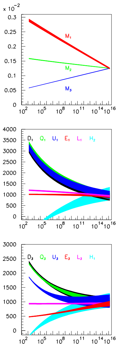
Fig. 142 Evolution of gaugino and sfermion (first and third generation) parameters in the CMSSM for m_0 = 966 GeV, m_{1/2} = 800 GeV, A_0 = 0 , \tan \beta = 51 , \text{sign} \mu = +1 [9, 10] to the GUT scale
