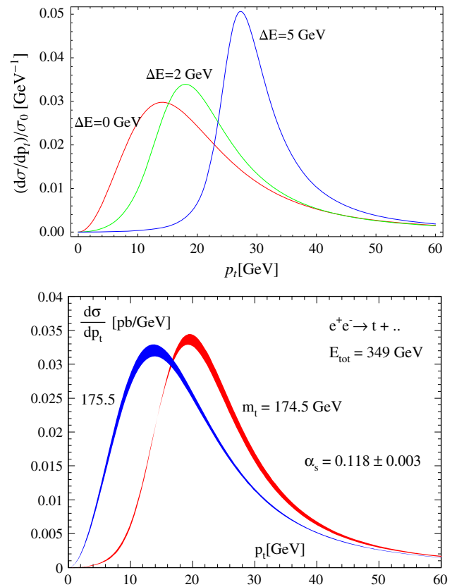
Fig. 106 Top quark momentum distribution at \Delta E = E - E_1 = 0, 2, 5 GeV (top) for m_t = 170 GeV and top-quark mass dependence (bottom) on the momentum distribution
