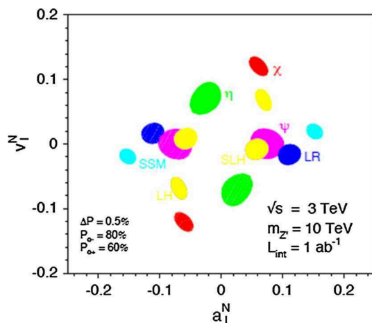
Fig. 10 New gauge bosons in the \mu^+\mu^- channel. The plot shows the expected resolution at CLIC with \sqrt{s} = 3 TeV and \mathcal{L} = 1 ab ^{-1} on the ‘normalised’ vector v_f^n = v_f \sqrt{s/(m_{Z'}^2 - s)} and axial-vector a_f^n = a_f \sqrt{s/(m_{Z'}^2 - s)} couplings to a 10 TeV Z' in terms of the SM couplings v_f, a_f . The mass of Z' is assumed to be unknown, nevertheless the couplings can be determined up to a two-fold ambiguity. The colours denote different Z' models [9, 10]
