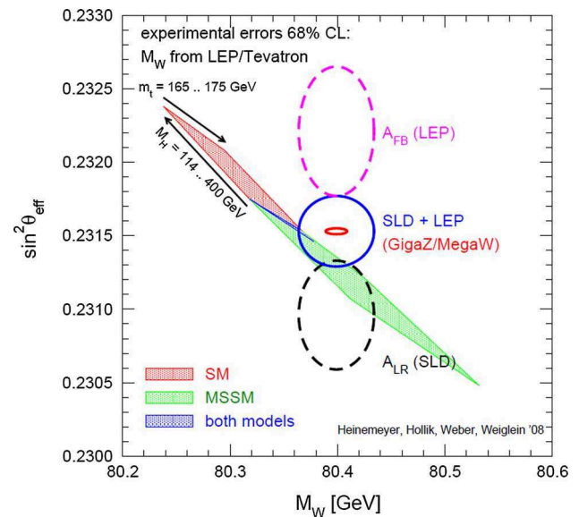
Fig. 114 MSSM parameter scan for M_W and \sin^2 \theta_{\text{eff}}^L over the ranges given in Eq. (116) with m_t = 165 \dots 175 \text{ GeV} . Today's 68 % CL ellipses (from A_{\text{FB}}^b (LEP), A_{\text{LR}}^e (SLD) and the world average) are shown as well as the anticipated GigaZ/MegaW precisions, drawn around today's central value
