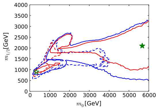
Fig. 155 The (m_0, m_{1/2}) planes in the CMSSM including the ATLAS 20/fb jets + \cancel{E}_T , \text{BR}(B_{s,d} \rightarrow \mu^+\mu^-) , m_h , \Omega_\chi h^2 , LUX, and other constraints. The most recent results are indicated by solid lines and filled stars, and previous fit based on \sim 5/\text{fb} of LHC data is indicated by dashed lines and open stars. The blue lines denote 68% CL contours, and the red lines denote 95% CL contours
