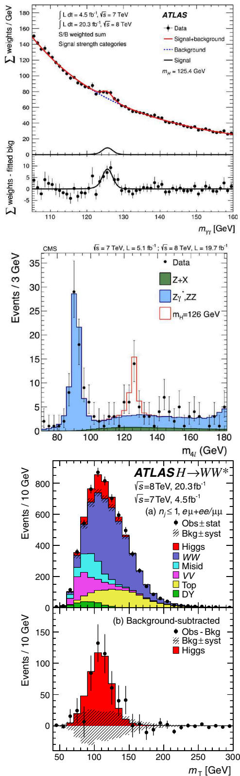
Fig. 15 Reconstructed distributions of the Higgs boson candidate decay products for the complete 2011/2012 data, expected backgrounds, and simulated signal from top the ATLAS H \rightarrow \gamma\gamma [101], centre the CMS H \rightarrow ZZ \rightarrow 4\ell [102], and bottom the ATLAS H \rightarrow WW \rightarrow 2\ell 2\nu [103] analyses
