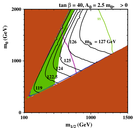
Fig. 151 The (m_{1/2}, m_0) plane for \tan \beta = 40 and \mu > 0 , assuming A_0 = 2.5m_0 , m_t = 173.2 GeV and m_b(m_b)_{\text{SM}}^{\overline{\text{MS}}} = 4.25 GeV. Contours and shaded regions are described in the text
