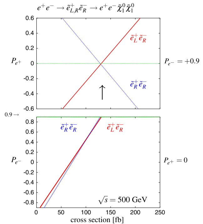
Fig. 5 Polarised cross sections versus P_{e^-} (bottom panel) and P_{e^+} (top panel) for e^+e^- \rightarrow \tilde{e}\tilde{e} -production with direct decays in \tilde{\chi}_1^0 e in a scenario where the non-coloured spectrum is similar to a SPS1a-modified scenario but with m_{\tilde{e}_L} = 200 GeV, m_{\tilde{e}_R} = 195 GeV. The associated chiral quantum numbers of the scalar SUSY partners \tilde{e}_{L,R} can be tested via polarised e^\pm -beams
