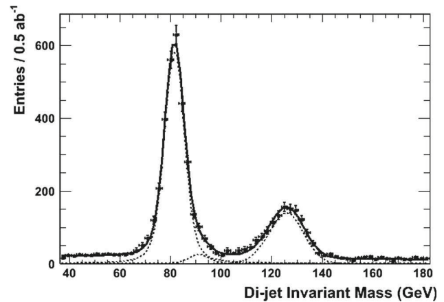
Fig. 130 Di-jet invariant mass distribution in inclusive 4-jet + missing energy SUSY events produced in \sqrt{s} = 3 \text{ TeV} e^+e^- collisions for 0.5 \text{ ab}^{-1} of fully simulated events. The result of the fit to extract the boson content is shown by the continuous line with the individual W , Z and h components represented by the dotted lines (from [1162])
