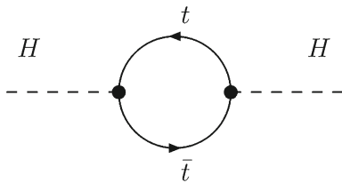
Fig. 115 Loop contribution of the top quark to the Higgs-boson mass
