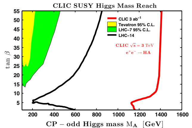
Fig. 58 Search reach in the m_A - \tan\beta plane for LHC and CLIC. The left-most coloured regions are current limits from the Tevatron with \sim 7.5\text{ fb}^{-1} of data at \sqrt{s}=1.96 TeV and from \sim 1\text{ fb}^{-1} of LHC data at \sqrt{s}=7 TeV. The black line is projection of search reach at LHC with \sqrt{s}=14 TeV and 300\text{ fb}^{-1} of luminosity [211]. The right-most red line is search reach of CLIC in the HA mode with \sqrt{s}=3 TeV. This search capacity extends well beyond the LHC [9,10]
