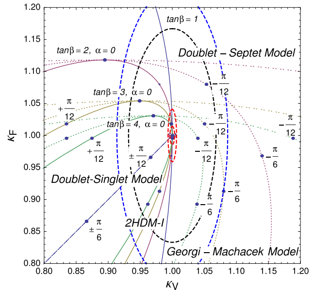
Fig. 78 The scaling factors in models with universal Yukawa couplings. The current LHC bounds and the expected LHC and ILC sensitivities are also shown at the 68.27 % CL. For details, see Ref. [340]
