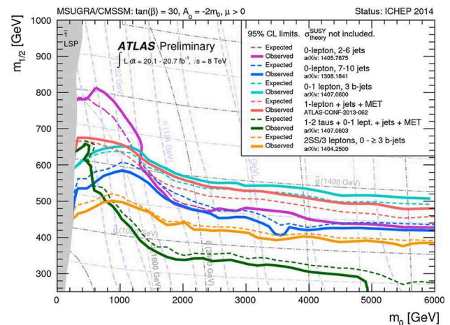
Fig. 125 95 % CL exclusion limits for MSUGRA/CMSSM models with \tan \beta = 30 , A_0 = -2m_0 and \mu > 0 presented in the [M_0, M_{1/2}] plane obtained by the ATLAS experiment with 20 \text{ fb}^{-1} of data at 8 TeV (from [1117])
