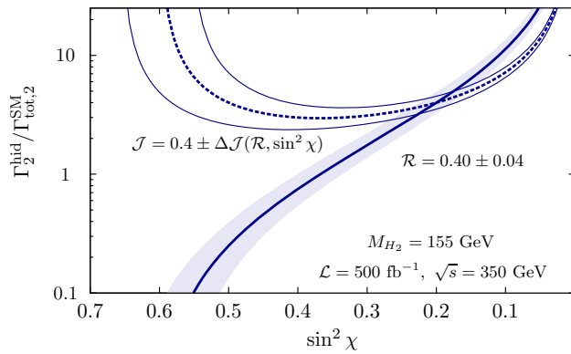
Fig. 86 Measurement of a hypothetical portal model at a 350 GeV linear collider, uncertainties are adopted from Ref. [458]. A measurement of \mathcal{R}_2 at the LHC, with only an upper 95 % confidence level bound on \mathcal{J}_2 does not constrain the region \Gamma_2^{\text{hid}}/\Gamma_{\text{tot},2}^{\text{SM}} below the \mathcal{J}_2 curve. This degeneracy is lifted with a measurement at a linear collider
