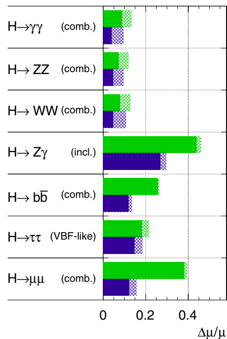
Fig. 31 Relative uncertainty on the signal strength determination expected for the ATLAS experiment [136]. Assuming a SM Higgs boson with a mass of 125 GeV and 300 \text{ fb}^{-1} and 3000 \text{ fb}^{-1} of 14 TeV data. The uncertainty pertains to the number of events passing the experimental selection, not to the particular Higgs boson process targeted. The hashed areas indicate the increase of the estimated error due to current theory systematic uncertainties
