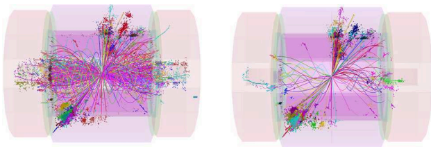
Fig. 57 Reconstructed particles in a simulated e^+e^- \rightarrow H^+H^- \rightarrow t\bar{t}b\bar{b} event at \sqrt{s}=3 TeV in the CLIC_ILD detector including the background from \gamma\gamma \rightarrow hadrons before (left) and after (right) applying tight timing cuts on the reconstructed cluster times [9,10]
