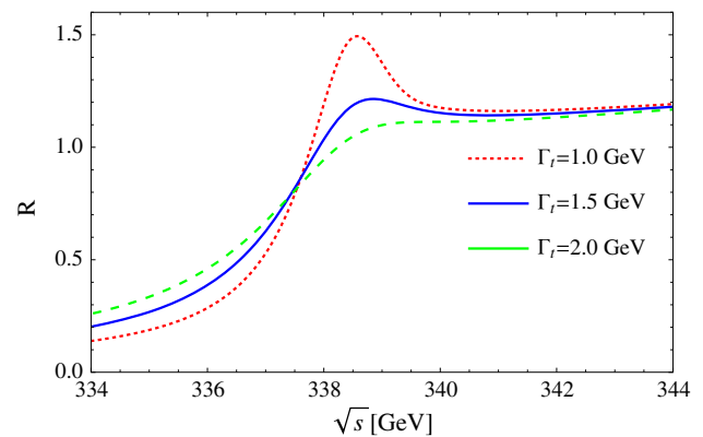
Fig. 101 The top quark production cross section R for m_t = 170 GeV and three values for top quark width. The LO formula for the cross section and \alpha_s(30\text{GeV}) = 0.142 is used
