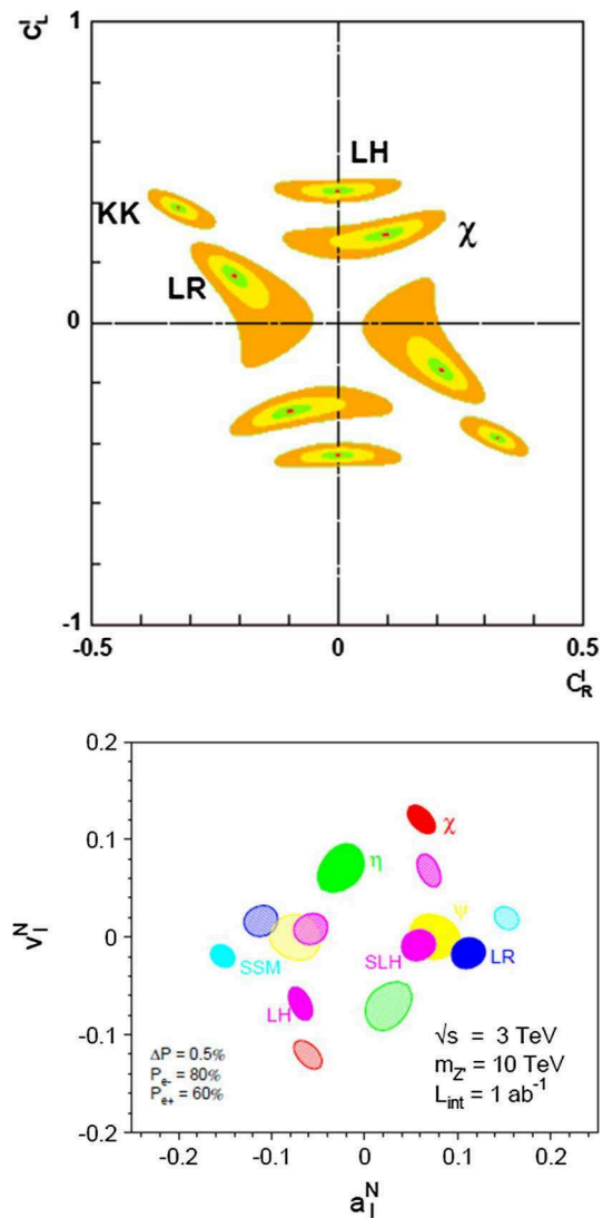
Fig. 121 Top Resolving power (95 % CL) for M_{Z'} = 1, 1.5 , and 2 \text{ TeV} and \sqrt{s} = 500 \text{ GeV} , \mathcal{L}_{\text{int}} = 1 \text{ ab}^{-1} , |P_{e^-}| = 80 \% , |P_{e^+}| = 60 \% , for leptonic couplings based on the leptonic observables \sigma , A_{\text{LR}} , A_{\text{FB}} . The couplings correspond to the E_6 \chi , LR, LH, and KK models. From Ref. [1000]. Bottom Expected resolution at CLIC with \sqrt{s} = 3 \text{ TeV} and \mathcal{L} = 1 \text{ ab}^{-1} on the “normalised” leptonic couplings of a 10 \text{ TeV} Z' in various models, assuming lepton universality. The mass of the Z' is assumed to be unknown. The couplings correspond to the E_6 \chi , \eta , and \psi , the SSM, LR, LH and SLH models. The couplings can only be determined up to a two-fold ambiguity. The degeneracy between the \psi and SLH models might be lifted by including other channels in the analysis ( \tau\tau , b\bar{b} ,...). From Refs. [9, 10, 1001]
