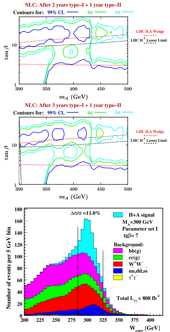
Fig. 99 Top production of A and H , with parameters corresponding to the LHC wedge, at the \gamma\gamma collider. Exclusion and discovery limits obtained for NLC collider for \sqrt{s} = 630 GeV, after 2 or 3 years of operation [642], Bottom the case M_H = M_A = 300 GeV at \chi_V^H \approx 0 in the MSSM. Distributions of the corrected invariant mass W_{corr} for selected b\bar{b} events at \tan \beta = 7 [643]
