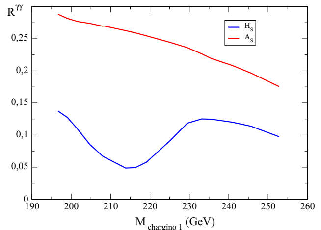
Fig. 90 The reduced coupling R^{\gamma\gamma} , as defined in Eq. (81), as function of M_{\text{chargino } 1} for M_{A_S} \sim M_{H_S} \sim 260 GeV, for a scenario explaining a 130 GeV photon line from dark matter annihilation in the galactic centre
