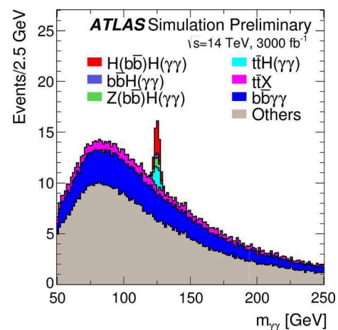
Fig. 36 Projected diphoton mass distribution for signal and background processes based on ATLAS simulations for a search for Higgs boson pair production with subsequent decays H \rightarrow b\bar{b} and H \rightarrow \gamma\gamma assuming an integrated luminosity of 3000 fb -1 [139]. The simulated distributions are scaled to match the expected event yields but do not necessarily reflect the corresponding statistical fluctuations
