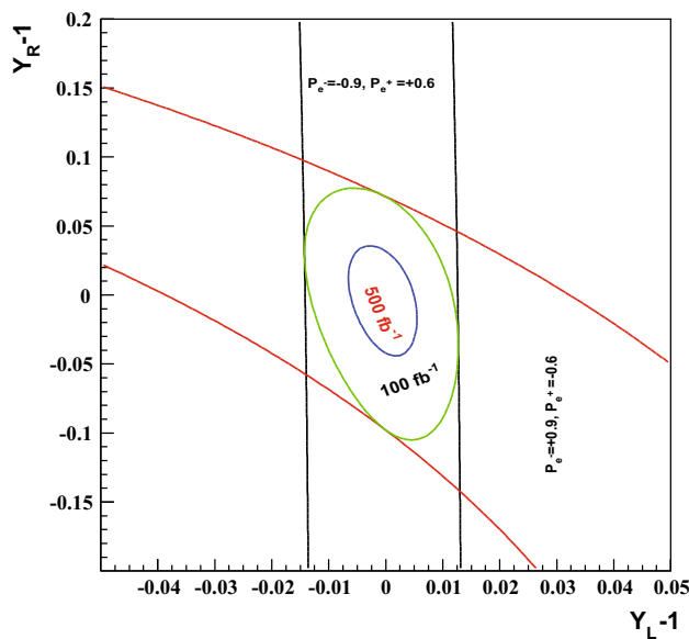
Fig. 4 Equivalence of the SUSY electroweak Yukawa couplings g_{\tilde{W}} , g_{\tilde{B}} with the SU(2) , U(1) gauge couplings g , g' . Shown are the contours of the polarised cross sections \sigma_L(e^+e^- \rightarrow \tilde{\chi}_1^0 \tilde{\chi}_2^0) and \sigma_R(e^+e^- \rightarrow \tilde{\chi}_1^0 \tilde{\chi}_2^0) in the plane of the SUSY electroweak Yukawa couplings normalised to the gauge couplings, Y_L = g_{\tilde{W}}/g , Y_R = g_{\tilde{B}}/g' [43,44] for a scenario with the electroweak spectrum similar to the reference point SPS1a
