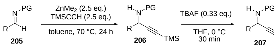
Scheme 68. Synthetic approach to N -protected propargylic amines 207 .
