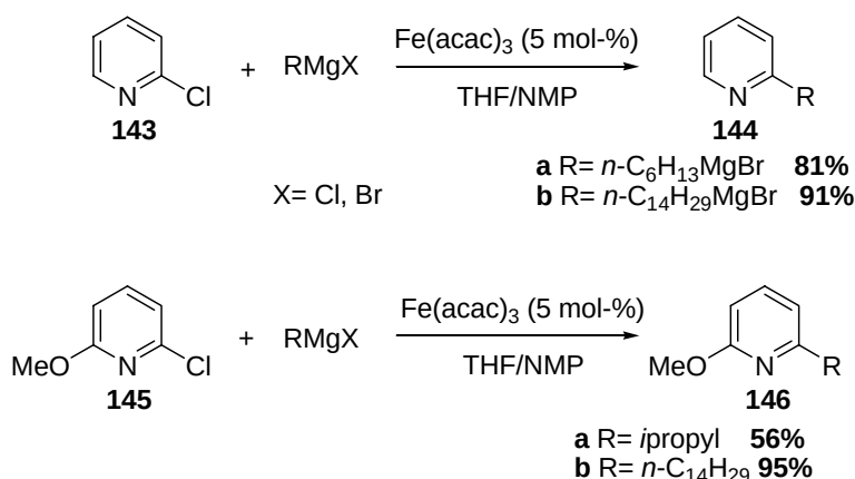
Scheme 43. Cross-coupling reactions of alkyl GRIGNARD-reagents with heteroaryl chlorides by FÜRSTNER.
