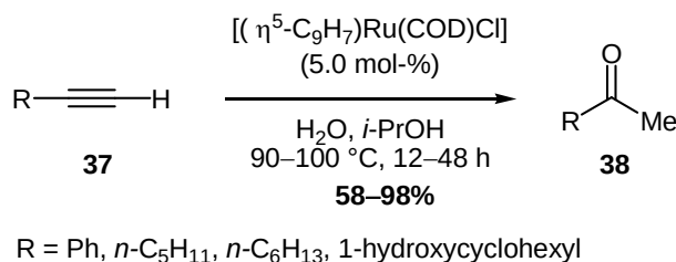
Scheme 11. Hydration of aliphatic terminal alkynes by BASSETI and GIMENO.
