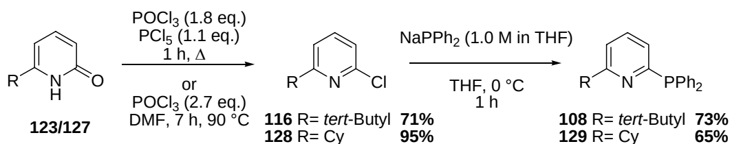
Scheme 36. Synthesis of pyridylphosphanes 108 and 129 starting from pyridine-2(1H)-ones.
