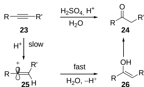
Scheme 7. Mechanism proposed for acid-catalyzed hydration.
