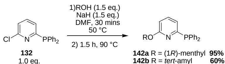
Scheme 42. Synthesis of 6-alkyloxy-substituted pyridylphosphanes 142a/b .
