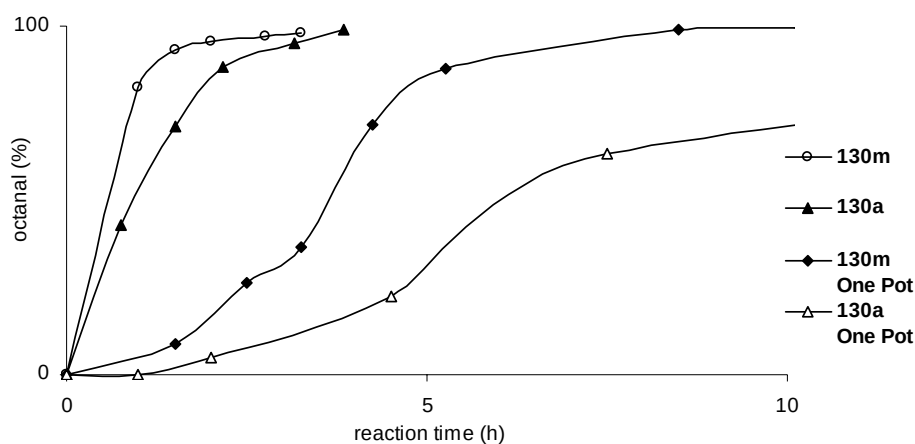
Figure 27. One-pot process of in situ catalyst formation and hydration of 1-octyne (GC data points).
