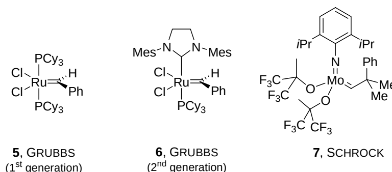
Figure 1. Catalysts for olefin metathesis.
