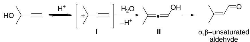
Scheme 24. The MEYER-SCHUSTER rearrangement.
