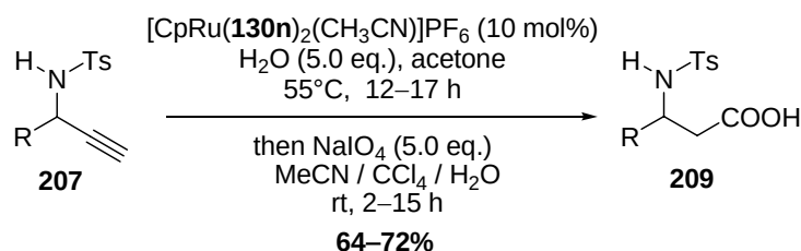
Scheme 72. Preparation of rac -β-amino acids 209 from N -tosyl amines 207 by a one-pot hydration/oxidation procedure.
