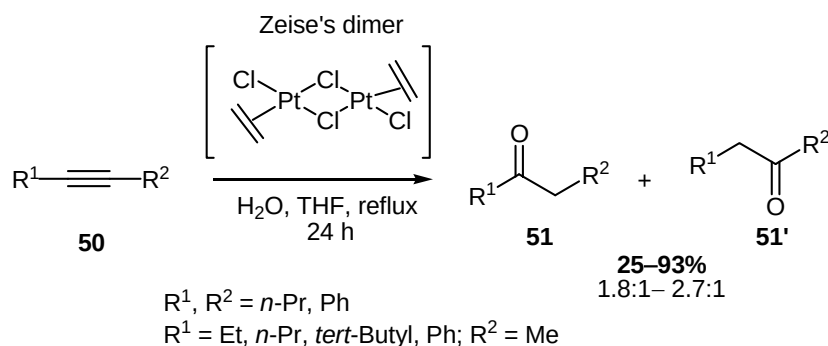
Scheme 16. ZEISE's dimer as catalyst for the hydration of alkynes by JENNING.
