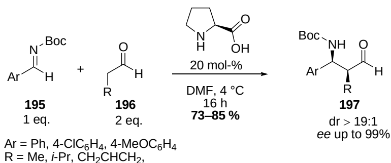
Scheme 65. Direct organocatalytic asymmetric MANNICH reactions between N -Boc protected imines 195 and aldehydes 196 by CORDOVA.
