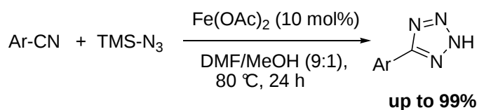
Scheme 46. Iron-catalyzed synthesis of tetrazoles.
