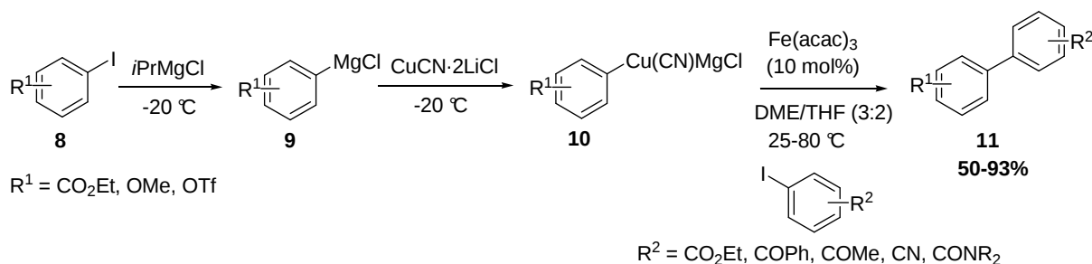
Scheme 9. Iron-catalyzed coupling reactions of organocopper reagents by Knochel.
