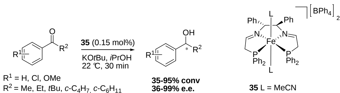
Scheme 23. Iron-catalyzed hydrogenation of ketones by Morris.
