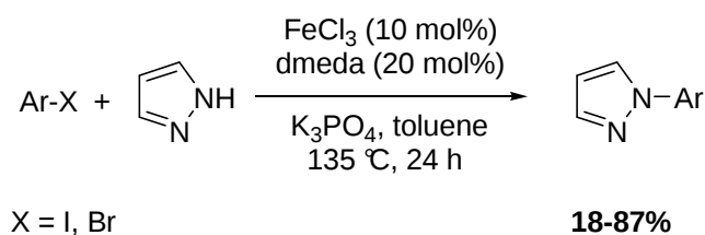
Scheme 31. Iron-catalyzed C-N arylation by Bolm
