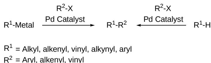
Scheme 1. Palladium-catalyzed cross-coupling.
