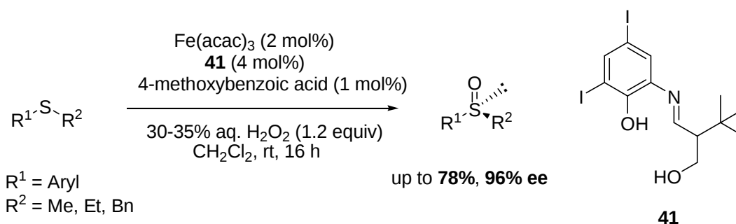
Scheme 29. Iron-catalyzed oxidation of sulfur by Bolm.
