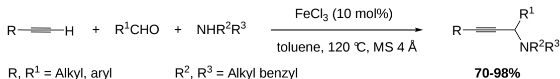
Scheme 17. Three component reaction by Wang.
