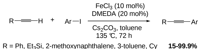
Scheme 14. Iron-catalyzed Sonogashira coupling by Bolm.
