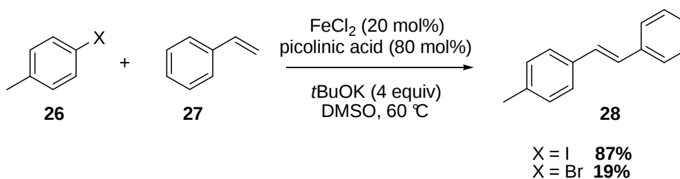
Scheme 18. Iron-catalyzed Mirozoki-Heck reaction by Vogel.
