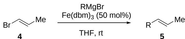
Scheme 3. Iron-catalyzed cross-coupling of Grignard reagent with vinyl halides by Kochi.
