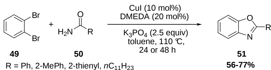
Scheme 38. Copper-catalyzed intramolecular O -arylation by Batey.
