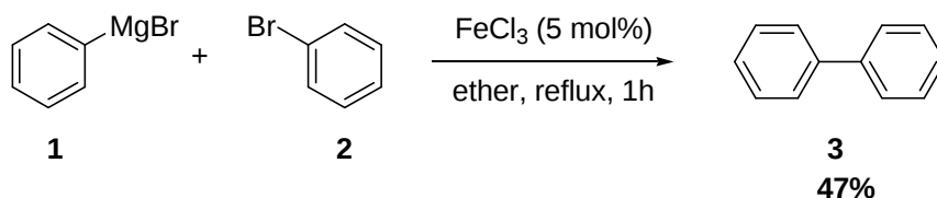
Scheme 2. Homocoupling of Grignard reagent by Kharasch.
