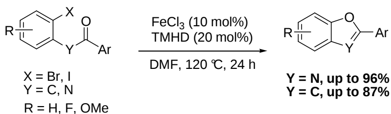
Scheme 45. Iron-catalyzed intramolecular O-arylation.
