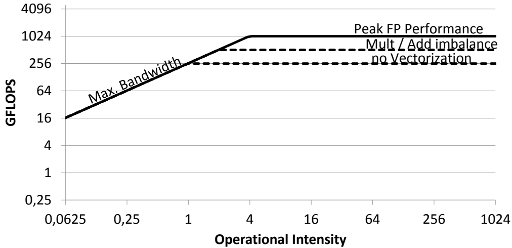
Figure 6.9: The Roofline Model applied to the BCS system.
