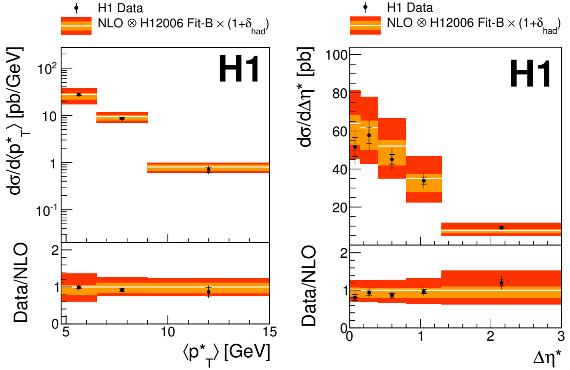
Figure 6: Diffractive dijet differential cross section as a function of \langle p_T^* \rangle and \Delta\eta^* . The inner error bars on the data points represent the statistical uncertainties, while the outer error bars include the systematic uncertainties added in quadrature. Further details are given in figure 3.
