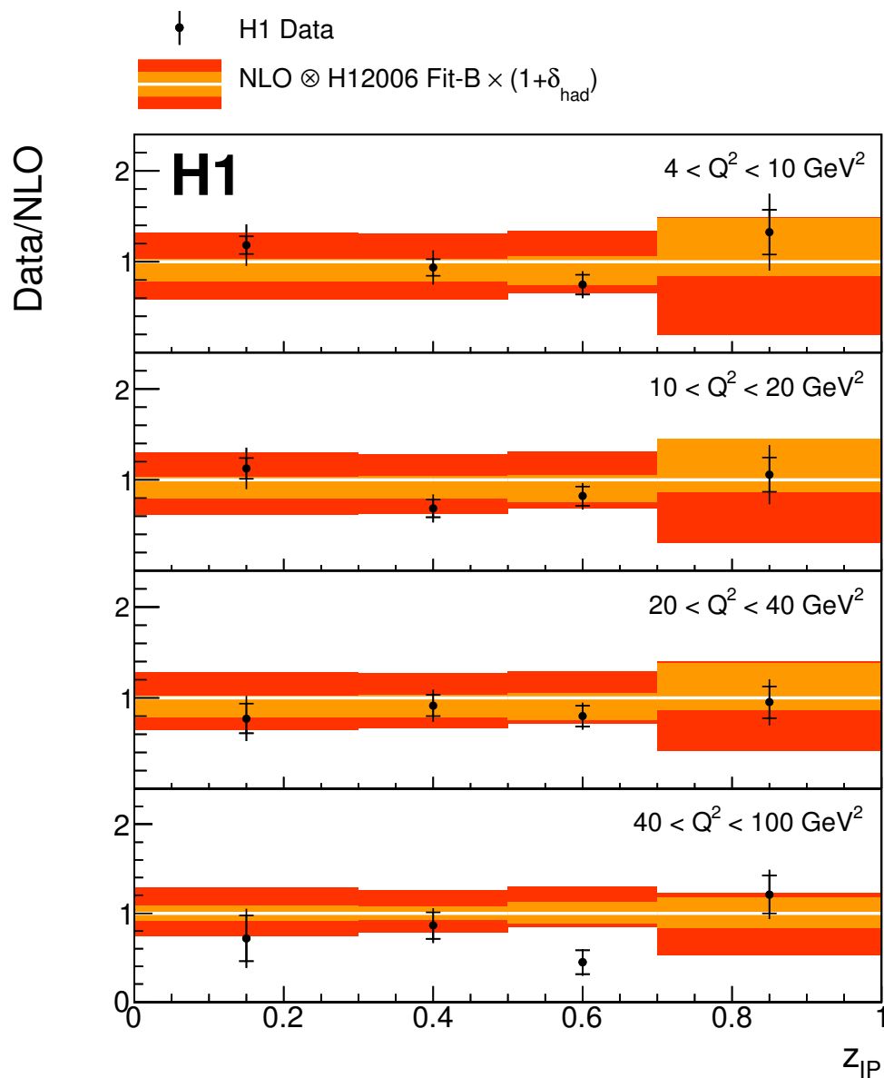
Figure 8: Ratio of the double-differential cross section to the NLO prediction as a function of z_{IP} and Q^2 . The inner error bars on the data points represent the statistical uncertainties, while the outer error bars include the systematic uncertainties added in quadrature. Further details are given in figure 3.
