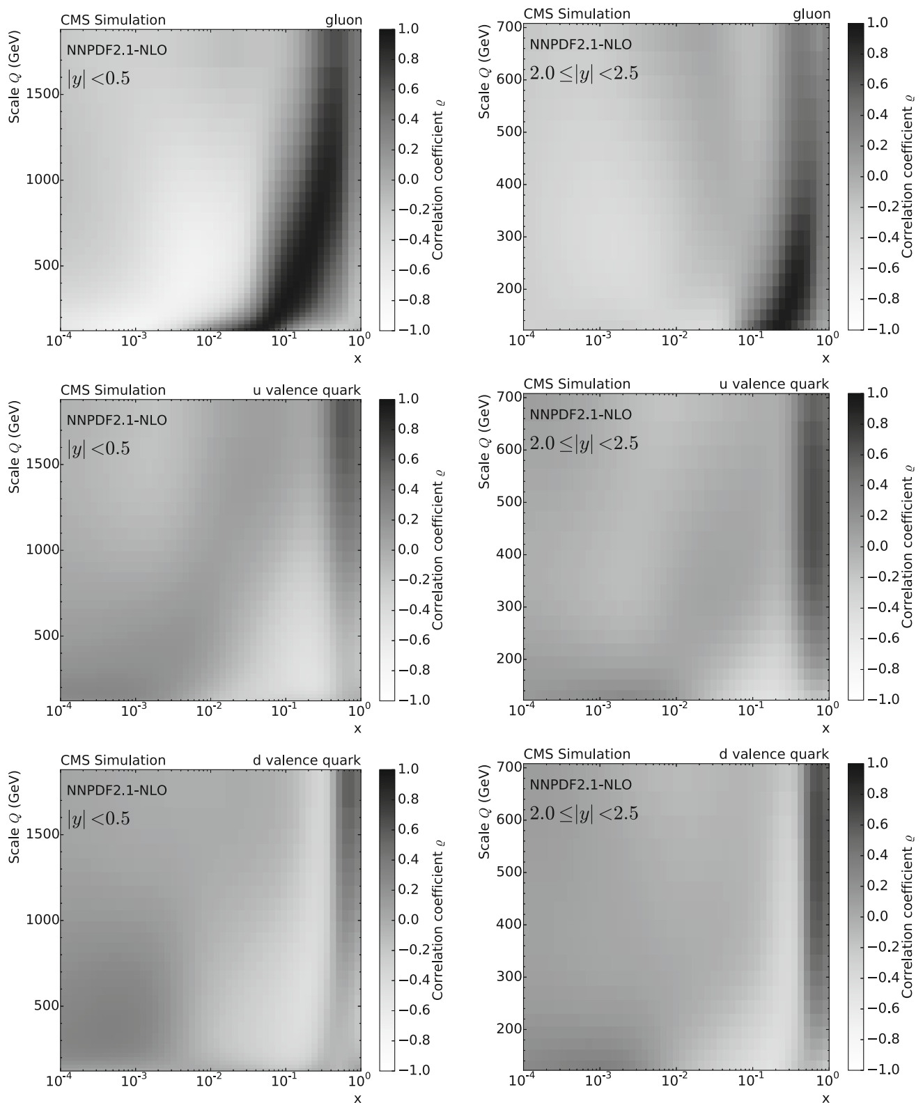
Fig. 11 The correlation coefficient between the inclusive jet cross section and the gluon (top row), the u valence quark (middle row), and the d valence quark PDFs (bottom row), as a function of the momentum
