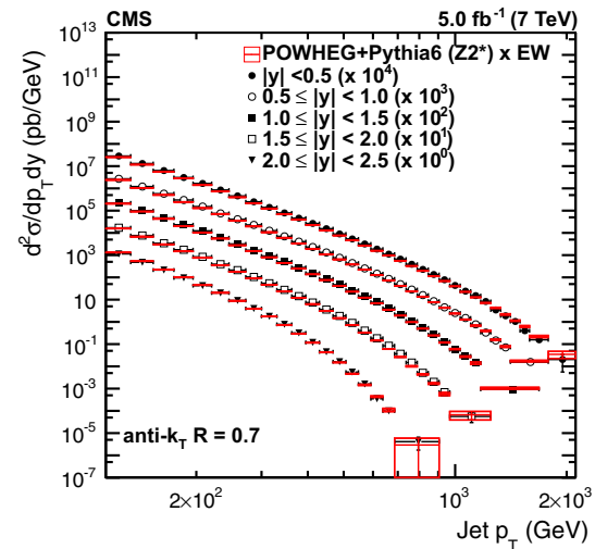
Fig. 1 Measured inclusive jet cross section from Ref. [1] compared to the prediction by POWHEG + PYTHIA6 tune Z2* at particle level complemented with electroweak corrections. The boxes indicate the statistical uncertainty of the calculation
