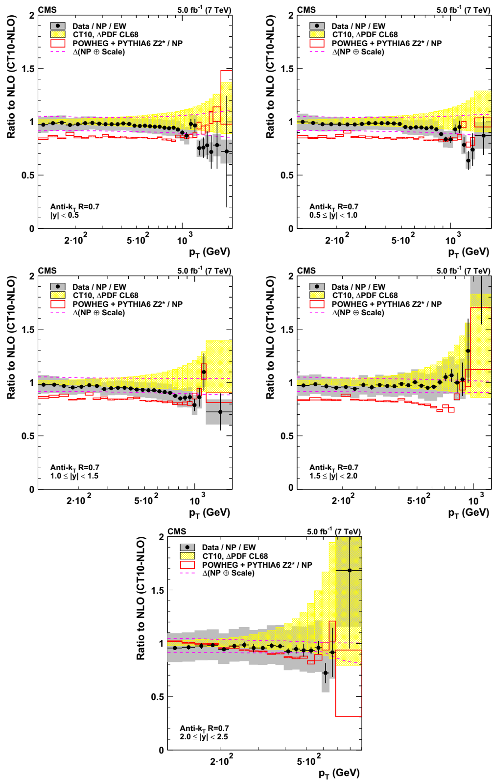
Fig. 18 Ratio of data to pQCD at NLO with the CT10-NLO PDF set multiplied by electroweak and NP corrections for the five bins in rapidity together with bands representing the CT10 PDF uncertainty (hatched), and the quadratically added scale and NP uncertainty (dashed lines). In
