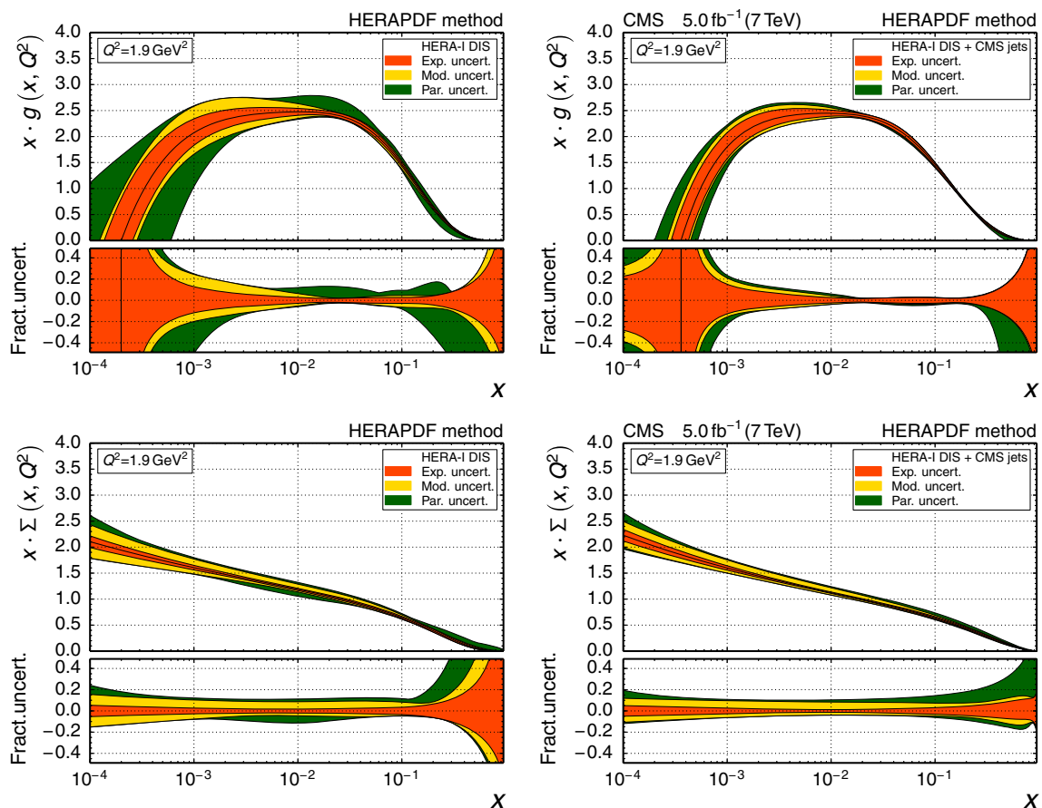
Fig. 12 The gluon (top) and sea quark (bottom) PDFs as a function of x as derived from HERA-I inclusive DIS data alone (left) and in combination with CMS inclusive jet data (right). The PDFs are shown
