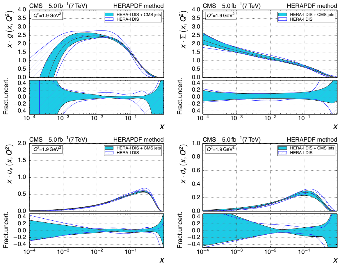
Fig. 14 The gluon (top left), sea quark (top right), u valence quark (bottom left), and d valence quark (bottom right) PDFs as a function of x as derived from HERA-I inclusive DIS data alone (dashed line) and in combination with CMS inclusive jet data (full line).
