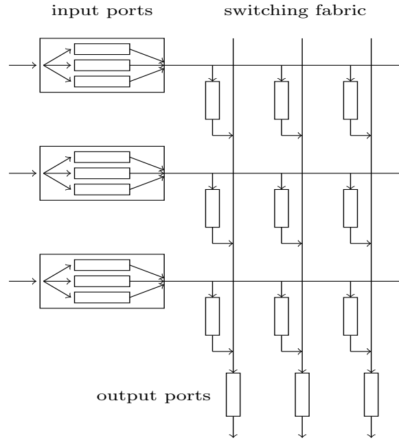
Figure 1.2: Buffered crossbar switch — An example with N = 3
