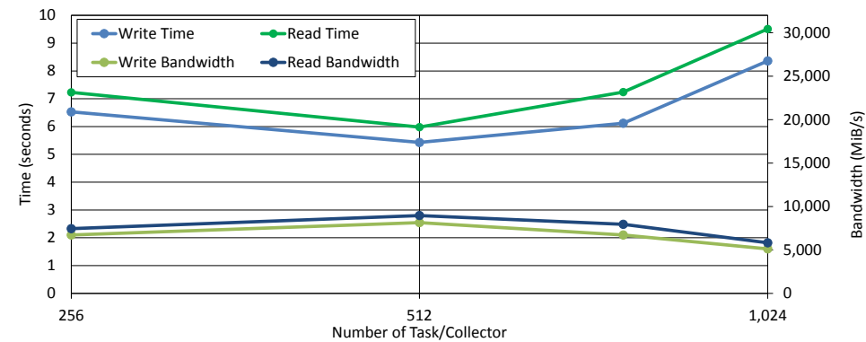
Figure 4.18: SIONlib coalescing tests with MP2C with different numbers of tasks per collector. Bandwidth and timings for writing and reading a checkpoint file are shown for one rack of JUQUEEN (64 tasks per node, 311 million particles).
