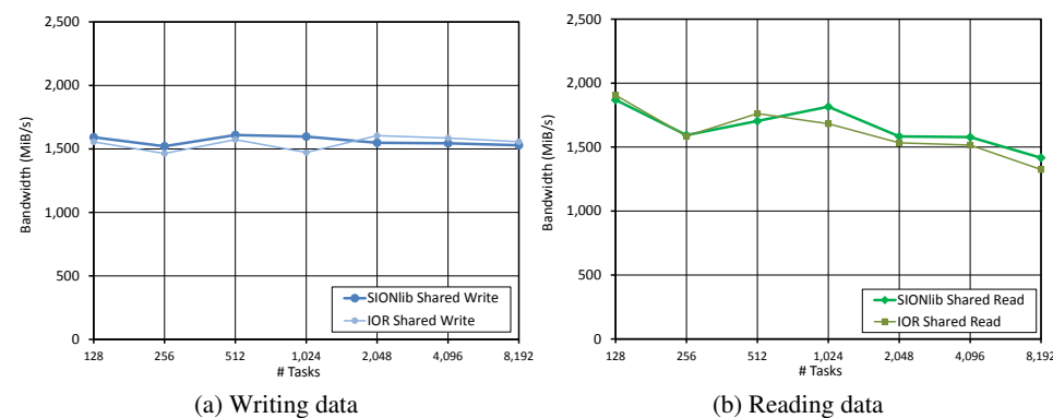
Figure 4.5: Comparison of IOR and SIONlib for baseline measurement with tasks using one I/O node on JUQUEEN (1-64 tasks per node, 2 GiB file data per node).
