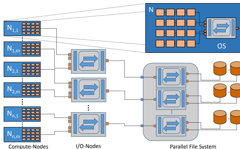
Figure 2.2: Abstract model of I/O network, compute node, and file system.
