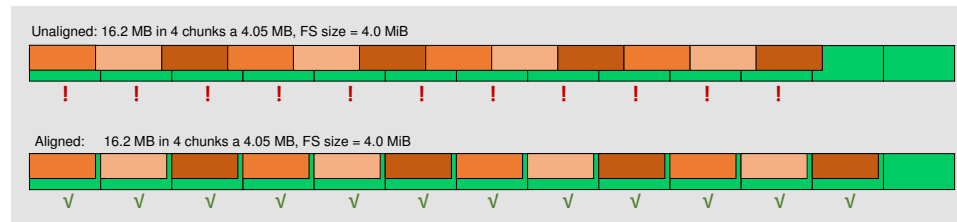
Figure 4.7: Unaligned vs. aligned shared access (three tasks). Without alignment, all chunks are consecutively positioned in an interleaving order. As a result, all file-system blocks are accessed by two different tasks concurrently. In contrast, if alignment is enabled, file-system blocks are accessed by only one task.
