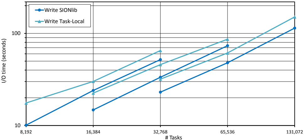
Figure 4.21: I/O timings for Scalasca’s trace-file generation using traditional task-local I/O or using a SIONlib container with one file per I/O-bridge node. The tests were repeated for different number of tasks per node on one midplane, on one rack, and on two racks of JUQUEEN (3 curves, 16-64 tasks per node).
