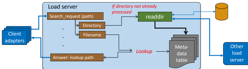
Figure 5.3: Handling of look-up requests by the Spindle server. Metadata will be processed for whole directories. If an object in a certain directory is searched, the metadata (e.g., file names) of the directory will be stored in the internal data structure.
