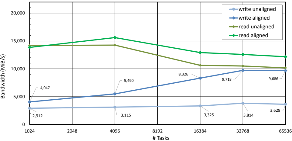
Figure 4.8: Measurement on JUQUEEN of aligned versus unaligned shared access, showing that alignment to file-system blocks increases the I/O bandwidth for writing significantly (1024 compute nodes with 1-64 tasks per node, 16.2 million bytes per task).
