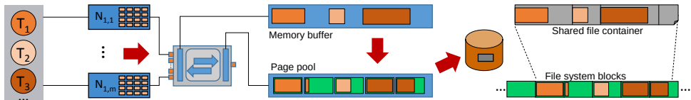
Figure 3.5: GPFS page handling for sparse shared files in a system with a hierarchical I/O infrastructure like JUQUEEN. On I/O nodes, file data is received in an incoming memory buffer and transferred by the operating system and the GPFS client to the pages in the page pool. File-system pages are transferred as full blocks to the file system, disregarding their degree of filling.
