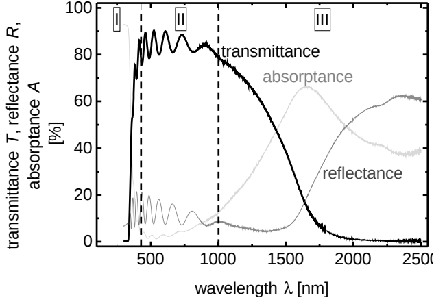
Fig. 2.2. Typical transmittance (black), reflectance (grey), and absorbance (light grey) of a common ZnO:Al layer as a function of wavelength. Three regions (I) - (III) are distinguished.
