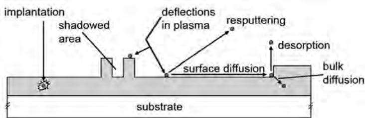
Fig. 2.5. Schematic representation of the processes that take place on the surface of the growing film during sputtering [15].
