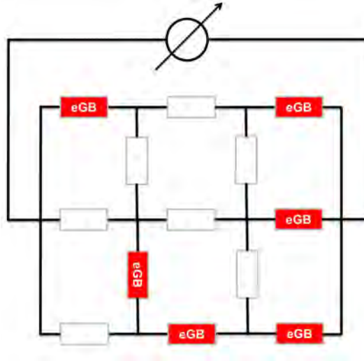
Fig. 5.22. The electrical simulation consists of a network whereby a sheet resistance value will be assigned to each data point of the curvature image. If the convex curvature lies above a threshold value r_{\text{curv}}^{\text{thr}} , a high sheet resistance R_{\text{eGB}} will be assigned to this point (red resistances). Otherwise, the sheet resistance R_{\text{flat}} of the flat reference substrates is taken.
