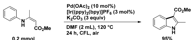
Scheme 10. Photoredox Catalysis in Palladium-Catalyzed Cyclization Reaction
