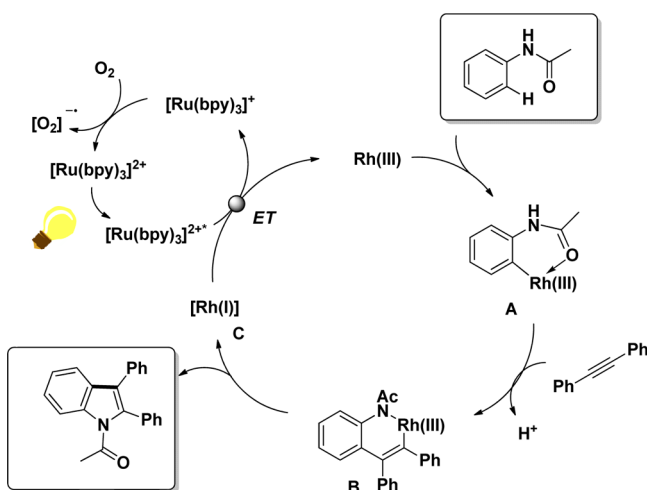
Scheme 9. Combined Rhodium- and Photoredox-Catalyzed Cyclization Reaction of Acetanilide and Diphenylacetylene
