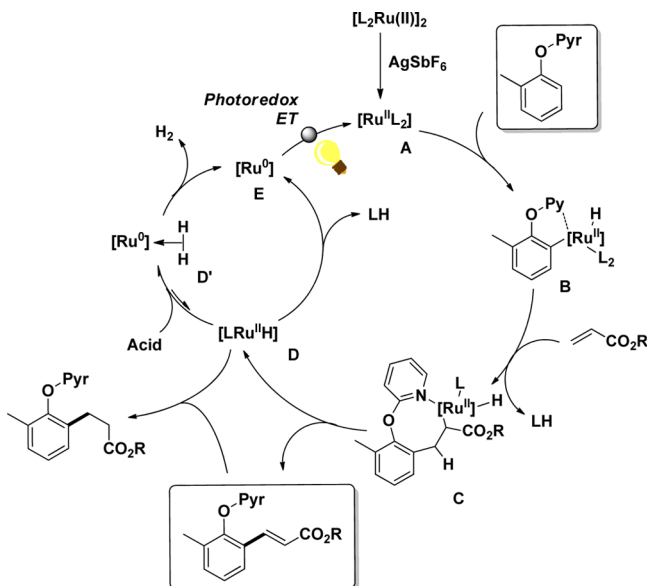
Scheme 14. Proposed Mechanism for the Ruthenium- and Photoredox-Catalyzed Olefination Reaction
