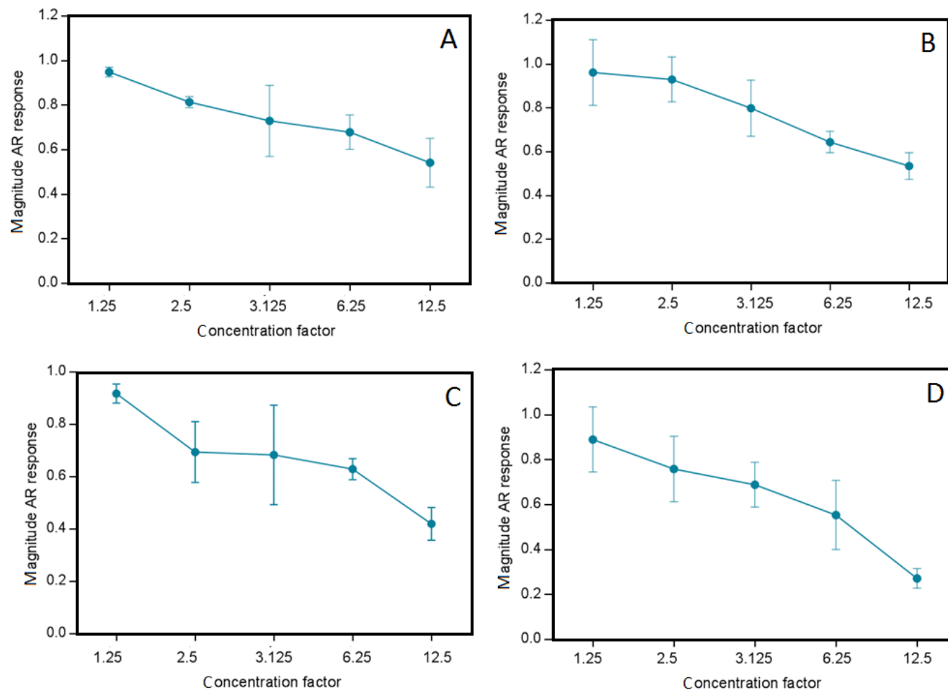
Figure 6.7: Magnitude of AR response versus different concentration factors of the active fractions obtained from the different columns, being fraction 19 for NH 2 (A), fraction 29 for PFP (B), fraction 25 from C18 (C) and fraction 37 from PYE (D). Average and standard deviation values for three replicates in one experiment.
