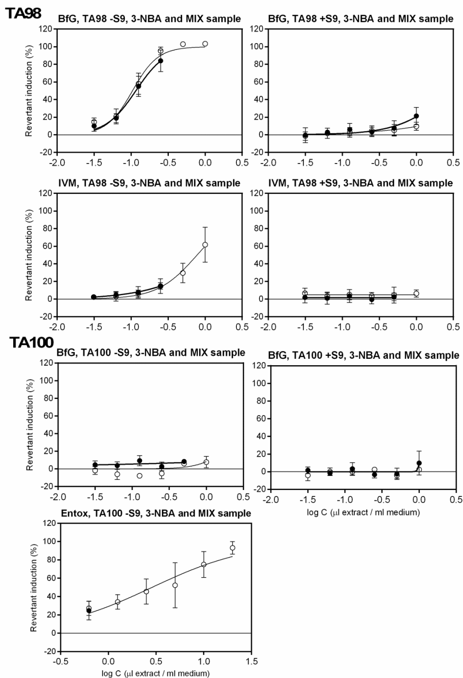
Figure S7: Ames assay revertant induction (%) in the 3-NBA ( \circ ) and mixture ( \bullet ) spikes versus log concentrations ( \mu\text{l} extract / ml medium) for BfG (pooled data for 2 experiments for each sample), IVM (pooled data for 2 experiments for each sample), and Entox (data for 1 experiment for each sample). Missing values for the mixture were excluded due to cytotoxicity. Mean values and standard deviations (error bars).
