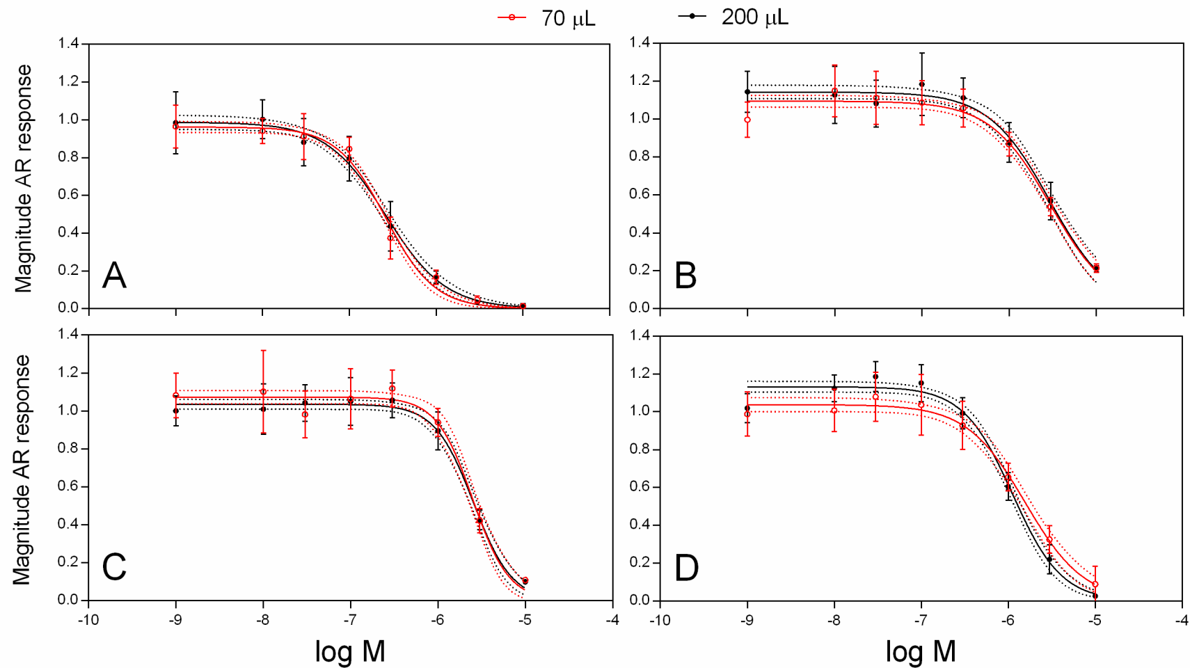
Figure 6.2: Magnitudes of AR response versus concentrations (log M) of (A) flutamide (5 tests), (B) bisphenol A (4 tests), (C) 1-hydroxypyrene (4 tests) and (D) triclosan (4 tests) following exposure volumes of 70 µL/well (red, -○-) or 200 µL/well (black, -●-) in the antagonistic assay. Mean and standard deviation values plus 95% confidence bands for 4 to 5 independent experiments in each exposure setup.
