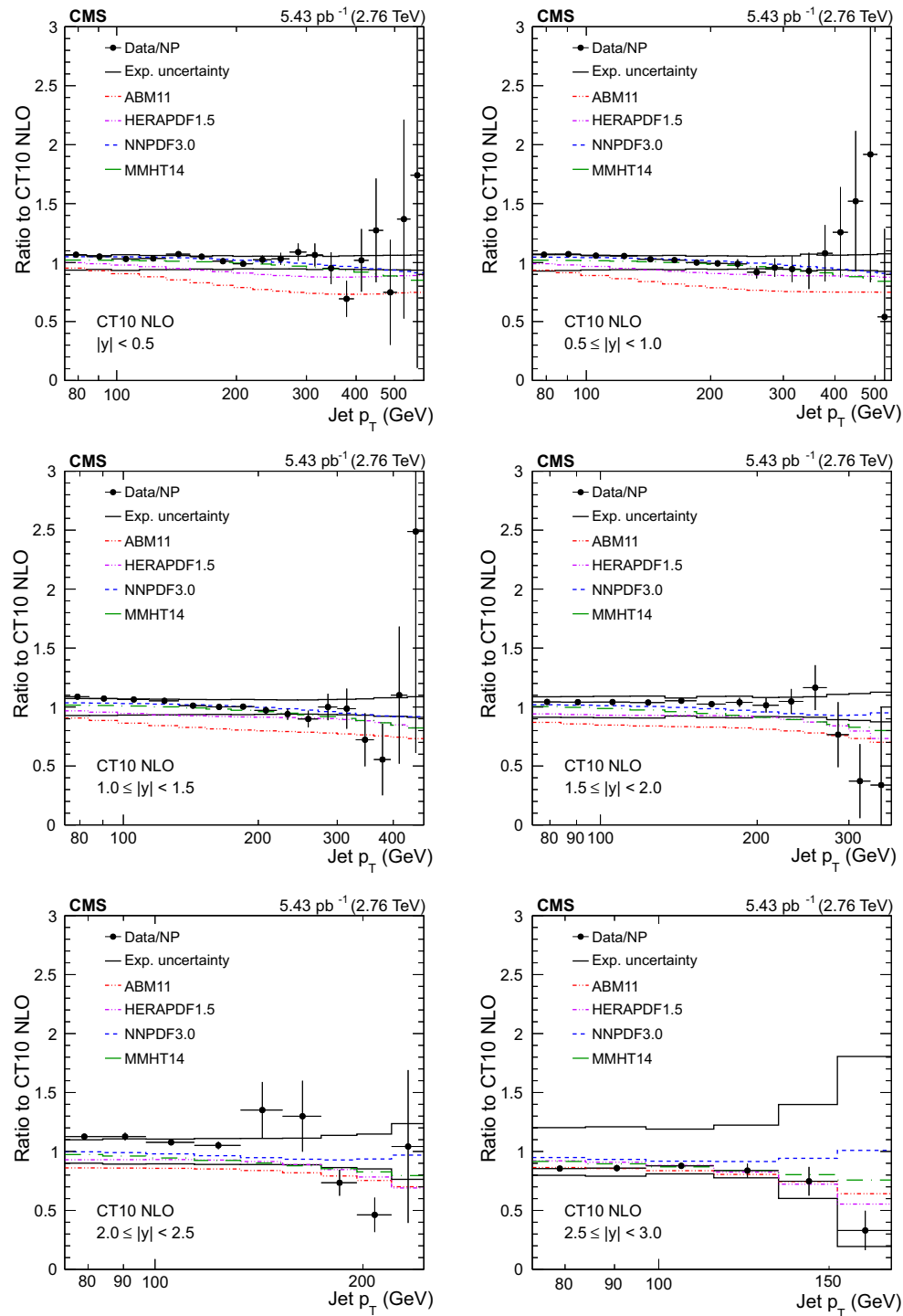
Fig. 3 The same data shown in Fig. 2 are presented showing comparisons to the NLO QCD predictions using a variety of PDFs, which are denoted by different line styles. The uncertainties corresponding to
