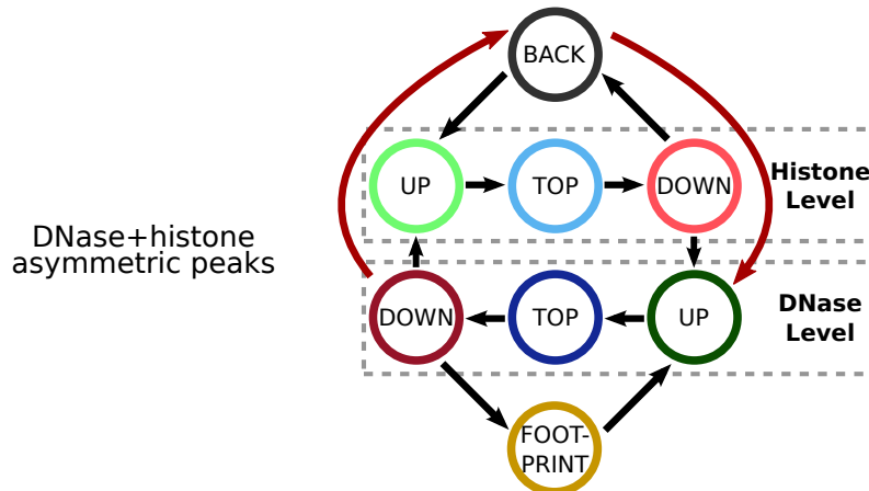
Figure 3.4: DNASE + HISTONE ASYMMETRIC PEAKS MODEL topology. Each circle represents a labeled HMM state. Each arrow represents an allowed transition between states. The red arrows represent the transitions added from the ORIGINAL DNASE + HISTONE MODEL. Self-transitions exist in all states and were omitted for simplicity. Source: Gusmao et al. (2014) (modified to fit thesis format and/or clarify key points).
