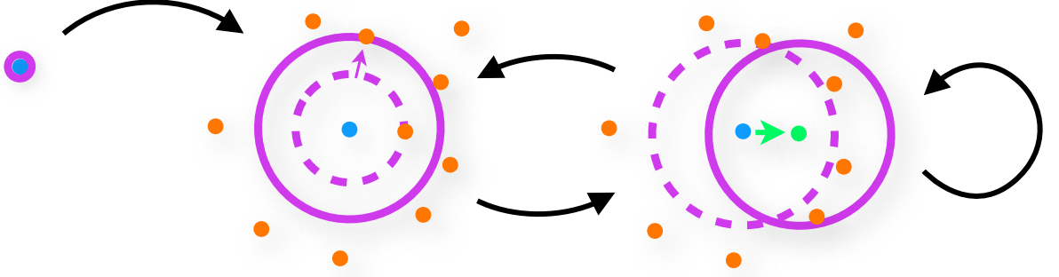
Figure 5.3: Hierarchical Medoid Shift. After being initialized with a seed (left), HMS iterates between two steps: Increasing the kernel bandwidth until a new point enters the kernel window (middle), and seeking the medoid using Medoid Shift (right).
