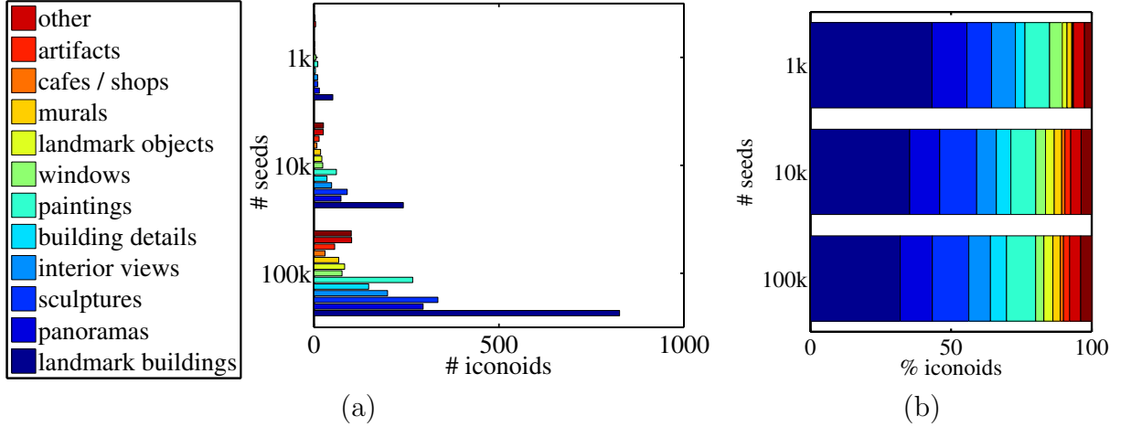
Figure 6.4: Distribution of categories for different numbers of seeds counting only clusters of size 5 or larger. (a) absolute (b) relative.
