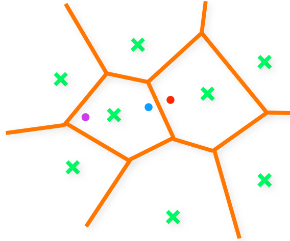
Figure 3.4: Visual words are the Voronoi cells formed by the cluster centers making up the visual vocabulary (green). The colored dots illustrate two types of quantization errors: The blue and red dots are very close in descriptor space, but are assigned different visual words, which can lead to false-negative matches. The purple and blue dots are far apart in descriptor space, but are still assigned to the same visual word which can lead to false-positive matches.
