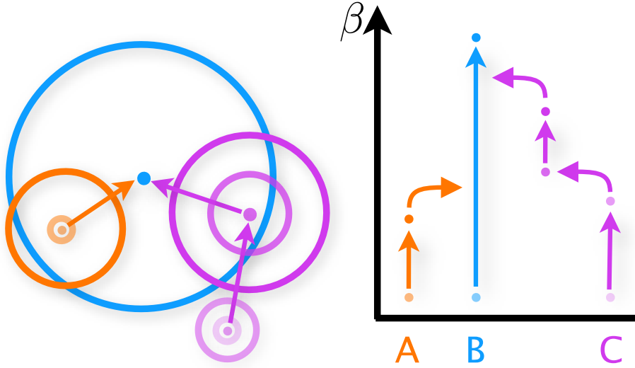
Figure 5.4: Relationship between clusters and dendrograms in Hierarchical Medoid Shift.
